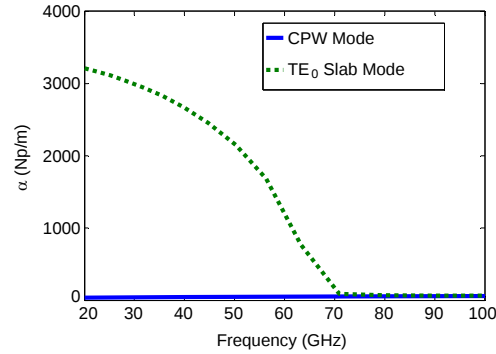
Figure 15. HFSS simulated \alpha for CPW and \text{TE}_0 modes.
