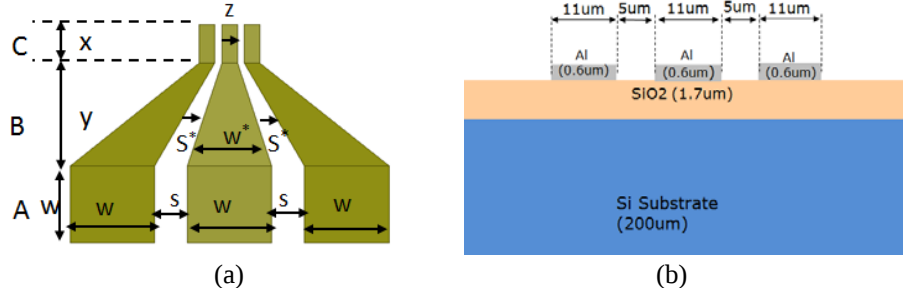
Figure 1. The FGCPW interconnect ( w = 60 \mu\text{m} , s = 23 \mu\text{m} , y = 200 \mu\text{m} , x = 25 \mu\text{m} , z = 11 , w^* varies from 60 \mu\text{m} at the bottom to 11 \mu\text{m} at the top, while s^* varies from 23 \mu\text{m} at the bottom to 5 \mu\text{m} at the top within region B, gap in C section is 5 \mu\text{m} ). (a) Top view. (b) Cross section.
