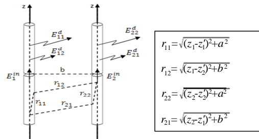
Figure 11. Array of two identical parallel linear antennas.
