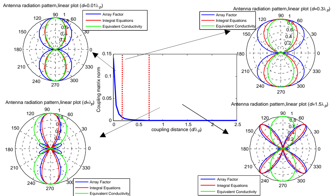
Figure 16. Array antenna radiation pattern obtained using effective conductivity approach, the proposed coupled integral equations approach and array factor method. Results obtained for different coupling distances.
