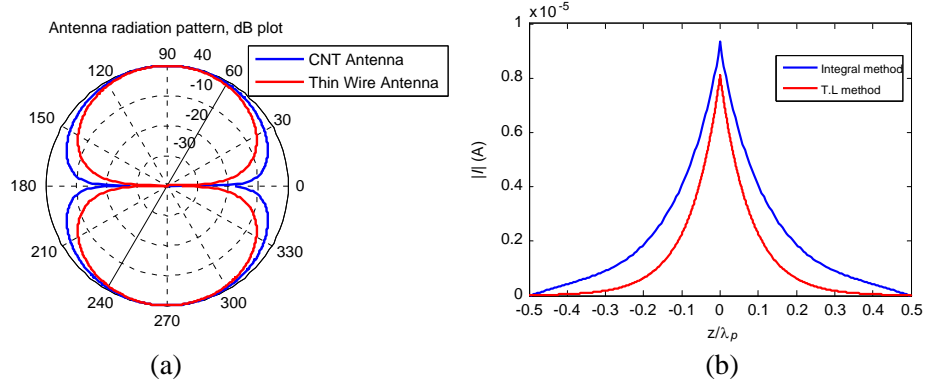
Figure 5. (a) Antenna radiation pattern obtained on a CNT dipole antenna and perfectly conducting thin wire antenna of length L = 20 \mu\text{m} and L = 2 \text{ mm} respectively, for operating frequency f = 150 \text{ GHz} . (b) Current distribution on a CNT dipole antenna using MoM method and transmission line method for an antenna length L = 300 \mu\text{m} and operating frequency f = 10 \text{ GHz} .
