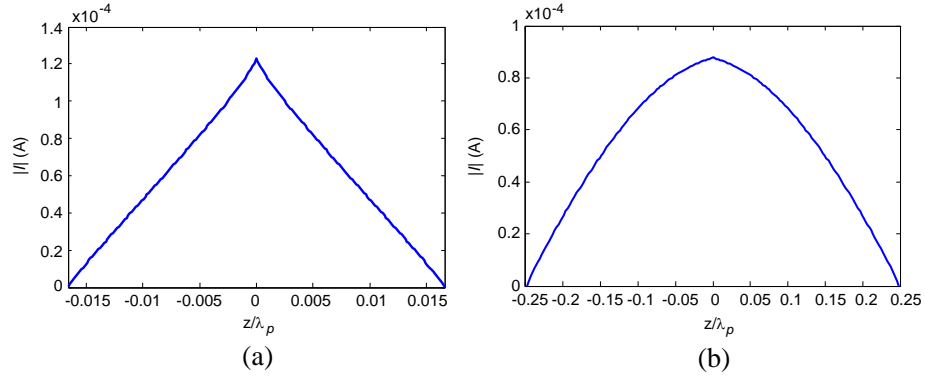
Figure 6. Current distribution obtained on a CNT dipole antenna of length L = 20 \mu\text{m} and radius a = 2.71 \text{ nm} . (a) Operating frequency f = 10 \text{ GHz} . (b) Operating frequency f = 150 \text{ GHz} .
