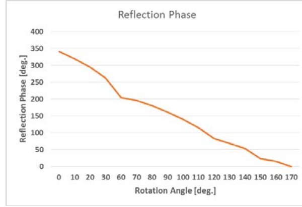
Figure 5. Reflection Phase of Pierrot cell against rotation about z -axis.
