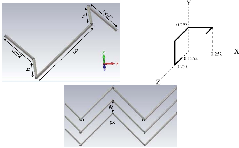
Figure 9. Geometry of a Morin cell and simulation in CST software. The figure depicts an LHCPSS (assuming the wave is travelling in the positive z -direction).
