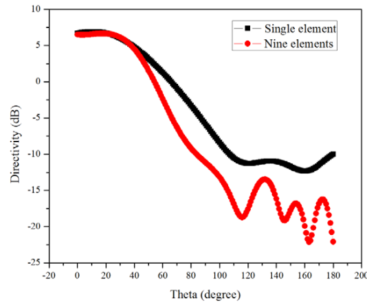
Figure 6. Radiation pattern (directivity plot) at frequency = 10.35 GHz.
