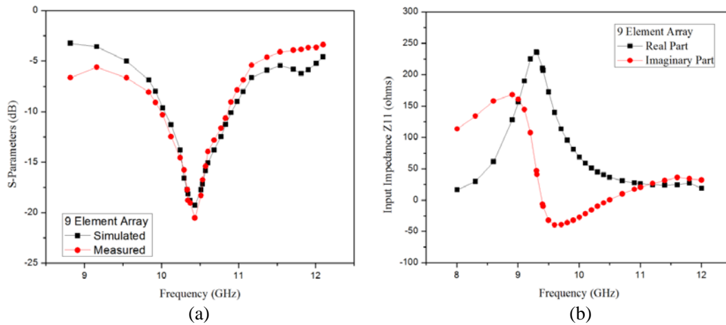
Figure 5. (a) Variation of S -parameters with frequency (for 9 element array). (b) Variation of input impedance with frequency (for 9 element array).
