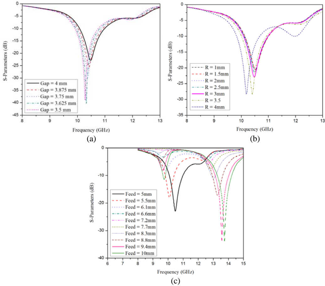
Figure 4. Variation of S -parameters with frequency for: (a) gap variation, (b) radius variation, (c) feed location variation.
