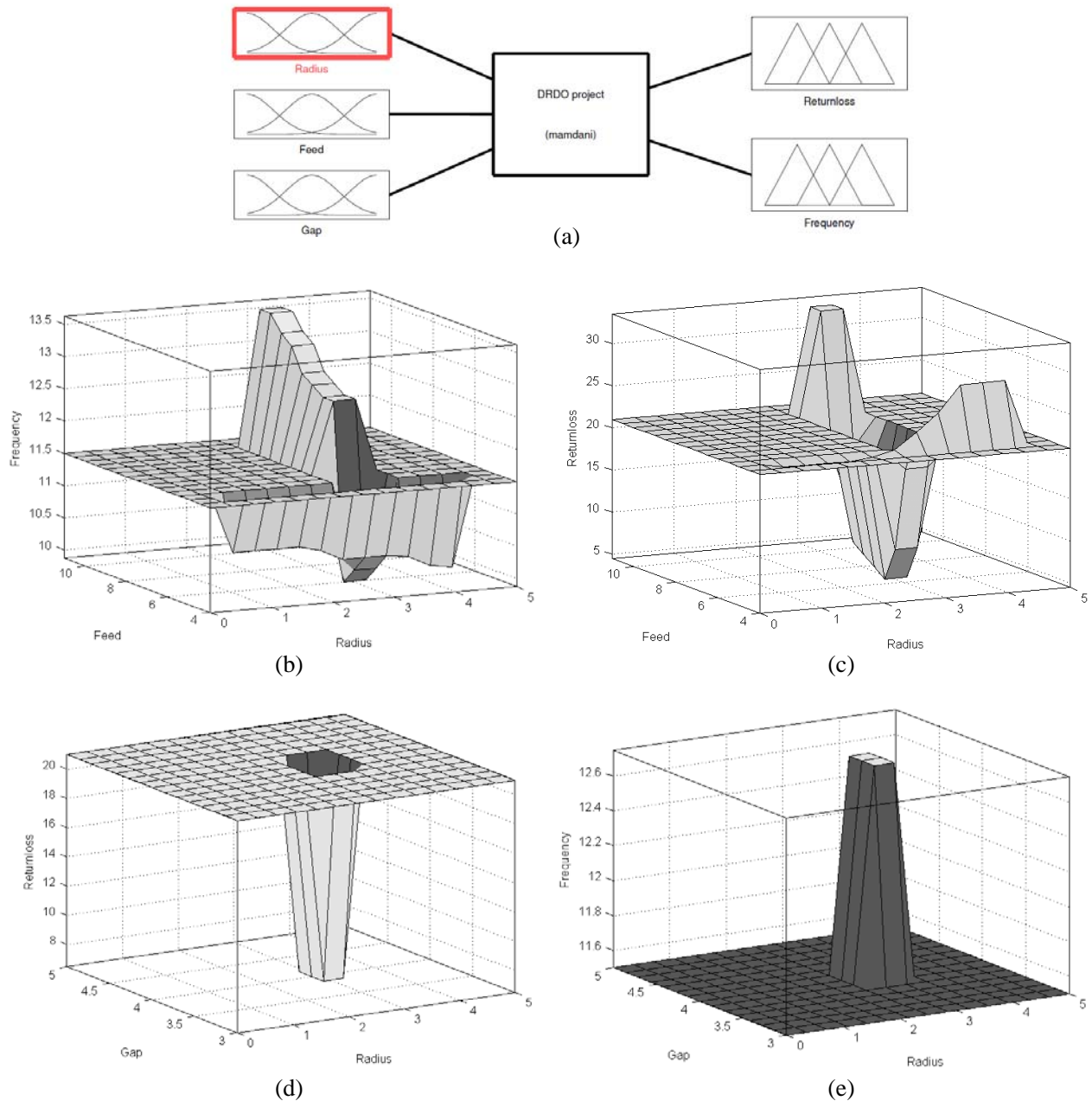
Figure 3. Surface plots for the variation of feed location, gap and radius with frequency and return loss. (a) Mamdani FIS model. (b) Frequency, feed, radius. (c) Return loss, feed, radius. (d) Return loss, gap, radius. (e) Frequency, gap, radius.
