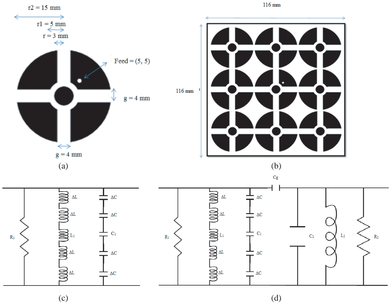
Figure 1. Geometry of proposed microstrip antenna. (a) Single element. (b) Nine element array. (c) Equivalent circuit of ring with notches. (d) Equivalent circuit of whole single element.
