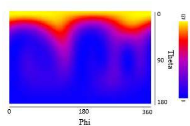
Figure 6. 2D far-field distribution at 5.5 GHz.
