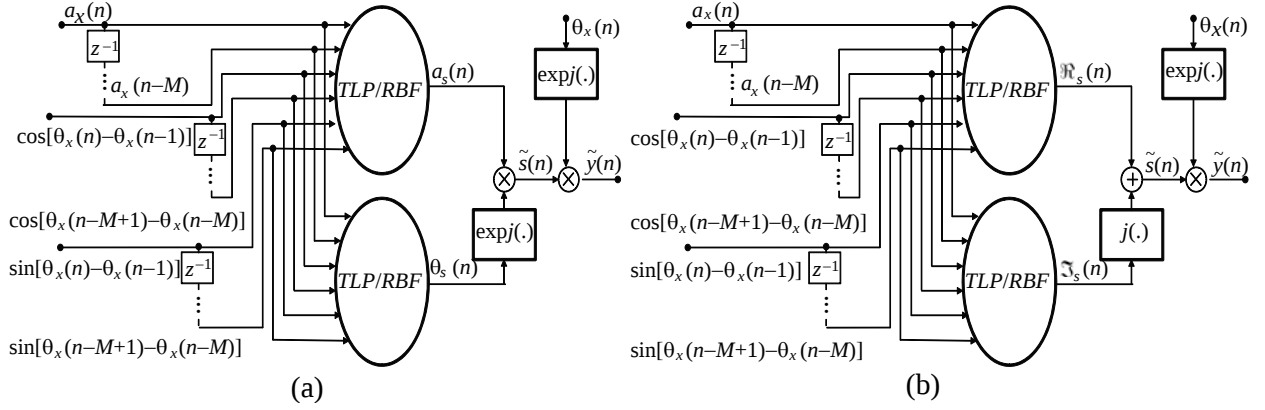
Figure 4. Block diagram of ANN-based PA behavioral models: (a) previous [13] and (b) proposed.
