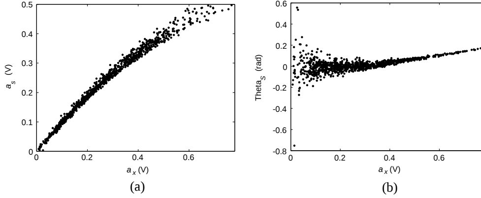
Figure 2. Nonlinear transfer characteristics measured on a GaN HEMT class AB PA excited by a WCDMA signal: (a) amplitude of \tilde{s} as a function of the instantaneous input amplitude, (b) polar angle of \tilde{s} as a function of the instantaneous input amplitude.
