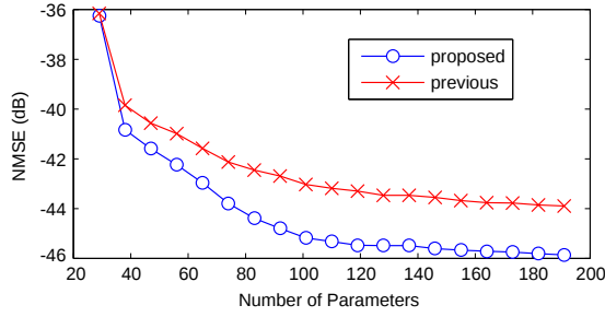
Figure 5. NMSE results as a function of the number of network parameters. The GaN HEMT class AB PA is modeled by TLPs having M = 2 and a variable number of neurons in the hidden layer.
