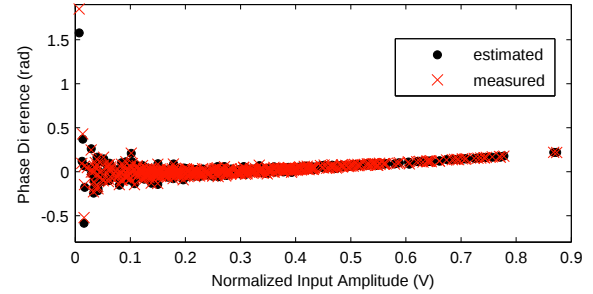
Figure 8. Measured and estimated AM-PM conversions. The GaN HEMT class AB PA is modeled by the proposed TLP having M = 2 and 110 network parameters.
