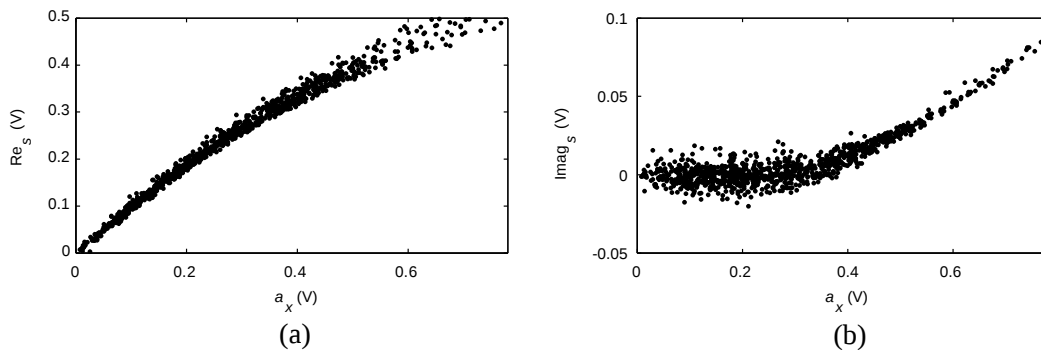
Figure 3. Nonlinear transfer characteristics measured on a GaN HEMT class AB PA excited by a WCDMA signal: (a) real part of \tilde{s} as a function of the instantaneous input amplitude, (b) imaginary part of \tilde{s} as a function of the instantaneous input amplitude.
