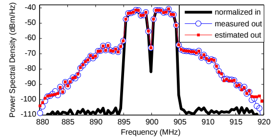
Figure 6. Power spectral densities of the measured and estimated PA output signals. The GaN HEMT class AB PA is modeled by the proposed TLP having M = 2 and 110 network parameters.
