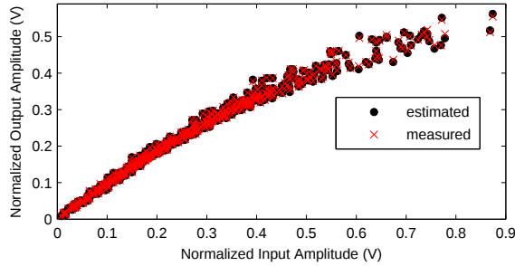
Figure 7. Measured and estimated normalized AM-AM conversions. The GaN HEMT class AB PA is modeled by the proposed TLP having M = 2 and 110 network parameters.
