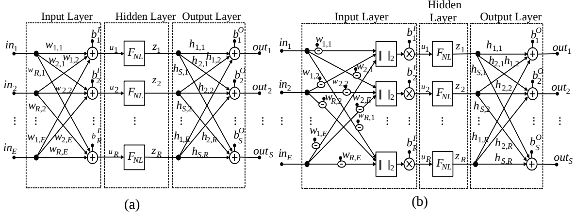
Figure 1. Block diagram of neural networks: (a) three-layer perceptron and (b) radial basis function.
