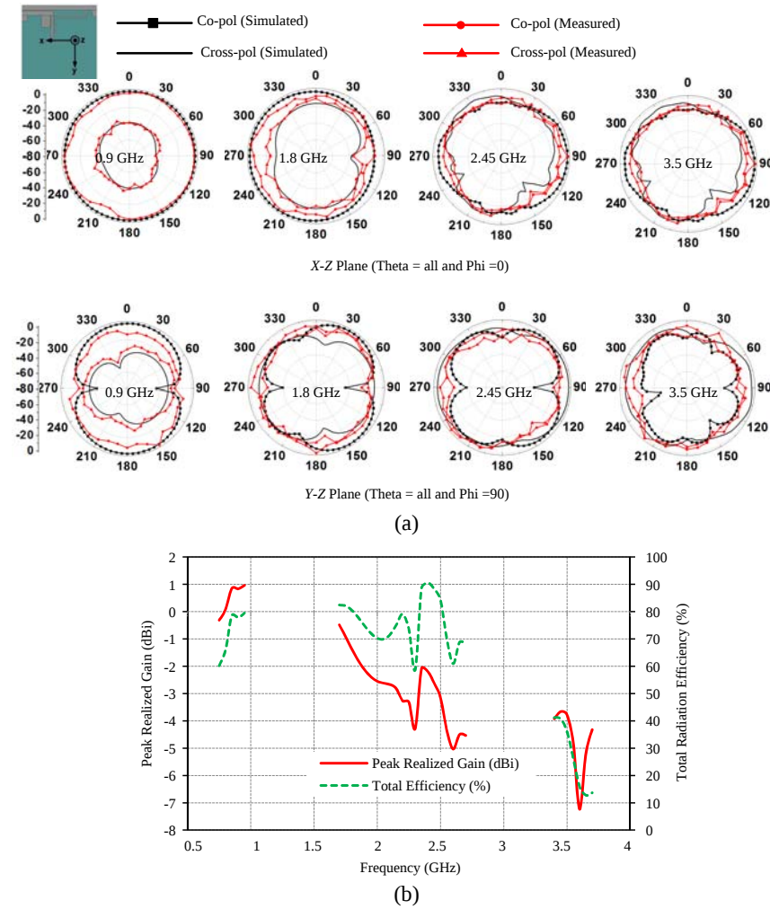
Figure 6. (a) Simulated and measured radiation patterns. (b) Variation of peak realized gain and total efficiency with frequency.
