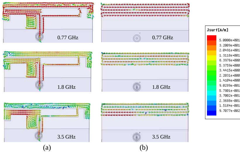
Figure 3. Vector surface current distribution at different frequencies. (a) Front view. (b) Rear view.
