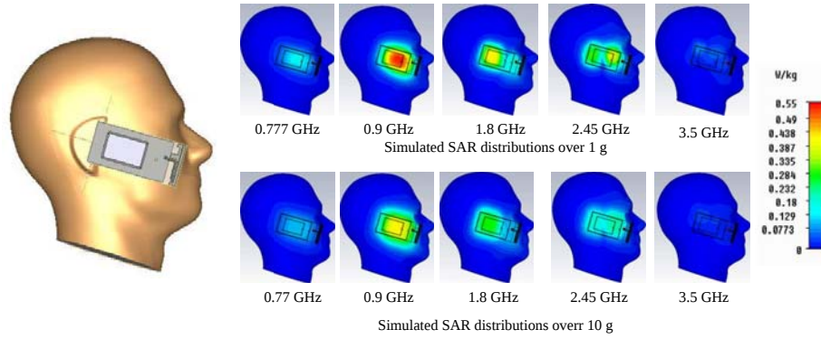
Figure 8. SAR simulation setup and SAR distribution on SAM head phantom.
