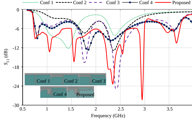
Figure 2. The variation of the reflection coefficient with frequency for different configurations during evolution.
