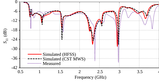
Figure 4. Simulated and measured reflection coefficient.
