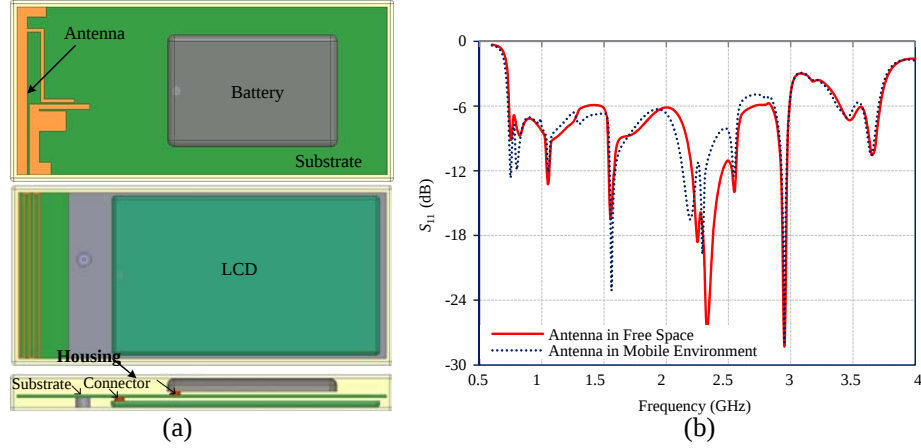
Figure 7. (a) Antenna in mobile environment. (b) Effect of mobile environment on S -parameters.
