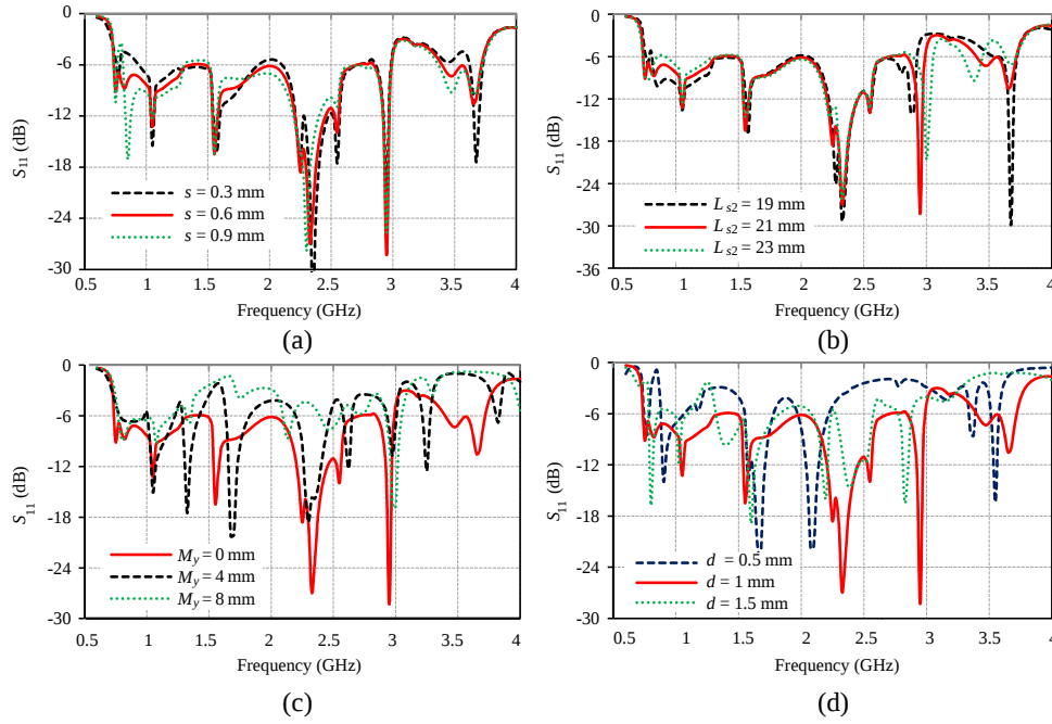
Figure 5. Variation of the reflection coefficient with shape parameters (a) s , (b) L_{s2} , (c) M_y , and (d) d .
