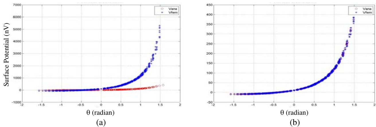
Figure 8. Analytical ( ^{\circ} Vana) and numerical ( ^{*} Vfem) potential distribution for a radial dipole near the interface. (a) is the result with all monopoles, (b) those for the monopoles located only in the brain layer.
