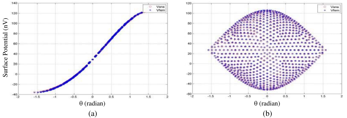
Figure 6. Analytical (°Vana) and numerical solution (*Vfem) on all surface's nodes versus the theta angle (radian), (b) shows the result for a centered radial dipole, (a) those for a centered tangential dipole.
