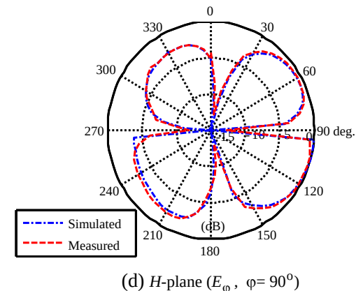
Figure 16. Radiation patterns of E and H plane for Antenna3, (a), (b) at 6.806 GHz and (c), (d) at 9.13 GHz.
