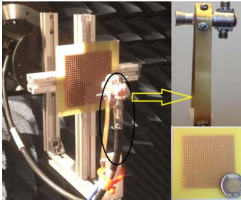
Figure 15. Fabricated bow-tie CP RA antenna.
