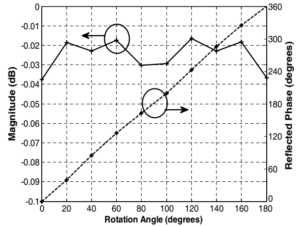
Figure 6. Reflected wave amplitude vs bowtie rotation at 30 GHz.
