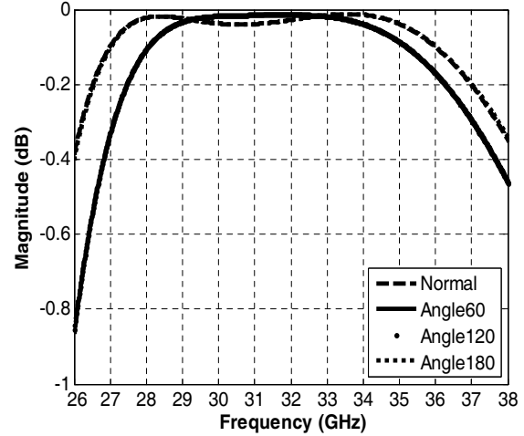
Figure 8. Co-polar wave maximization in operating band.
