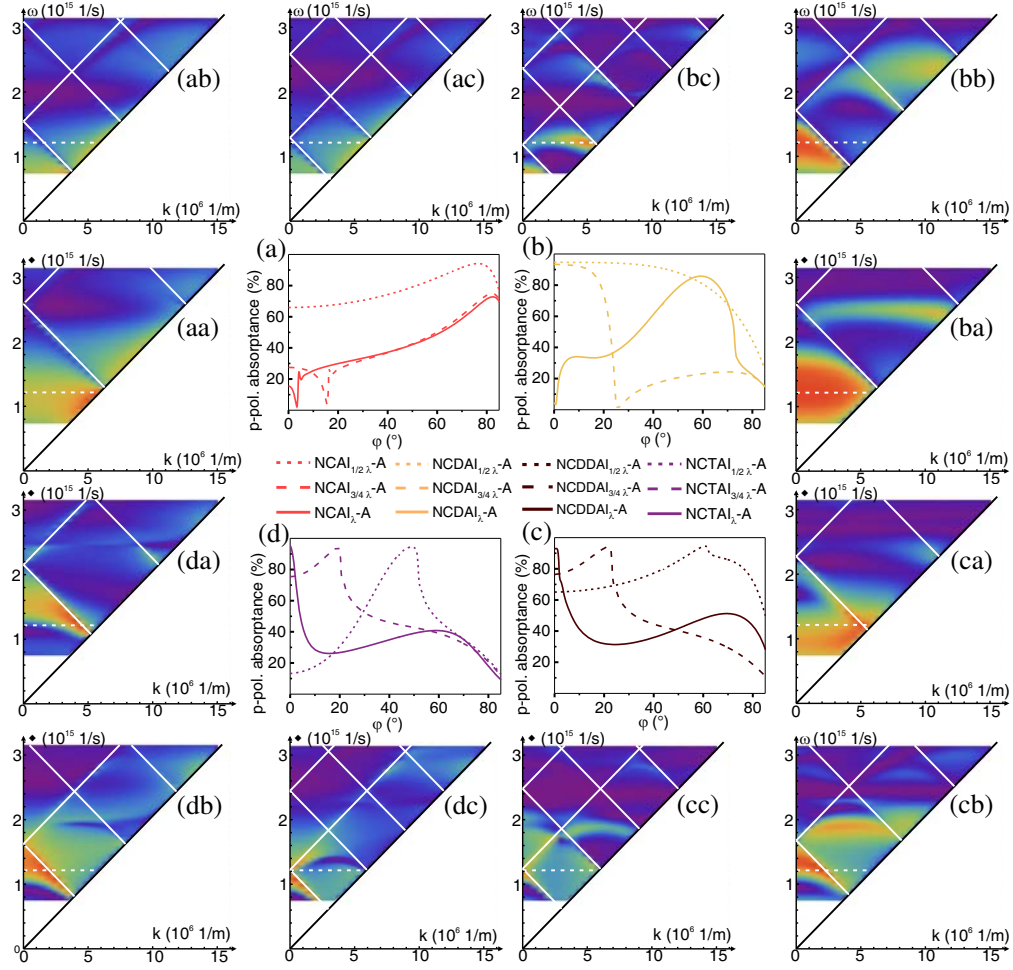
Figure 3. Polar-angle-dependent p-polarized absorptances at 1550 nm of (a) NCAI-, (b) NCDAl-, (c) NCDDAl- and (d) NCTAl-A-SNSPD at \gamma = 90^\circ azimuthal orientation (in S-orientation). Dispersion diagrams of (aa) \text{NCAI}_{1/2\lambda}^{-} , (ab) \text{NCAI}_{3/4\lambda}^{-} , (ac) \text{NCAI}_{\lambda}^{-} , (ba) \text{NCDAl}_{1/2\lambda}^{-} , (bb) \text{NCDAl}_{3/4\lambda}^{-} , (bc) \text{NCDAl}_{\lambda}^{-} , (ca) \text{NCDDAl}_{1/2\lambda}^{-} , (cb) \text{NCDDAl}_{3/4\lambda}^{-} , (cc) \text{NCDDAl}_{\lambda}^{-} , (da) \text{NCTAl}_{1/2\lambda}^{-} , (db) \text{NCTAl}_{3/4\lambda}^{-} and (dc) \text{NCTAl}_{\lambda}^{-} -A-SNSPD in S-orientation.
