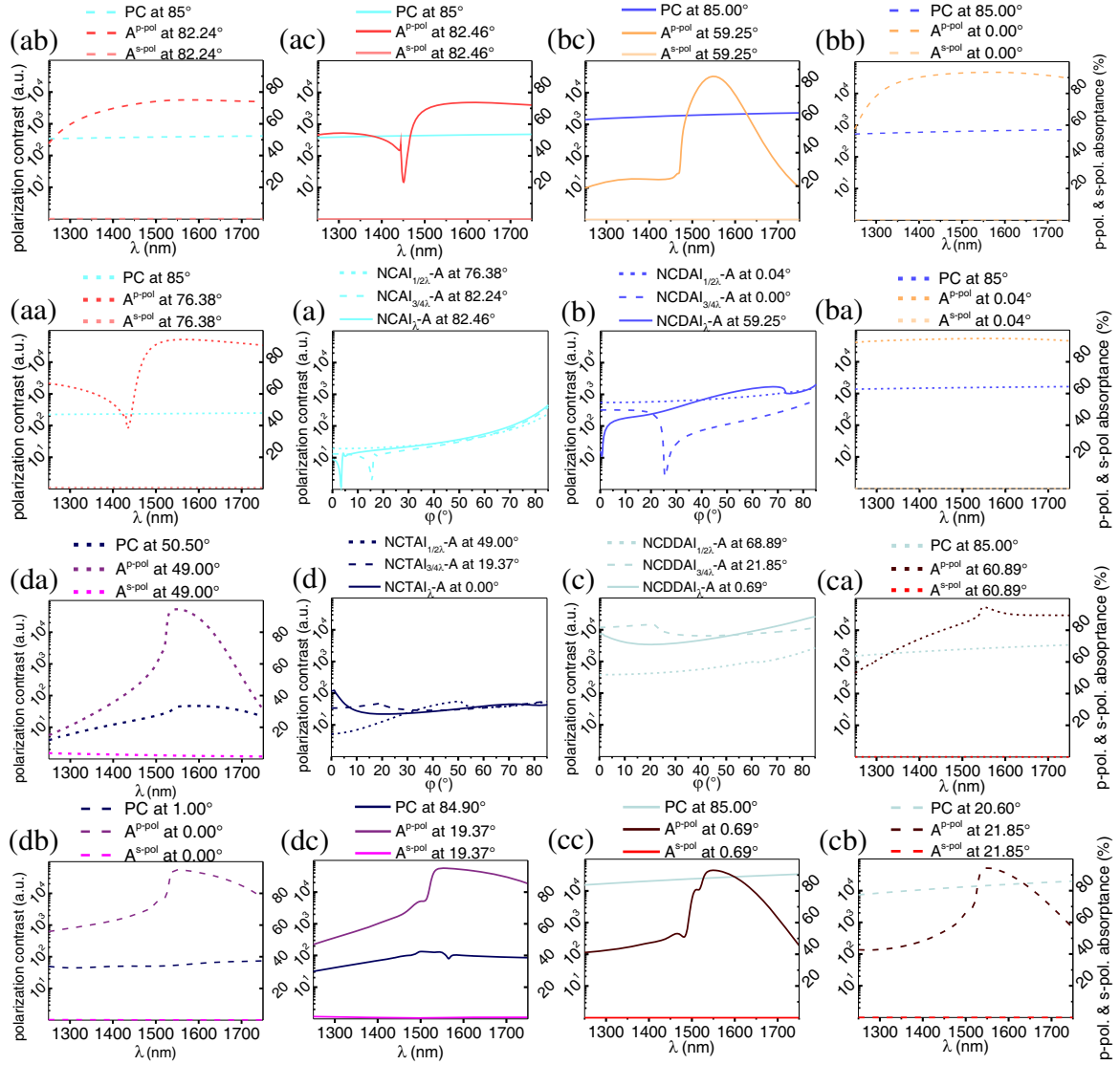
Figure 5. Polar-angle-dependent polarization contrast achievable via (a) NCAI-, (b) NCDAl-, (c) NCDDAl- and (d) NCTAl-A-SNSPD. Wavelength-dependent polarization contrast (PC) at contrast maxima and wavelength-dependent p -polarized ( A^{p-pol} ) and s -polarized ( A^{s-pol} ) absorptance at absorptance maxima in (aa) NCAI_{1/2*\lambda^-} , (ab) NCAI_{3/4*\lambda^-} , (ac) NCAI_{\lambda^-} , (ba) NCDAl_{1/2*\lambda^-} , (bb) NCDAl_{3/4*\lambda^-} , (bc) NCDAl_{\lambda^-} , (ca) NCDDAl_{1/2*\lambda^-} , (cb) NCDDAl_{3/4*\lambda^-} , (cc) NCDDAl_{\lambda^-} , (da) NCTAl_{1/2*\lambda^-} , (db) NCTAl_{3/4*\lambda^-} and (dc) NCTAl_{\lambda^-} -A-SNSPD.
