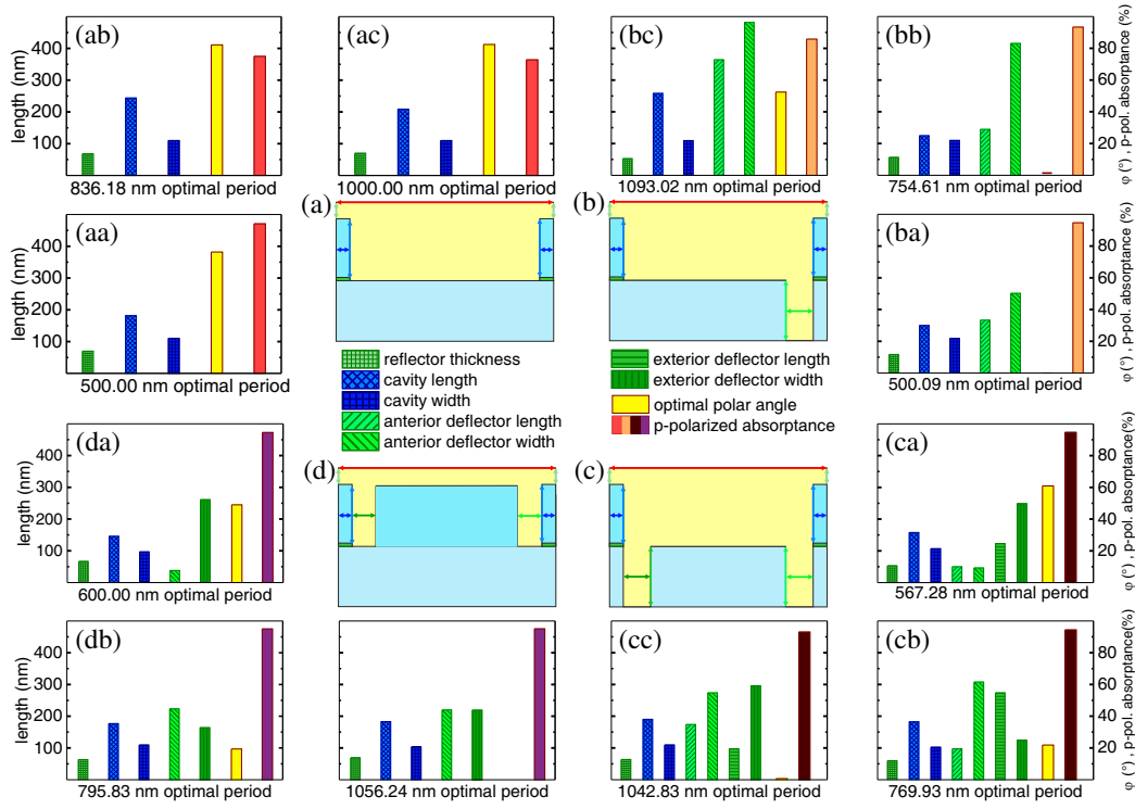
Figure 2. Schematics of geometry optimization method of (a) NCAI-, (b) NCDAl-, (c) NCDDAl- and (d) NCTAI-A-SNSPD. Histograms showing the optimized geometrical parameters, p -polarized absorptance and optimal polar angle in (aa) NCAI _{1/2*\lambda^-} , (ab) NCAI _{3/4*\lambda^-} , (ac) NCAI _{\lambda^-} , (ba) NCDAl _{1/2*\lambda^-} , (bb) NCDAl _{3/4*\lambda^-} , (bc) NCDAl _{\lambda^-} , (ca) NCDDAl _{1/2*\lambda^-} , (cb) NCDDAl _{3/4*\lambda^-} , (cc) NCDDAl _{\lambda^-} , (da) NCTAI _{1/2*\lambda^-} , (db) NCTAI _{3/4*\lambda^-} and (dc) NCTAI _{\lambda^-} -A-SNSPD.
