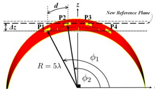
Figure 6. Convex bending geometry to calculate the required phase shift for gain compensation.
