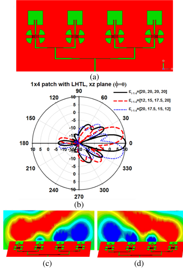
Figure 8. The 1 \times 4 phased array using BST/polymer based LHTL phase shifter with radial stubs: (a) top view, (b) E -plane radiation pattern for various steered beam, and (c) E -field maps for steered beams.
