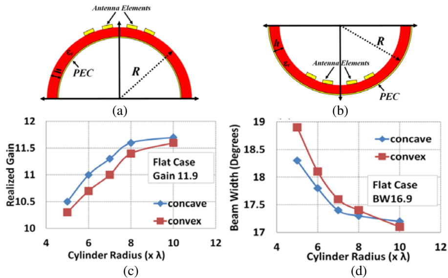
Figure 5. Schematic of the antenna array with (a) convex bending and (b) concave bending, and the bending effects for various concave and convex geometries (c) on the simulated maximum gain in dB and (d) on the beam width in degrees.
