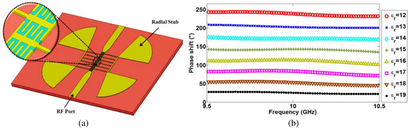
Figure 3. BST/polymer composite based LHTL phase shifter with radial stubs: (a) schematic of the design, (b) simulated phase shifts in degrees for various values of the dielectric constant.
