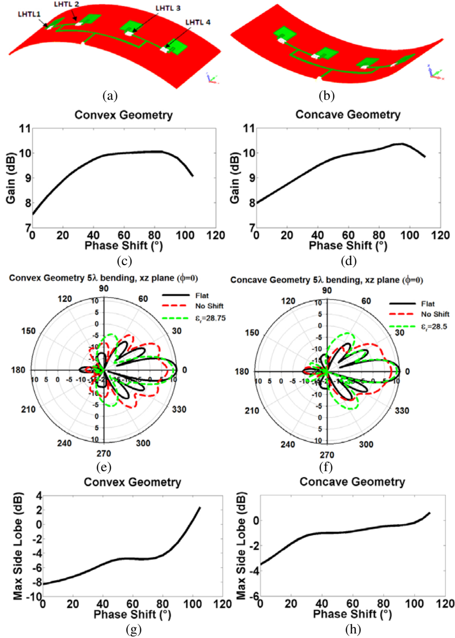
Figure 7. The conformal antenna array with (a) convex and (b) concave bending, the simulated gain in dB versus corresponding phase shift for the array with (c) convex and (d) concave geometry, the simulated E -plane radiation pattern for the array with (e) convex and (f) concave geometry, and the simulated maximum side lobe level for the array with (g) convex and (h) concave geometry.
