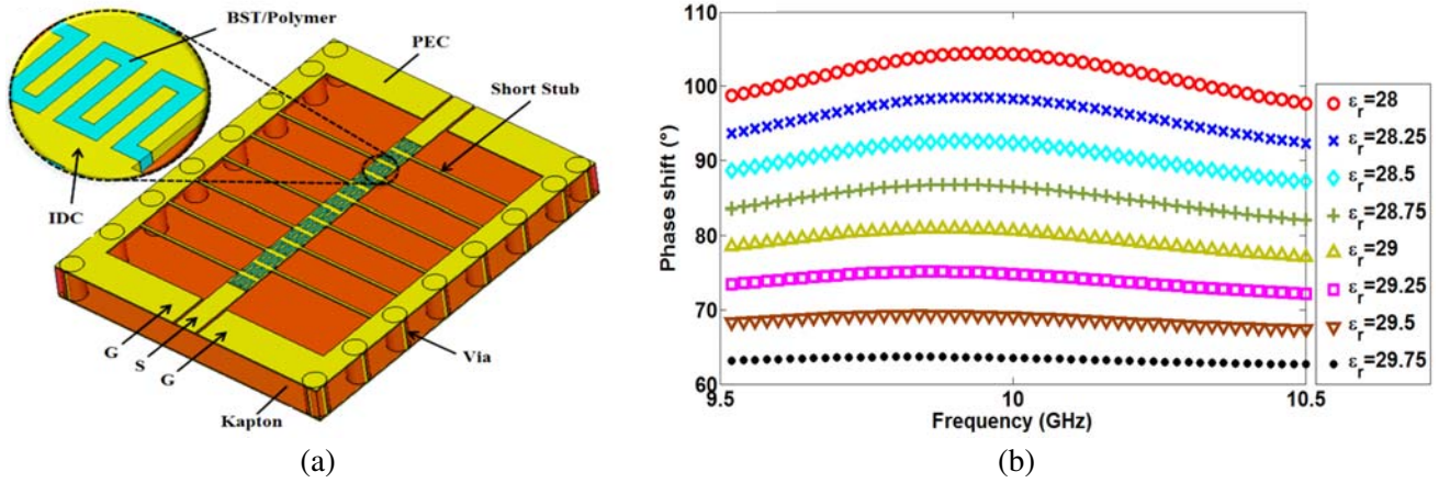
Figure 1. BST/polymer composite based CPW LHTL phase shifter: (a) schematic of the design, (b) simulated phase shifts in degrees for different values of dielectric constant.
