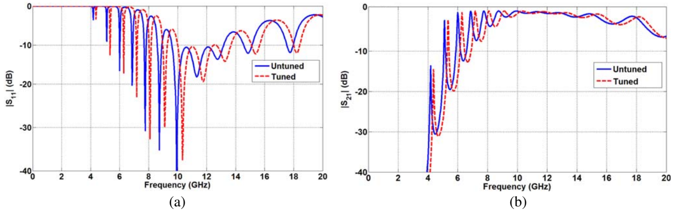
Figure 2. Simulated results of BST/polymer composite based CPW LHTL phase shifter: (a) |S_{11}| in dB, and (b) simulated |S_{21}| in dB.
