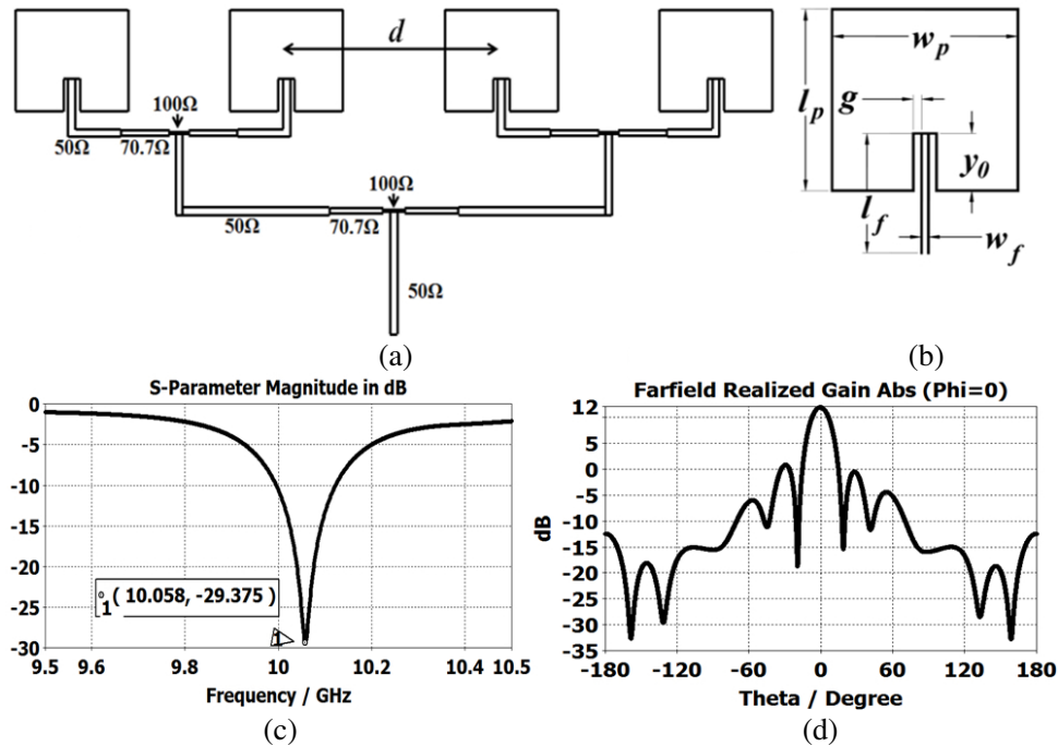
Figure 4. Rectangular patch antenna: (a) top view of a 1 \times 4 array, (b) top view of a single patch, (c) |S_{11}| in dB, (d) realized farfield gain in dB at resonance.
