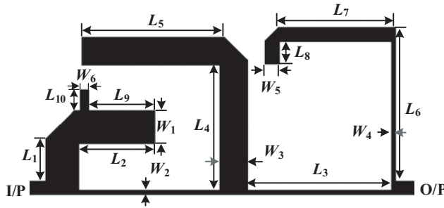
Figure 5. Layout of the proposed bandpass filter with ten transmission zeros.
