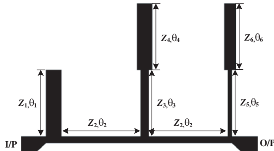
Figure 1. Configuration of the bandpass filter with ten transmission zeros.
