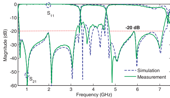
Figure 7. Simulated and measured results of the bandpass filter with ten transmission zeros.
