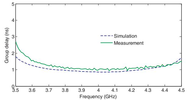
Figure 8. Simulated and measured group delay ( S_{21} ) of the bandpass filter with ten transmission zeros.
