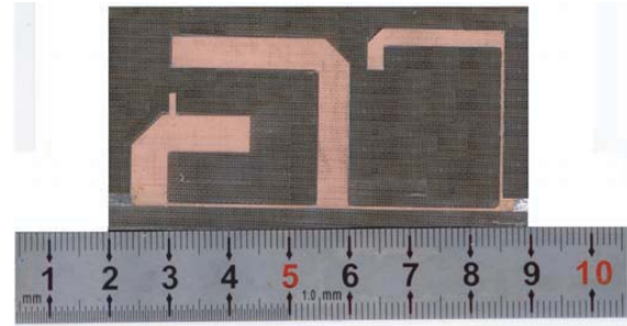
Figure 6. Photograph of the fabricated bandpass filter with ten transmission zeros.
