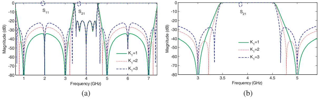
Figure 2. Simulated S -parameters of the bandpass filter with ten transmission zeros under different impedance ratio K_1 . ( K_1 = 1 , K_2 = 1 , Z_1 = 23 \Omega , Z_2 = 163 \Omega , Z_3 = 26.5 \Omega , Z_5 = 44.5 \Omega ; K_1 = 2 , K_2 = 1 , Z_1 = 23 \Omega , Z_2 = 152 \Omega , Z_3 = 47.3 \Omega , Z_5 = 44.5 \Omega ; K_1 = 3 , K_2 = 1 , Z_1 = 23 \Omega , Z_2 = 138.5 \Omega , Z_3 = 80 \Omega , Z_5 = 44.5 \Omega ).
