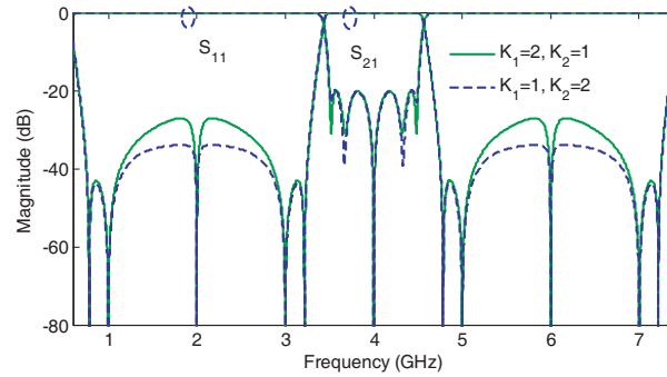
Figure 4. Simulated S -parameters of the bandpass filter with ten transmission zeros under different K_1 and K_2 . ( K_1 = 2 , K_2 = 1 , Z_1 = 23 \Omega , Z_2 = 152 \Omega , Z_3 = 47.3 \Omega , Z_5 = 44.5 \Omega ; K_1 = 1 , K_2 = 2 , Z_1 = 23 \Omega , Z_2 = 161.5 \Omega , Z_3 = 26.5 \Omega , Z_5 = 7 \Omega ).
