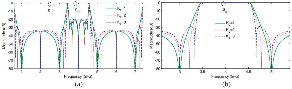
Figure 3. Simulated S -parameters of the bandpass filter with ten transmission zeros under different impedance ratio K_2 . ( K_1 = 1 , K_2 = 1 , Z_1 = 23 \Omega , Z_2 = 163 \Omega , Z_3 = 26.5 \Omega , Z_5 = 44.5 \Omega ; K_1 = 1 , K_2 = 2 , Z_1 = 23 \Omega , Z_2 = 161.5 \Omega , Z_3 = 26.5 \Omega , Z_5 = 77 \Omega ; K_1 = 1 , K_2 = 3 , Z_1 = 23 \Omega , Z_2 = 159.5 \Omega , Z_3 = 26.5 \Omega , Z_5 = 136 \Omega ).
