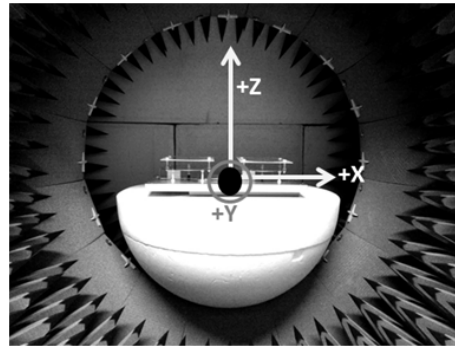
Figure 9. Antenna array placement in the measurement chamber.
