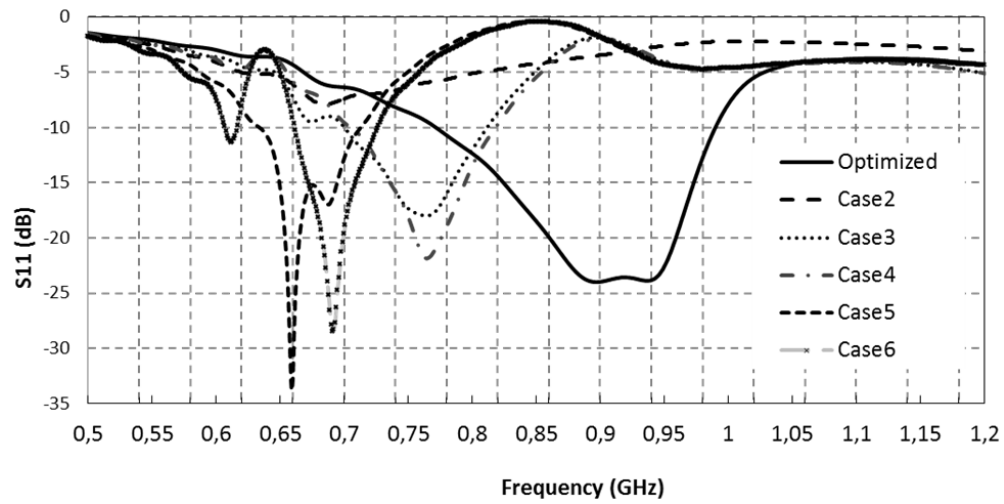
Figure 4. Simulated reflection coefficients for different patch shape combinations defined in Table 1.
