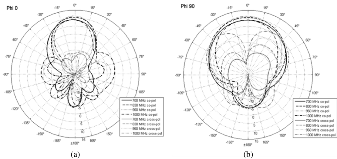
Figure 12. (a) Measured radiation pattern at array E -plane cut, (b) radiation pattern at array H -plane cut.
