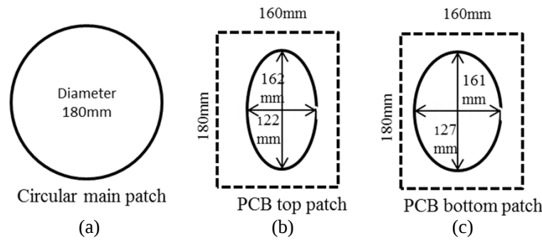
Figure 2. (a) Circular main patch. (b) Elliptical patch on PCB top. (c) Elliptical patch on PCB bottom.
