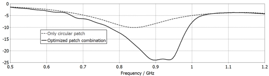
Figure 5. Simulated reflection coefficients for only circular patch and optimized patch combination.
