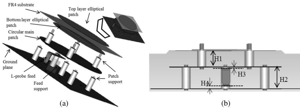
Figure 1. (a) Elevated single element patch 3D shape. (b) Side view single element, spacing between circular patch and PCB, H1 = 25 mm, spacing between circular patch and ground, H2 = 33.6 mm, spacing between circular patch and L-probe fed H3 = 1.2 mm, spacing between L-probe fed bottom and ground, H4 = 4 mm.
