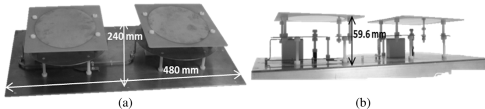
Figure 7. (a) Two-element array structure. (b) Patch and fed line fixing mechanics.
