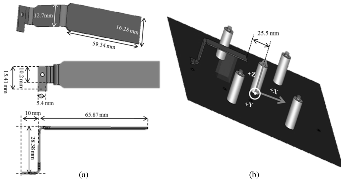
Figure 3. (a) L-probe fed structure. (b) Circular patch center and L-probe edge spacing.
