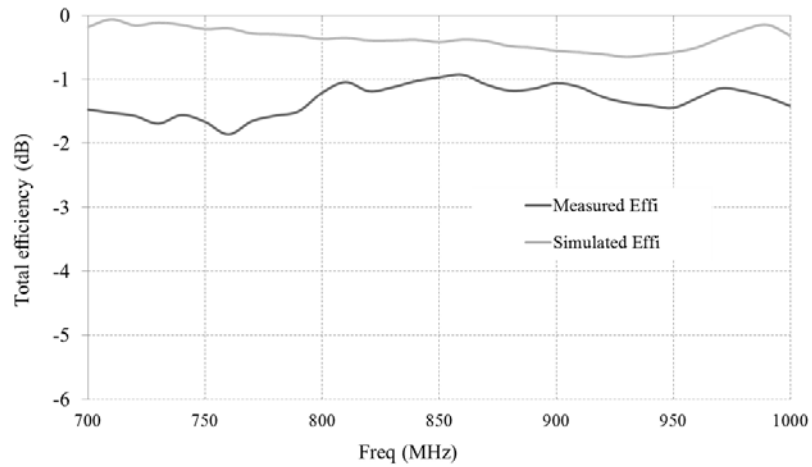
Figure 10. Measured and simulated total efficiency for antenna array.
