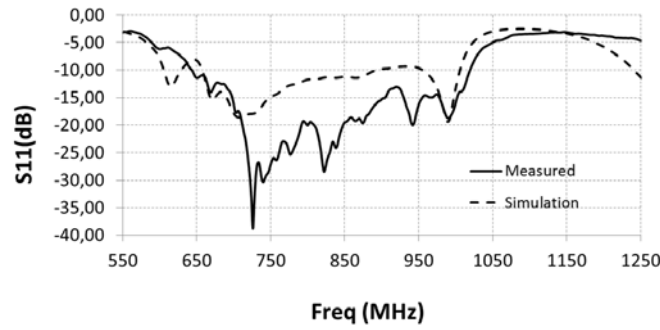
Figure 8. Measured and simulated reflection coefficients for the two-element array.
