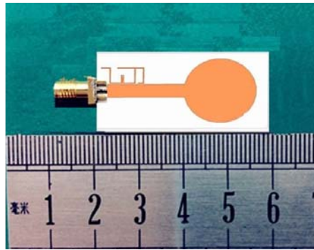
Figure 7. Photograph of the fabricated UWB antenna with triple-notched bands.
