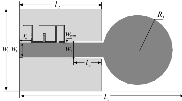
Figure 1. Layout of the proposed UWB antenna with triple notched-bands.
