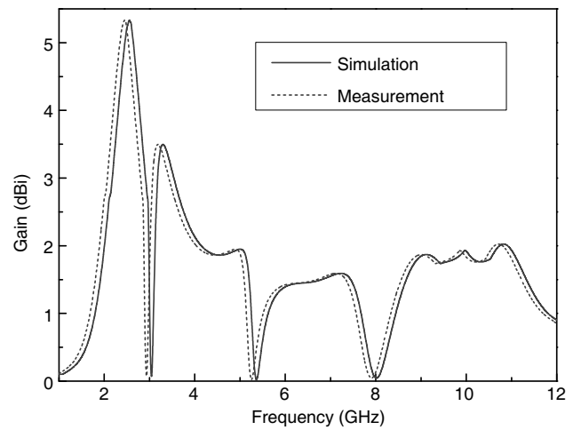
Figure 6. Measured and simulated peak gain of the proposed UWB antenna with triple-notched bands.
