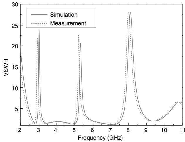
Figure 5. Measurement and simulation of VSWR.
