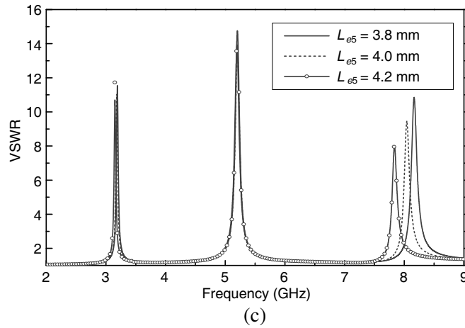
Figure 3. Simulated VSWR of the coupled triple-mode SLR for various dimensions: (a) L_{e2} , (b) L_{e4} , (c) L_{e5} .
