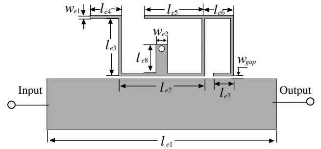
Figure 2. Geometry of proposed triple-mode SLR.
