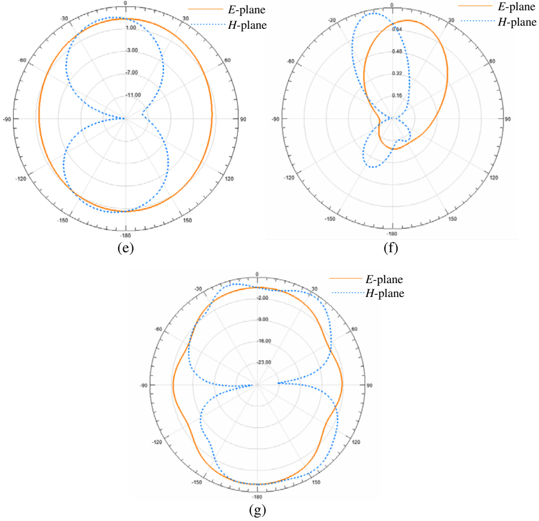
Figure 4. Measured radiation pattern of the UWB planar monopole antenna: (a) 2.5 GHz, (b) 3.0 GHz, (c) 5.0 GHz, (d) 5.2 GHz, (e) 7.5 GHz, (f) 8.0 GHz, (g) 10.0 GHz.
