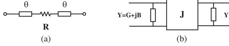
Figure 4. Resistive coupling structure: (a) the circuit to be realized; and (b) the equivalent circuit.
