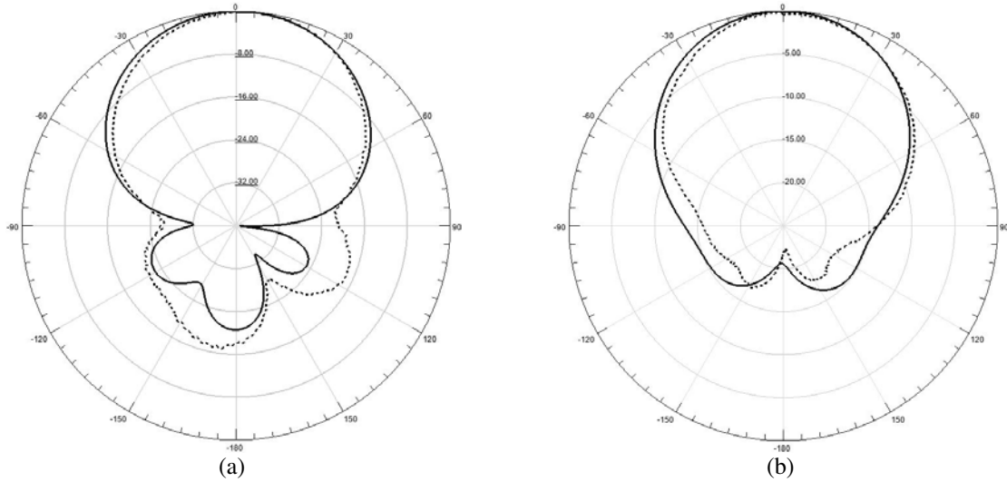
Figure 5. Normalized radiation pattern for the proposed design. (a) E -plane; (b) H -plane. Solid line, simulated; dotted line, measured.
