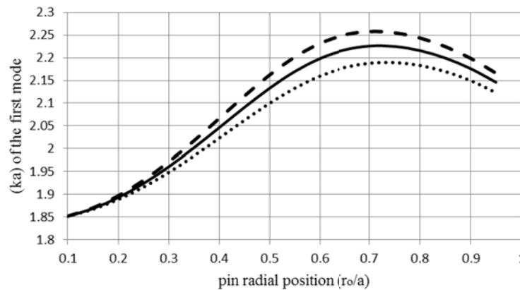
Figure 2. The normalized resonant frequency of the dominant mode for the single pin patch. Dashed line ( b/a = 0.04 ), solid line ( b/a = 0.03 ) and dotted line ( b/a = 0.02 ).
