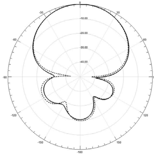
Figure 6. Simulated radiation patterns ( E -plane) for the proposed inhomogeneous design (solid) and the same design with homogeneous dielectric with permittivity of 1.46 (dotted).
