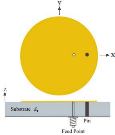
Figure 1. Geometry of the proposed antenna with a probe feed.
