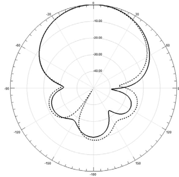
Figure 8. Normalized radiation pattern ( E -plane) for both designs. Single pin (solid) and two-pin (dotted).
