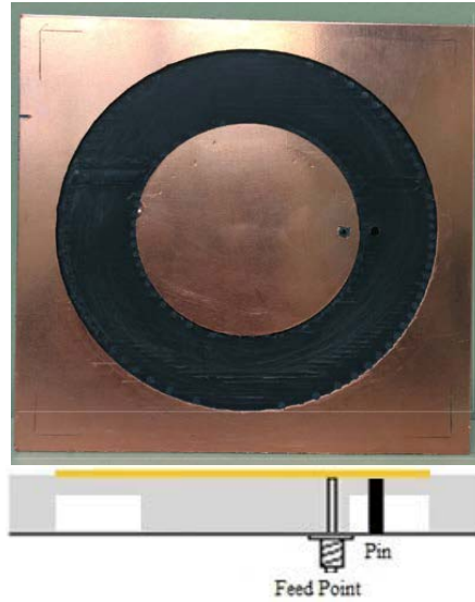
Figure 3. The back side of the fabricated design with a side view of its geometry (with the ground plane removed).
