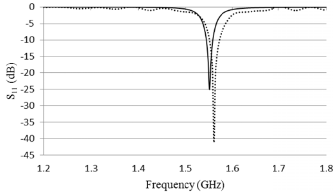
Figure 4. Reflection coefficient |S_{11}|_{dB} of the proposed design. Simulation results (solid) and experimental results (dotted).
