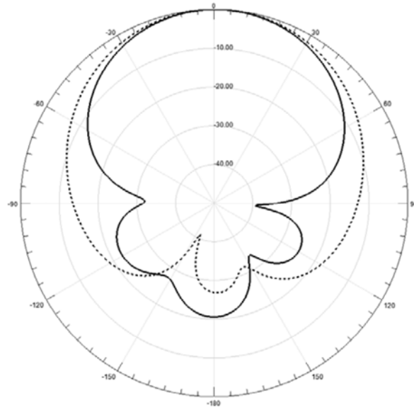
Figure 7. Comparison between simulated radiation patterns of the pin loaded design and conventional unloaded circular patch ( E -plane). Pin loaded (solid) and unloaded (dotted).
