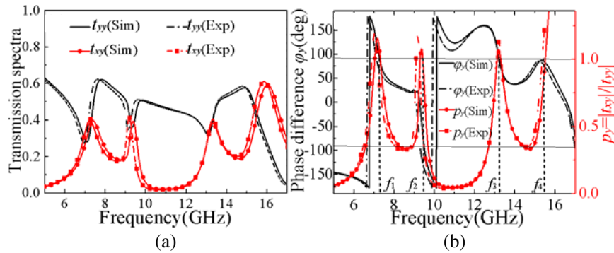
Figure 2. Simulated and measured results for the designed CMM: (a) the co- and cross-polarization transmission coefficients ( t_{yy} and t_{xy} ), (b) the ratio p_y and phase difference \phi_y between the co- and cross-polarization.
