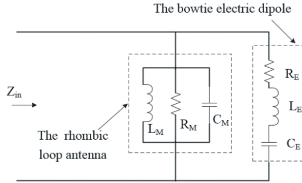
Figure 2. Simplified equivalent circuit of the electrical-magnetic composite patch antenna.
