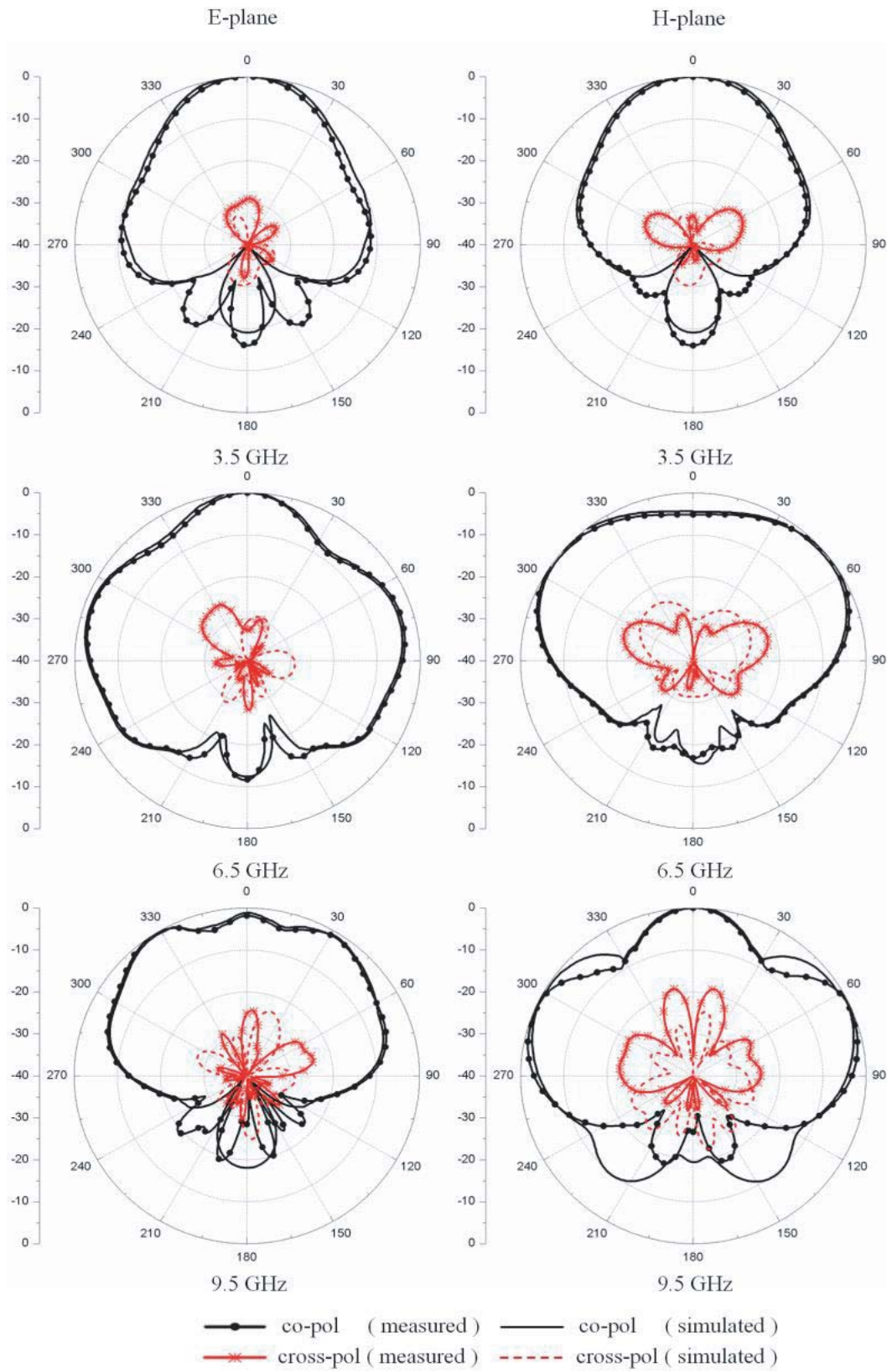
Figure 7. Measured and simulated radiation patterns at 3.5, 6.5 and 9.5 GHz.
