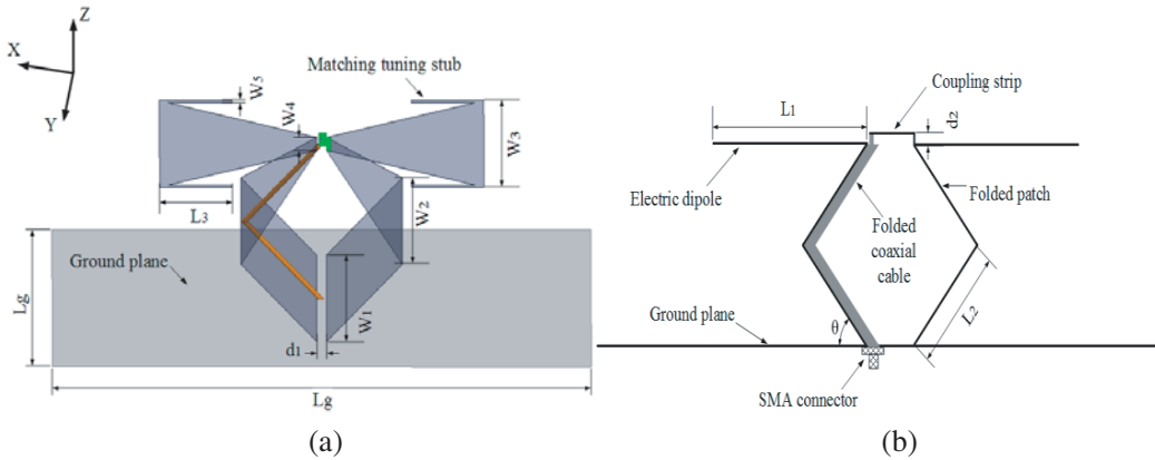
Figure 1. Geometry of the electrical-magnetic composite antenna: (a) 3D view; (b) Side view.
