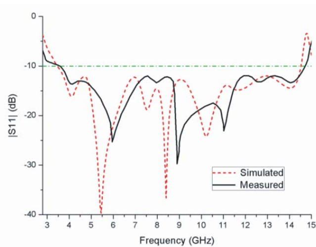
Figure 6. Measured and simulated |S_{11}| against frequency.
