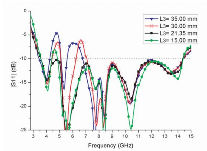
Figure 4. Effects of various tuning stubs' length L_3 .
