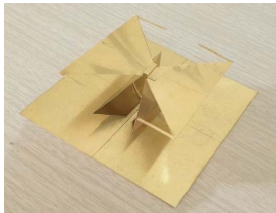
Figure 5. Picture of the manufactured antenna.
