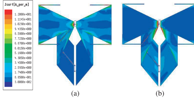
Figure 3. Current distributions of the dipole-loop composite antenna at different times: (a) t = 0 ( T/2 ); (b) t = T/4 ( 3T/4 ).
