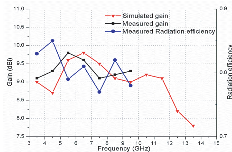
Figure 8. Gains and radiation efficiency of the proposed antenna.
