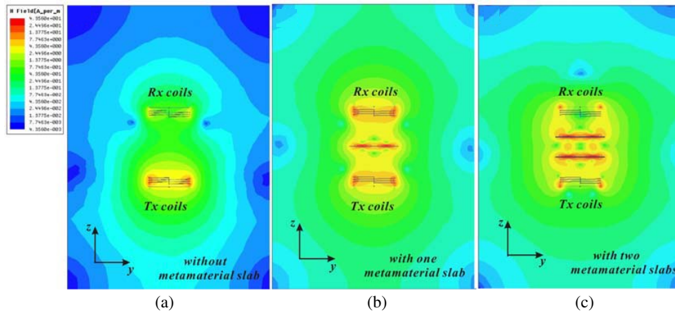
Figure 5. Comparison of magnetic field distribution of WPT system, (a) without MM slab, (b) with one MM slab, (c) with two MM slabs.
