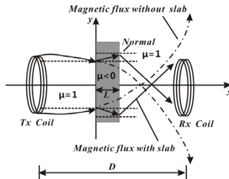
Figure 1. System configuration for the analysis of divergent field focus effect through MM slab.
