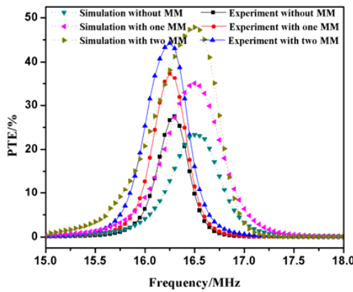
Figure 9. Comparison of simulation and measured PTEs in 3 different cases at a distance of 30 cm.
