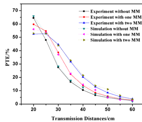
Figure 10. Comparison of simulation and measured PTEs versus transmission distances.
