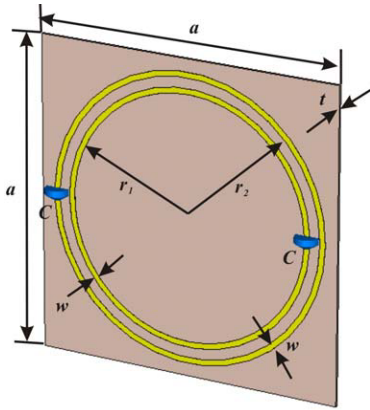
Figure 2. Schematic diagram of unit cell of CLSRRs.
