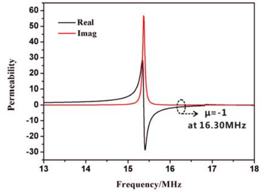
Figure 3. Simulated results of CLSRRs, retrieved effective permeability.
