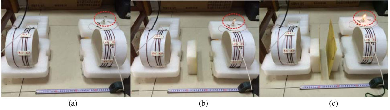
Figure 11. WPT experiment to a 10W light bulb. Pictures are taken with same settings. (a) Traditional system without MM slab, (b) system with one MM slab, and (c) system with two MM slabs.
