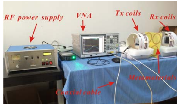
Figure 8. Photograph of the experiment setup of metamaterial-based WPT system.
