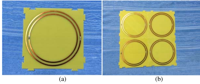
Figure 7. Photographs of the fabricated assembled CLSRRs slabs. (a) 1 \times 1 unit cell, (b) 2 \times 2 unit cells.
