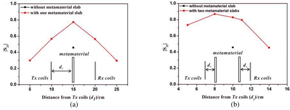
Figure 6. |S_{21}| versus the distance of the MM slab from Tx coils ( d_1 ), (a) with one MM slab, (b) with two MM slabs.
