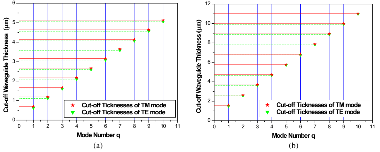
Figure 2. Comparison of the cut-off thicknesses of non uniform optical waveguide for the modes: 1 \leq p \leq 10 , of TE mode (▼ points) and TM mode (* points) applying the exact Fresnel coefficient given in Eq. (1). (a) Air/polymer/SiO 2 waveguide. (b) Air/AsGa/AlAsGa waveguide.
