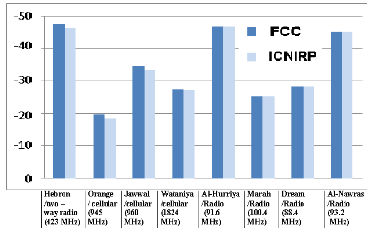
Figure 3. 10 \log(Pd_{30m}/Pd_{safe} \text{ threshold}) in dB vs. transmitting towers where the safe threshold power density is referenced to FCC and ICNIRP respectively.
