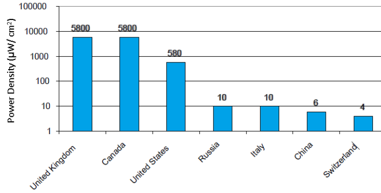
Figure 2. Some international exposure standards at cell phone frequencies (800–900 MHz).
