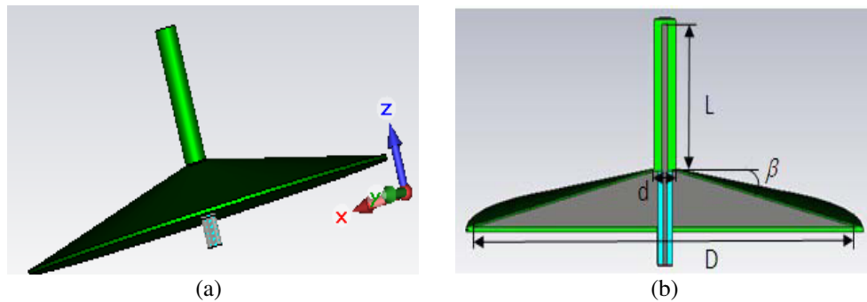
Figure 3. Geometry of the conical ground plane monopole antenna; (a) 3-D view, (b) center cut side view.
