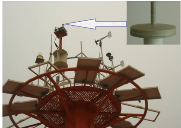
Figure 12. The antenna installed on the top of the oceanic buoy platform.
