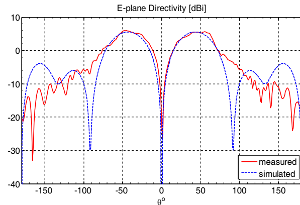
Figure 11. The measured directivity of the manufactured antenna at 5.885 GHz.
