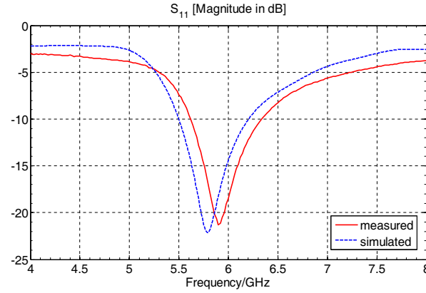
Figure 10. The measured magnitude of S_{11} of the monopole antenna.
