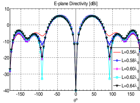
Figure 7. Parameter L sweep for patterns (other parameters are set as in Table 1).
