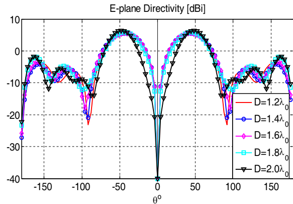
Figure 9. Parameter D sweep for patterns (other parameters are set as in Table 1).
