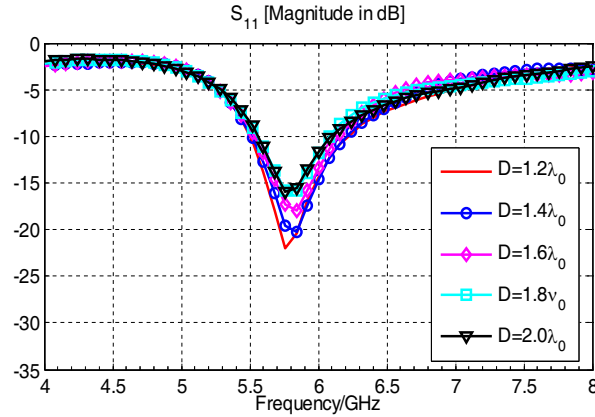
Figure 6. Parameter D sweep for S_{11} (other parameters are set as in Table 1).
