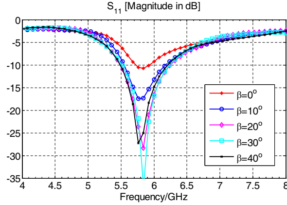
Figure 5. Parameter \beta sweep for S_{11} (other parameters are set as in Table 1).
