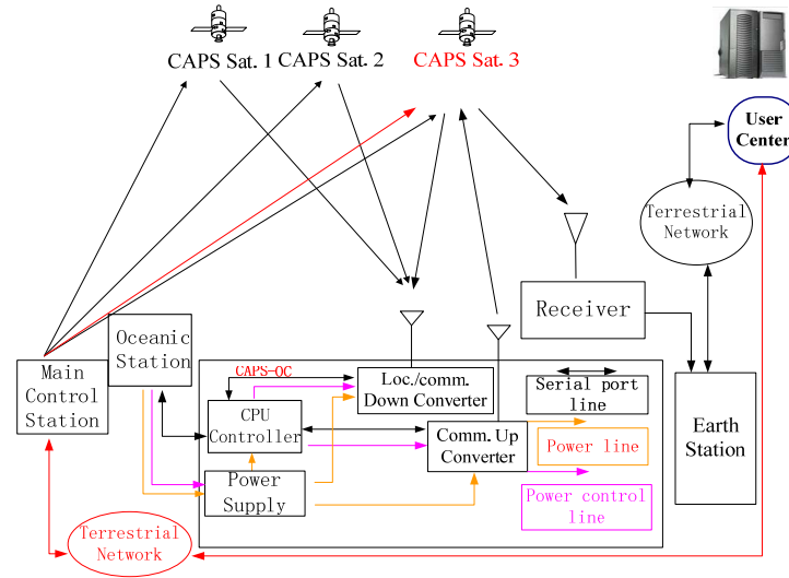
Figure 1. Operational principle of the CAPS experimental system.
