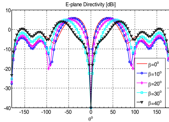
Figure 8. Parameter \beta sweep for patterns (other parameters are set as in Table 1).
