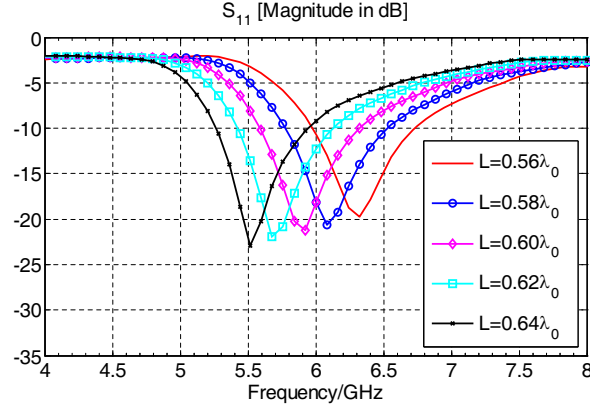
Figure 4. Parameter L sweep for S_{11} (other parameters are set as in Table 1).
