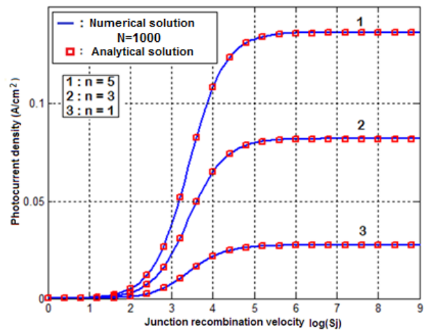
Figure 13. Photocurrent density versus Sj for various values of illumination level n : D = 26 cm 2 /s; L = 0.01 cm; Sb = 10^3 cm/s, front surface illumination.
