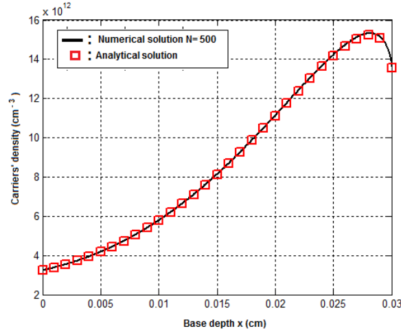
Figure 7. Minority carrier's density; D = 26 \text{ cm}^2/\text{s} ; L = 0.01 \text{ cm} ; Sb = 10^3 \text{ cm/s} , back surface illumination.
