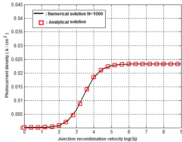
Figure 12. Photocurrent density versus Sj ; D = 26 cm 2 /s; L = 0.01 cm; Sb = 10^3 cm/s, front surface illumination.
