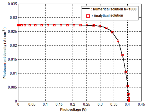
Figure 16. Current-voltage characteristics; D = 26 \text{ cm}^2/\text{s} ; L = 0.01 \text{ cm} ; Sb = 10^3 \text{ cm/s} , front surface illumination.
