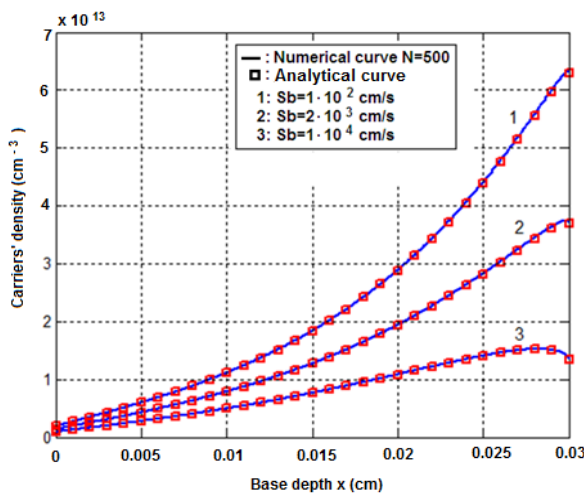
Figure 8. Minority carriers density for various back surface recombination velocities Sb : D = 26 \text{ cm}^2/\text{s} ; L = 0.01 \text{ cm} ; Sj = 10^4 \text{ cm/s} , back surface illumination.
