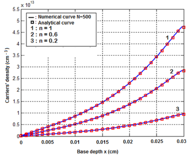
Figure 9. Minority carriers density for various values of n : D = 26 \text{ cm}^2/\text{s} ; L = 0.01 \text{ cm} ; Sj = 10^5 \text{ cm/s} , Sb = 10^3 \text{ cm/s} , back surface illumination.
