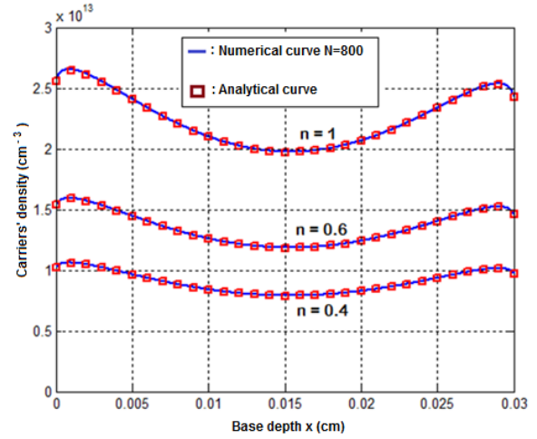
Figure 11. Minority carrier's density for various values of n : D = 26 cm 2 /s; L = 0.01 cm; Sj = 4, 6 \times 10^3 cm/s; Sb = 5 \times 10^3 cm/s, simultaneous illumination.
