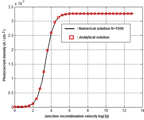
Figure 14. Photocurrent density versus Sj : D = 26 \text{ cm}^2/\text{s} ; L = 0.01 \text{ cm} ; Sb = 10^3 \text{ cm/s} , back surface illumination.
