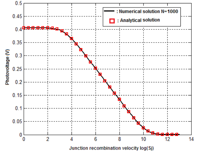
Figure 15. Photovoltage versus junction recombination velocity Sj : D = 26 \text{ cm}^2/\text{s} ; L = 0.01 \text{ cm} ; Sb = 10^3 \text{ cm/s} , front illumination.
