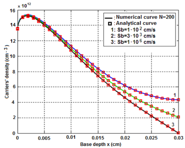
Figure 5. Minority carriers density for various junction recombination velocities S_b : D = 26 \text{ cm}^2/\text{s} ; L = 0.01 \text{ cm} ; S_j = 10^3 \text{ cm/s} , front surface illumination.
