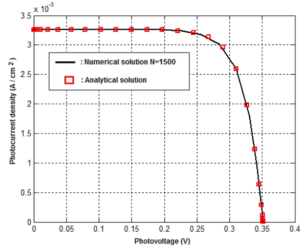
Figure 17. Current-voltage characteristics; D = 26 \text{ cm}^2/\text{s} ; L = 0.01 \text{ cm} ; Sb = 10^3 \text{ cm/s} , back surface illumination.
