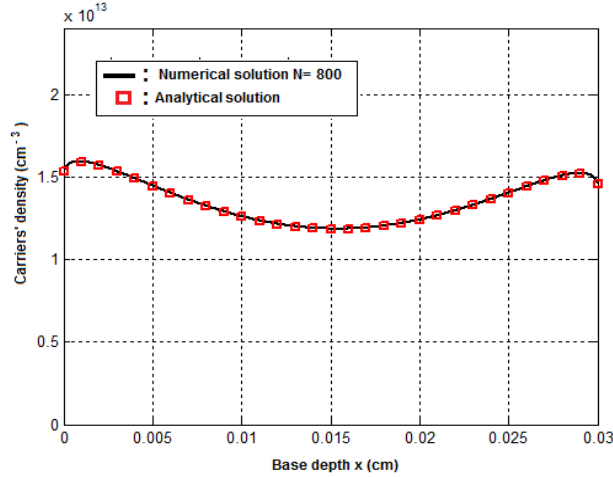
Figure 10. Minority carrier's density; Sj = 10^4 cm/s; D = 26 cm 2 /s; L = 0.01 cm; Sb = 10^4 cm/s, simultaneous illumination.
