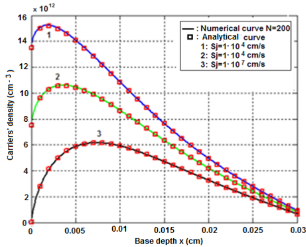
Figure 4. Minority carriers density for various junction recombination velocities S_j : D = 26 \text{ cm}^2/\text{s} ; L = 0.01 \text{ cm} ; S_b = 10^3 \text{ cm/s} , front surface illumination.
