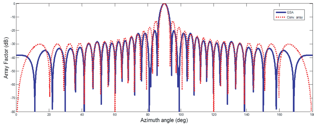
Figure 4. Normalized array factor of the 32-element linear array obtained using GSA and Conventional array with prescribed null at 99^\circ .
