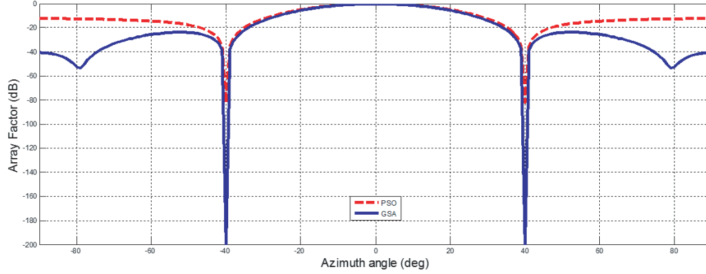
Figure 7. The produced radiation pattern with one symmetric null imposed at 40^\circ .
