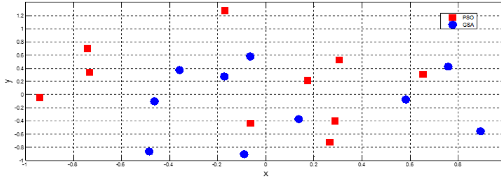
Figure 8. Normalized positions of the elements in wavelengths synthesized for one null pattern using GSA & PSO.
