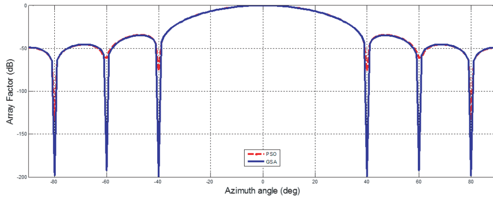
Figure 9. The produced radiation pattern with three nulls imposed at 40^\circ , 60^\circ and 80^\circ .
