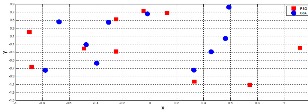
Figure 10. Normalized positions of the elements in wavelengths synthesized for three nulls pattern using GSA & PSO.
