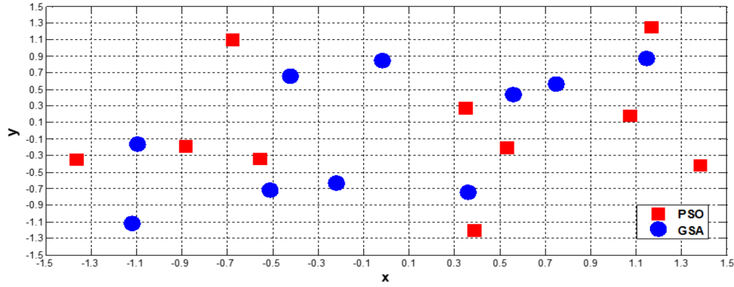
Figure 12. Normalized positions of the elements in wavelengths synthesized for four nulls pattern using GSA & PSO.
