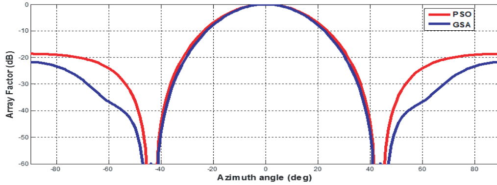
Figure 13. The produced radiation pattern with broad null at 41^\circ to 47^\circ .
