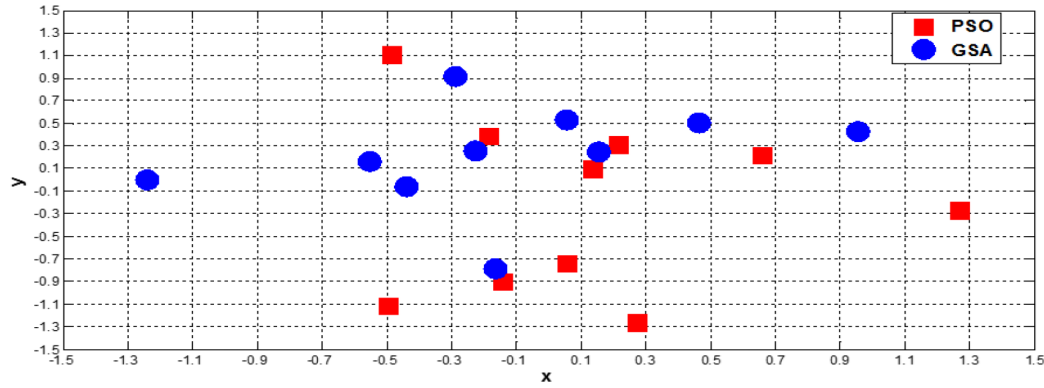
Figure 14. Normalized positions of the elements in wavelengths synthesized for broad null pattern using GSA and PSO.
