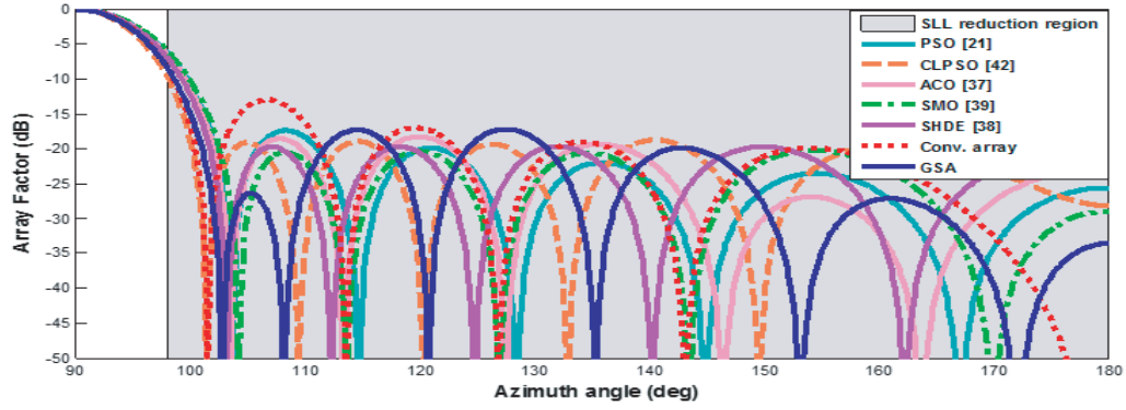
Figure 3. Normalized array factor of the 10-element linear array obtained using GSA algorithm compared with PSO [21], Comprehensive Learning Particle Swarm Optimization (CLPSO) [42], Ant Colony Optimization (ACO) [37], Spider Monkey Optimization (SMO) [39], Self-adaptive Hybrid Differential Evolution algorithm (SHDE) [38] and conventional array. The region of suppressed SLL is [98^\circ \ 180^\circ] .
