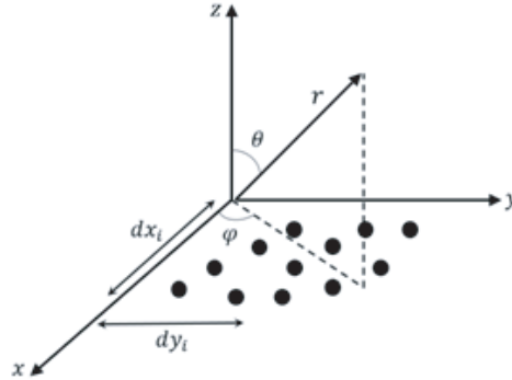
Figure 6. Geometry of N elements planar array.
