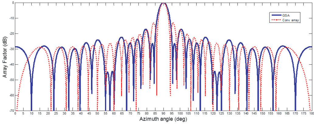
Figure 5. Normalized array factor of the 28-element linear array obtained using GSA and conventional array with three desired nulls at 120^\circ , 122.5^\circ and 125^\circ angles.
