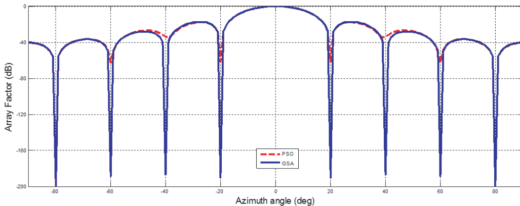
Figure 11. The produced radiation pattern with four symmetric nulls imposed at 20^\circ , 40^\circ , 60^\circ and 80^\circ .
