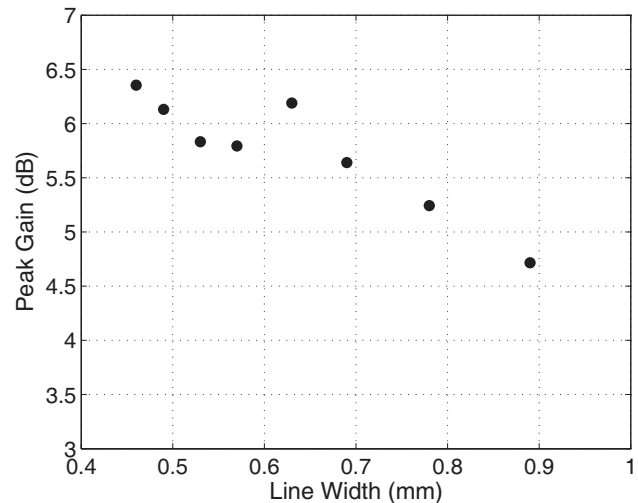
Figure 13. Effect of linewidth on peak gain of circular meshed patch ( T_{\text{circ}} = 60\% ).
