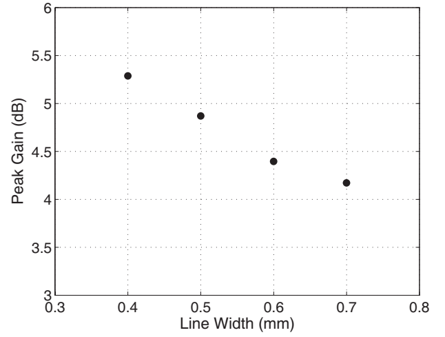
Figure 7. Effect of current path lines on peak gain of rectangular meshed patch ( T_{rect} \approx 70\% ).
