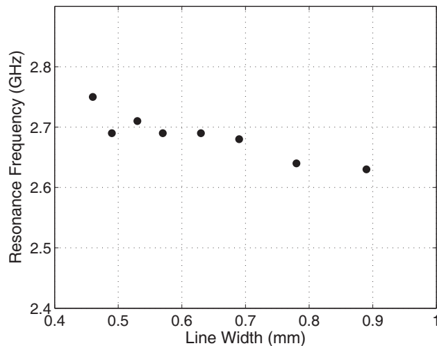
Figure 12. Effect of linewidth on resonant frequency of circular meshed patch ( T_{\text{circ}} = 60\% ).
