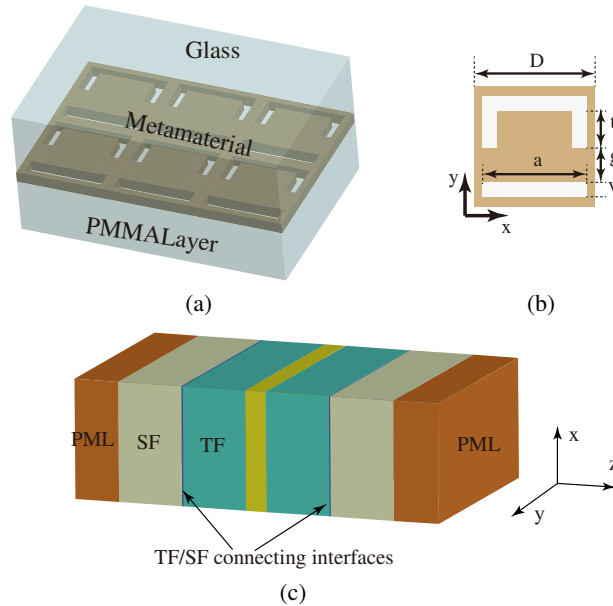
Figure 2. (a) Schematic pattern of the metamaterial comprising a periodic array of complementary SRRs. (b) The feature size of a unit cell. D = 540 nm, lateral slit a = 470 nm, top vertical slit and gap t = g = 170 nm, and slit width w = 65 nm. (c) Configuration for the FDTD method. PMLs were set to be in the z direction and periodic boundary conditions were used at the both x and y directions.
