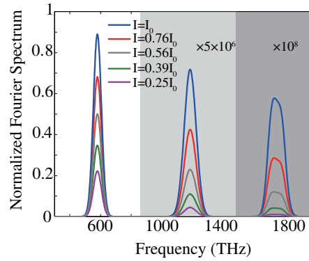
Figure 6. Nonlinear scattering spectra for a 20 nm radius gold nanosphere under different pump power.
