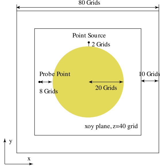
Figure 9. The FDTD simulation setup. The electric field was recorded at the probe point.
