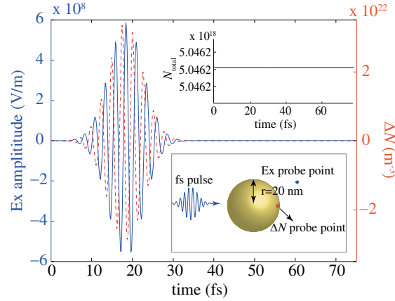
Figure 5. The E_x component of scattered field (blue solid line) and the fluctuation of charge density on the nanosphere surface (dashed red line), plotted vs. time. The upper inset shows the temporal evolution of the overall electron charges within the nanosphere. The bottom inset schematically shows the simulation configuration for modeling the nonlinear generations of harmonics for the gold nanosphere.
