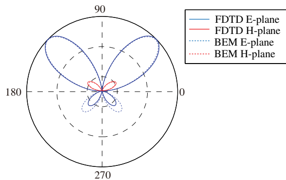
Figure A1. Second-harmonic radiation pattern of a 100 nm radius gold sphere calculated by the boundary element method (BEM) and the proposed FDTD method. The computational configuration for the BEM can be found in our published work [17].
