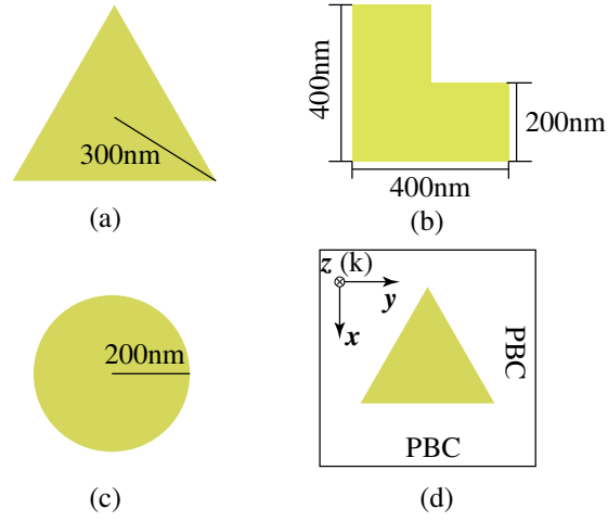
Figure 12. Unit cells of metasurfaces with different rotational symmetries. (a) A triangle rod with a three-fold rotational symmetry. (b) An L-shape with symmetry breaking. (c) A cylinder with a central symmetry. (d) Simulation layout for modeling the SHG from the metasurfaces illuminated by circularly polarized pulses.
