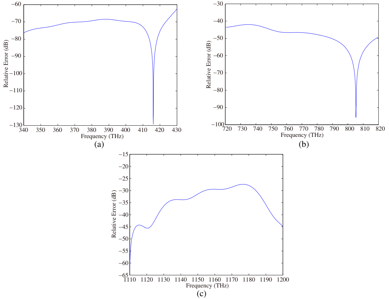
Figure 11. Reflection errors for the (a) linear scattered waves, (b) second harmonic waves and (c) third harmonic waves.
