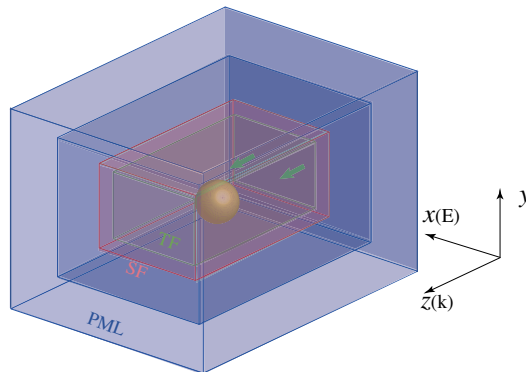
Figure 4. Layout of the simulation of nonlinear optical scattering from a gold nanosphere illuminated by a strong lasing pulse.
