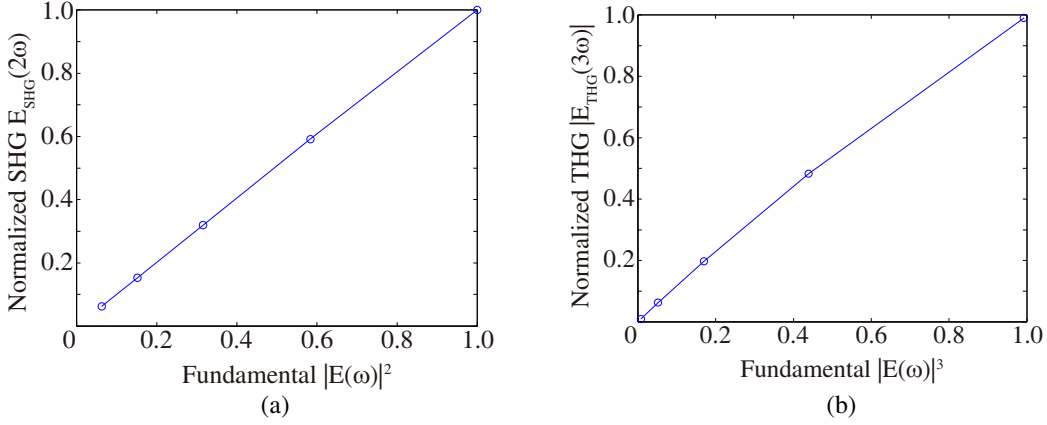
Figure 7. The peak intensities of the second and third harmonics vs. the second and third power of the fundamental intensities, respectively. (a) Second harmonics; (b) Third harmonics.
