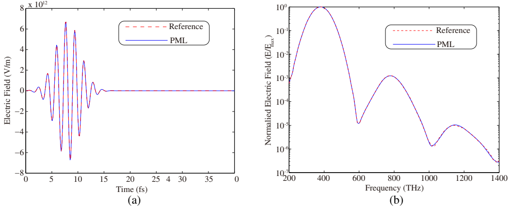
Figure 10. (a) Electric field as a function of time. (b) A semi-log plot of the Fourier transform of the electric field as a function of frequency with the logarithmic scale used for the y axis.
