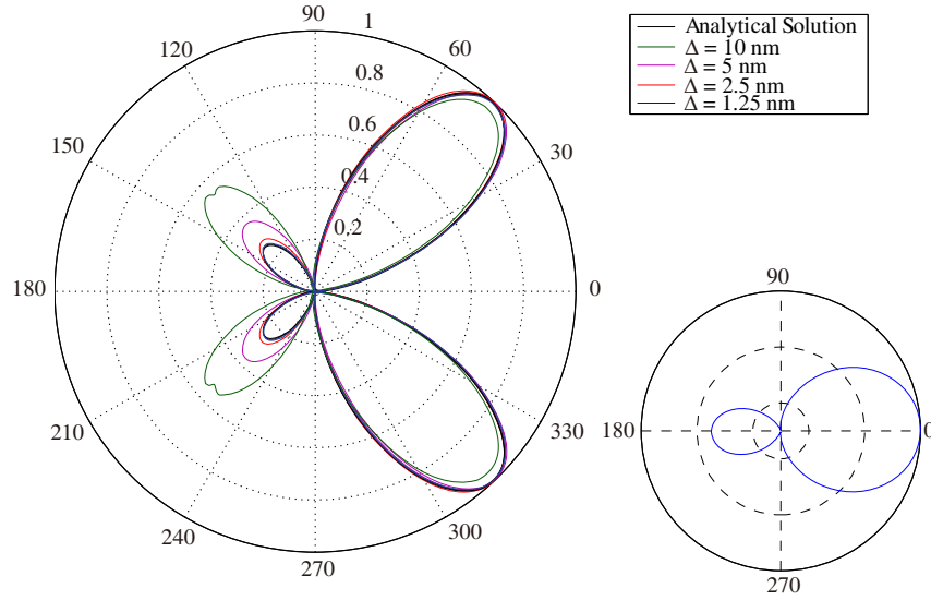
Figure 8. Second harmonic radiation diagrams as a function of \theta at \varphi = 0^\circ , for a gold nanosphere of radius R = 100 nm. The pump wavelength was \lambda = 780 nm and all curves were normalized by the maximum obtained for the result with \Delta = 1.25 nm. The right inset shows the radiation pattern at the fundamental frequency.
