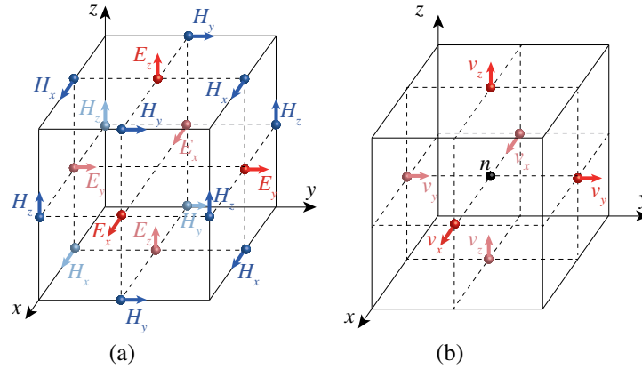
Figure 1. The Yee grids for the Maxwell-hydrodynamic system. (a) Maxwell's equations. (b) Hydrodynamic equations.
