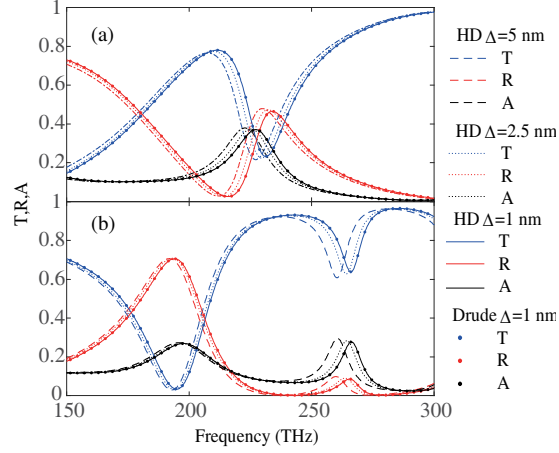
Figure 3. The calculated spectra of transmittance ( T(\omega) = |t(\omega)|^2 ), reflectance ( R(\omega) = |r(\omega)|^2 ), and absorptance ( A(\omega) = 1 - T(\omega) - R(\omega) ) for the metamaterial system in Fig. 2. The results are shown for (a) x -polarization and (b) y -polarization.
