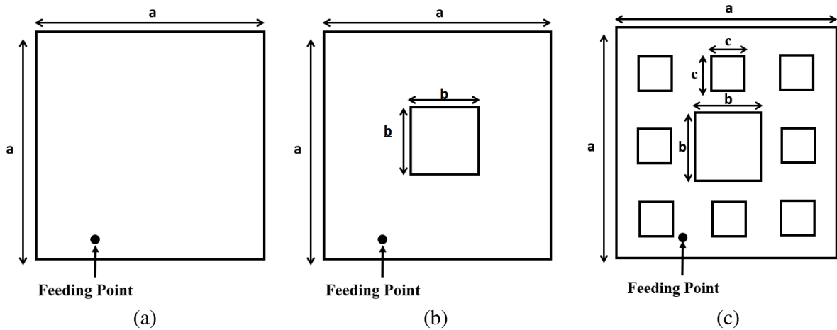
Figure 1. Sierpinski carpet fractal antenna geometry under consideration. (a) Zeroth Iteration. (b) First Iteration. (c) Second Iteration.
