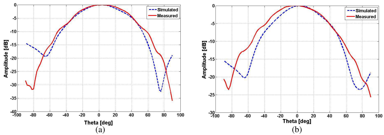
Figure 5. Comparison of the simulated and measured normalized radiation pattern of the Sierpinski carpet fractal antenna in (a) \phi = 0^\circ plane and (b) \phi = 90^\circ plane.
