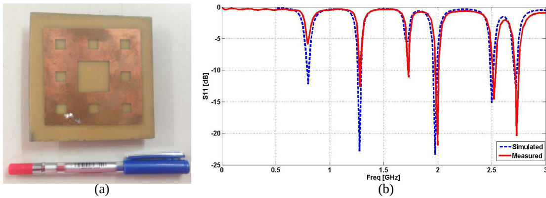
Figure 4. (a) Prototype of the square Sierpinski carpet fractal antenna. (b) Comparison of the simulated and measured return loss characteristics of the Sierpinski carpet fractal antenna designed using the proposed model.
