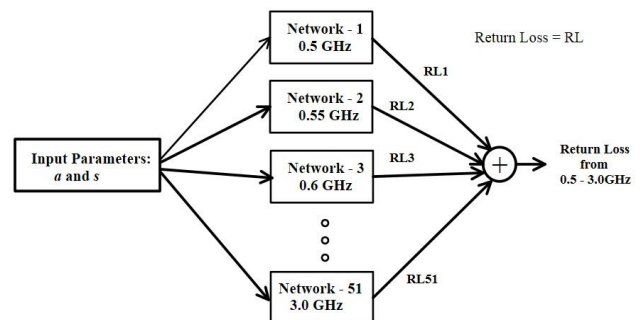
Figure 3. Proposed model for the diagnosis of the return loss characteristics.
