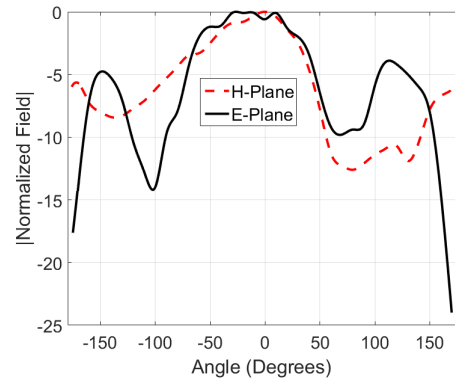
Figure 9. Measured normalized E -plane and H -plane far-field radiation patterns at 5.6 GHz.
