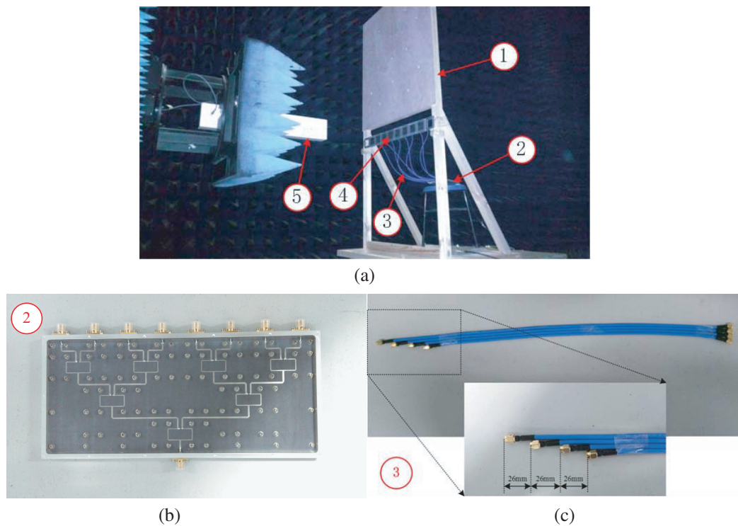
Figure 4. Photos of the experiment system: (a) overview; (b) power divider; (c) coaxial cables with four different phase delays of '0°', '90°', '180°' and '270°'.
