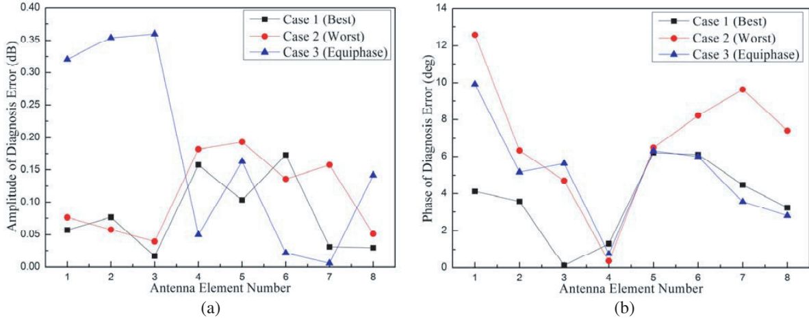
Figure 5. Array calibration errors under the three array excitation phases.
