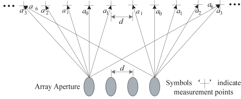
Figure 3. Illustration of the couplings between the measurement probe in the measurement points and the antenna elements.
