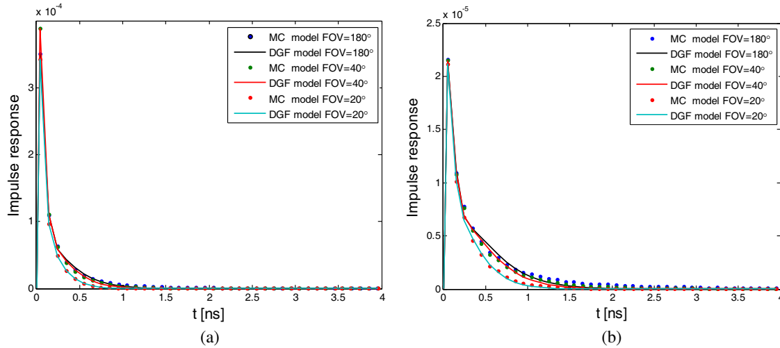
Figure 3. Impulse response in coastal water by Monte Carlo (MC) simulation and Double Gamma Functions (DGF) fitting. (a) L = 20 m, (b) L = 30 m.
