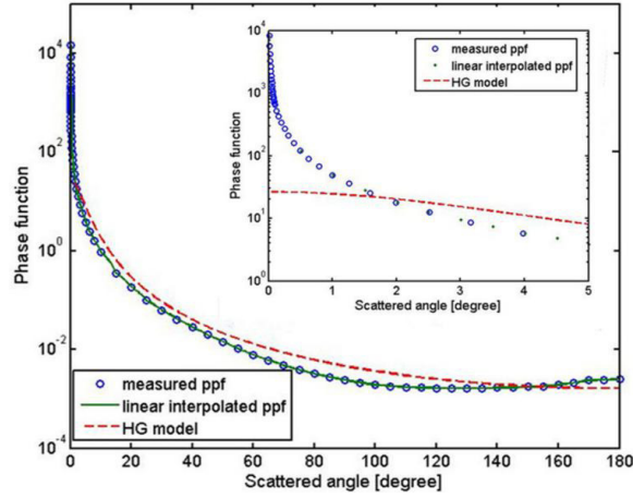
Figure 1. Particle phase function from [11] and HG phase function.
