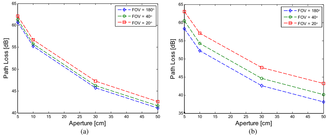
Figure 6. Curve of path loss for different apertures. (a) Coastal water ( L = 30 m). (b) Harbor water ( L = 9 m).
