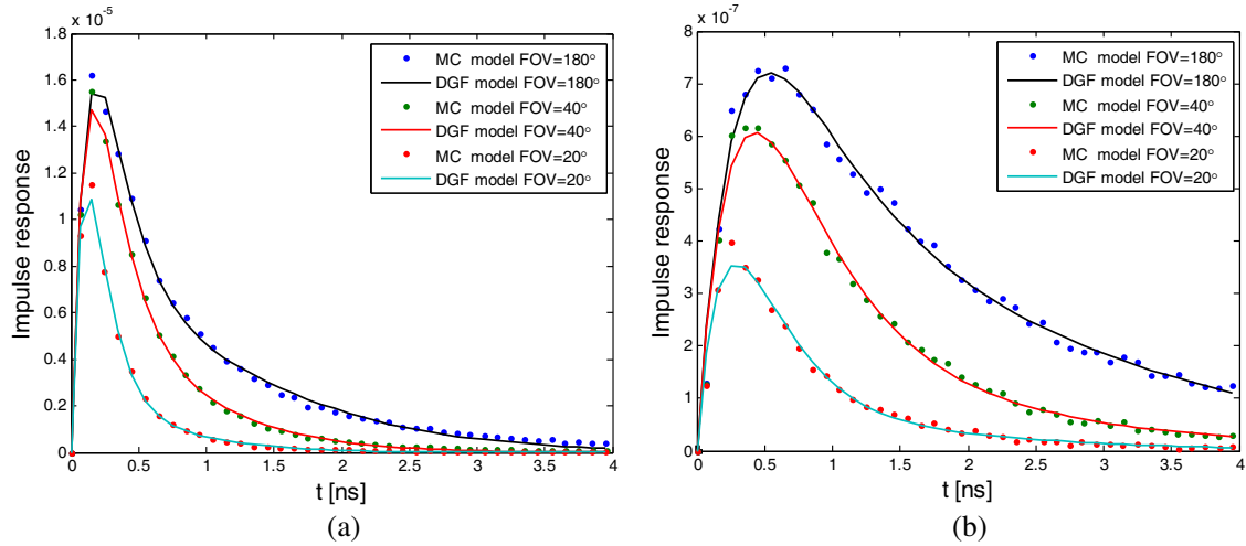
Figure 4. Impulse response in harbor water by Monte Carlo (MC) simulation and Double Gamma Functions (DGF) fitting. (a) L = 9 m, (b) L = 12 m.
