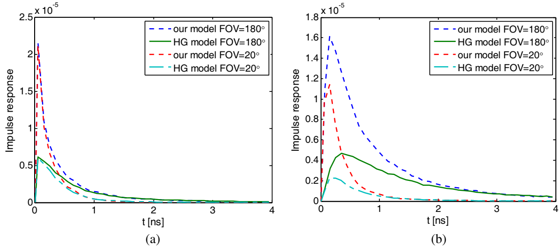
Figure 2. Impulse response by Monte Carlo (MC) simulation based on Petzold's measured phase function (our model) and HG phase function (HG model) respectively. (a) Coastal water ( L = 30 m). (b) Harbor water ( L = 9 m).
