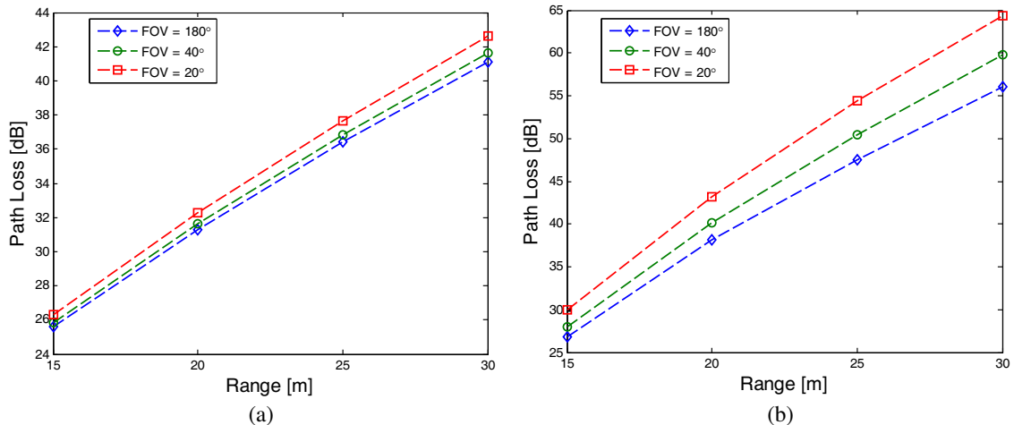
Figure 5. Curve of path loss for different link ranges. (a) Coastal water. (b) Harbor water.
