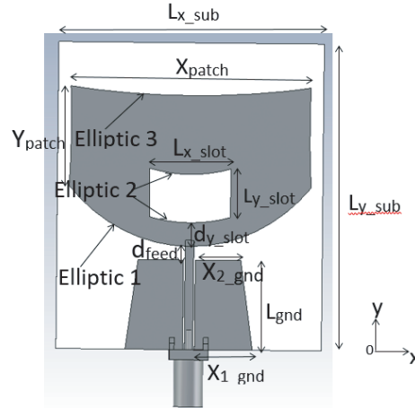
Figure 1. Omnidirectional UWB antenna schematic.
