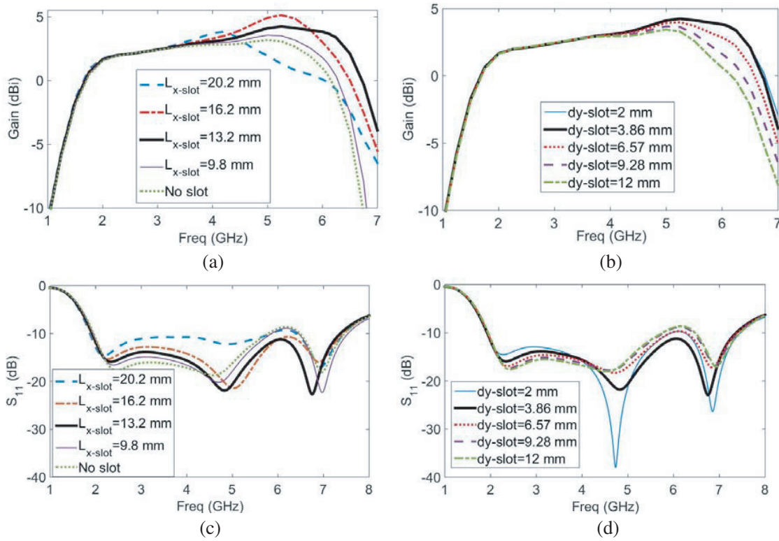
Figure 5. Effect of the length of the slot and distance between slot and feeding point on antenna gain and matching: (a), (b) effect of L_{x-slot} , and d_{y-slot} , on antenna gain, (c), (d) effect of L_{x-slot} , and d_{y-slot} , on antenna matching.
