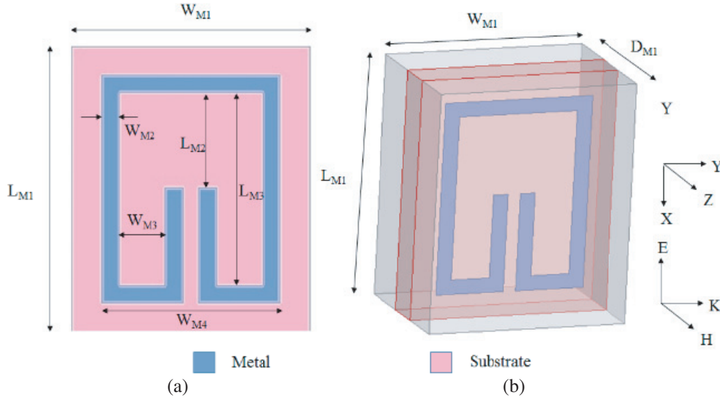
Figure 1. Simulation model of SRR unit cell. (a) Top view and (b) 3-D view.
