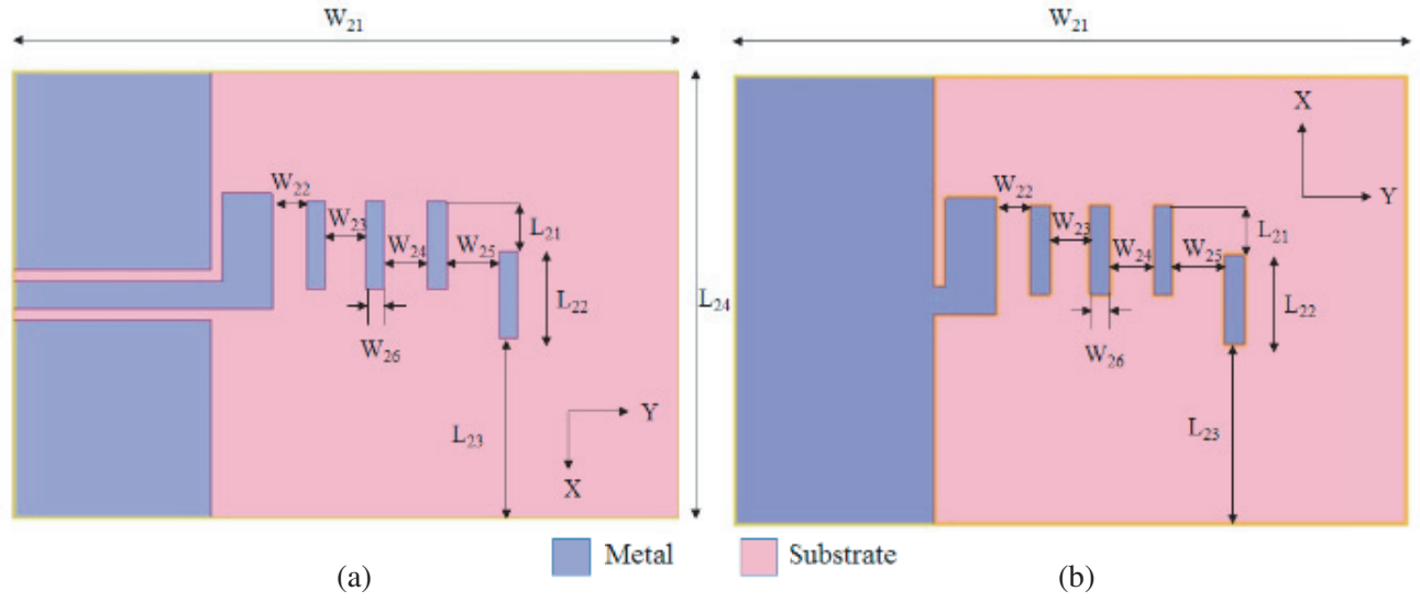
Figure 3. Design of microstrip Yagi array. (a) Top layer and (b) bottom layer.
