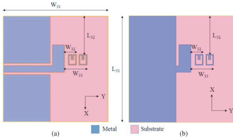
Figure 4. Design of SRR Loaded Yagi antenna. (a) Top layer and (b) bottom layer.
