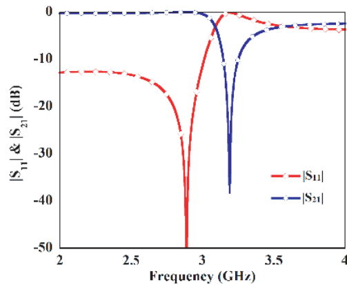
Figure 5. S parameters for SRR unit cell.
