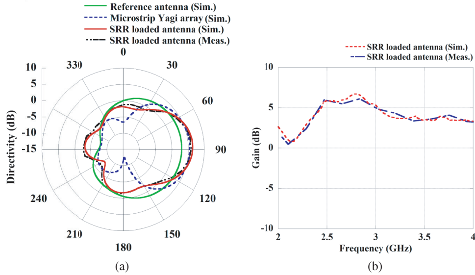
Figure 8. (a) Comparison of antenna's radiation characteristics. (b) Measured and simulated gain versus frequency plot of the SRR loaded Yagi antenna.
