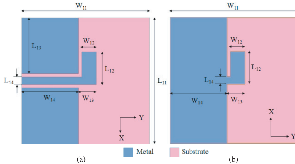
Figure 2. Design of reference antenna. (a) Top layer and (b) bottom layer.
