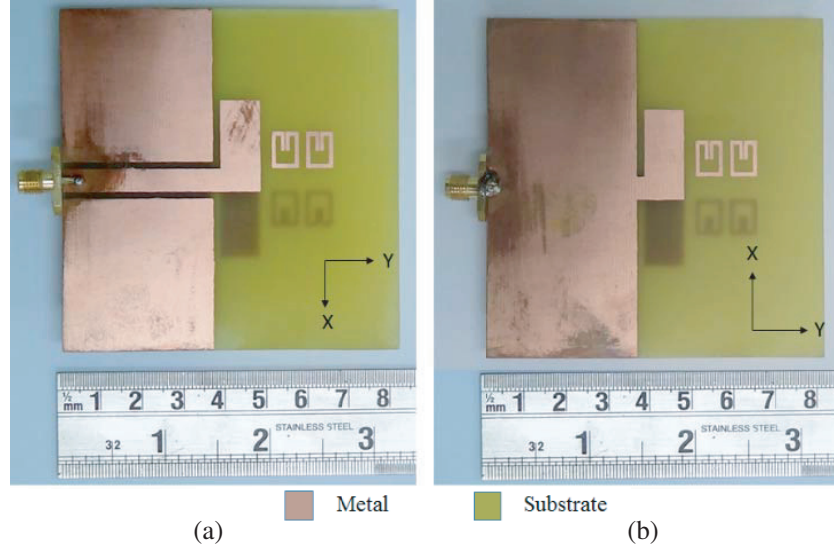
Figure 7. Fabricated prototype of SRR loaded Yagi antenna. (a) Top layer and (b) bottom layer.
