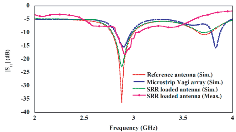
Figure 6. Return loss characteristics for designed antennas.
