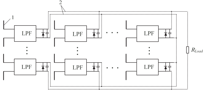
Figure 1. The rectenna array schematics: 1 — radiator; 2 — wires of the power collection circuit; LPF — low-pass filter.
