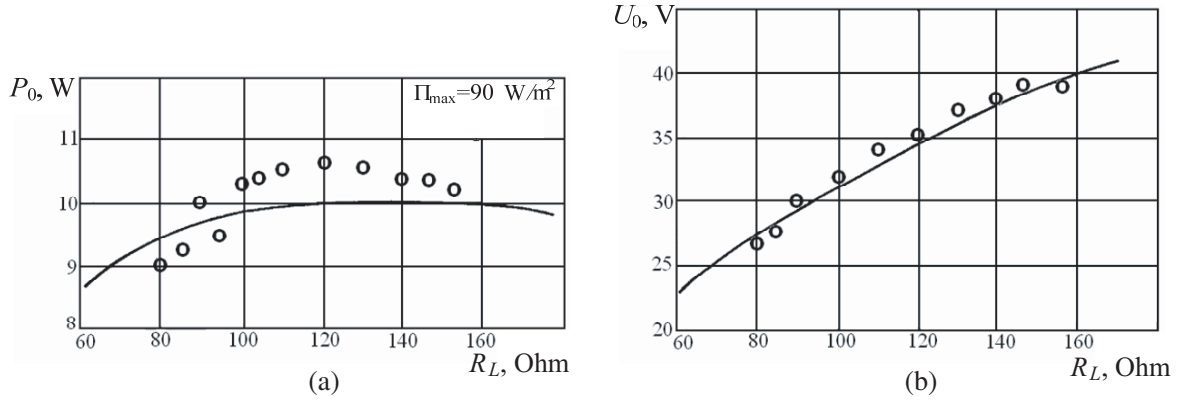
Figure 9. The DC power and voltage versus the load resistance for the experimental rectenna: (a) power; (b) voltage; \Pi_{\max} is power flux density at the rectenna. The energy transmission was performed at the distance of 3 m.
