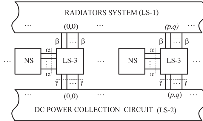
Figure 3. The block-diagram of the rectenna array.
