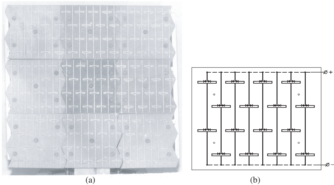
Figure 8. The experimental rectenna: (a) design; (b) the schematic diagram of the base module.
