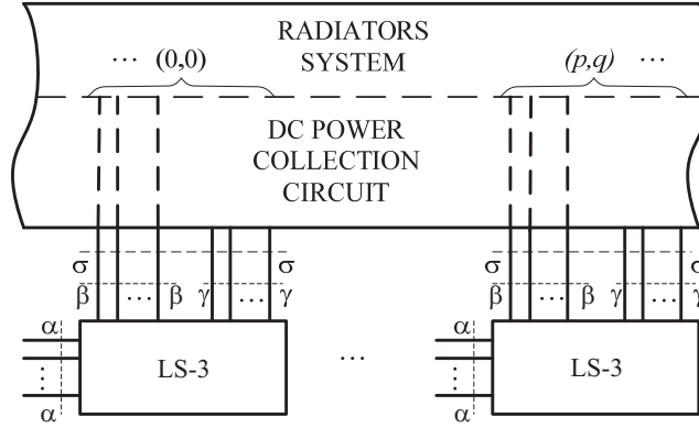
Figure 5. The modified linear subcircuit of the rectenna.
