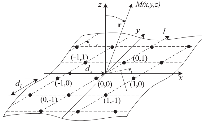
Figure 2. The periodic structure of the rectenna array.
