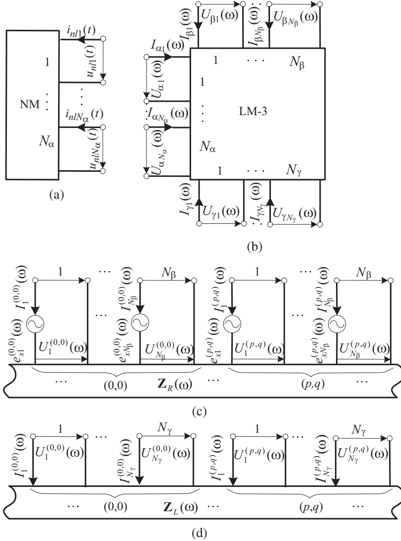
Figure 4. The rectenna subcircuits as multipole at the step of determining the state variables.
