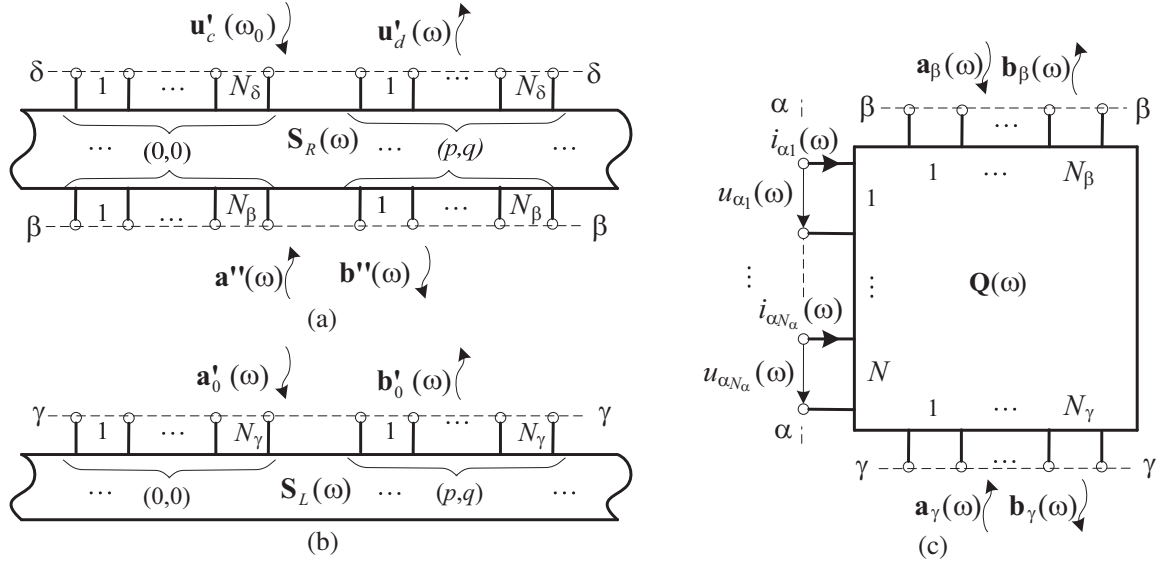
Figure 7. The representation of the linear rectenna subcircuits at the stage of the external parameter definition.
