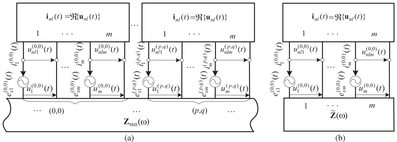
Figure 6. Schematics of the infinite periodic array of the RRE.
