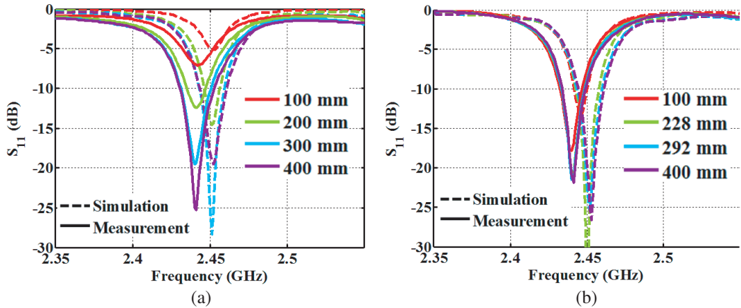
Figure 4. S_{11} magnitude comparison. (a) Metallic flaps [6]. (b) Plasma wall.
