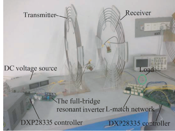
Figure 9. The experimental setup of the system.
