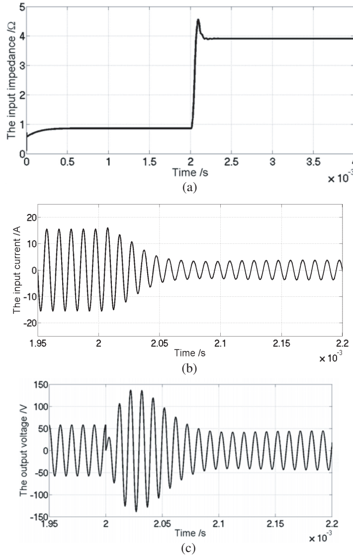
Figure 7. The simulation results with D = 30 cm. (a) The input impedance versus time. (b) The input current versus time. (c) The output versus time.
