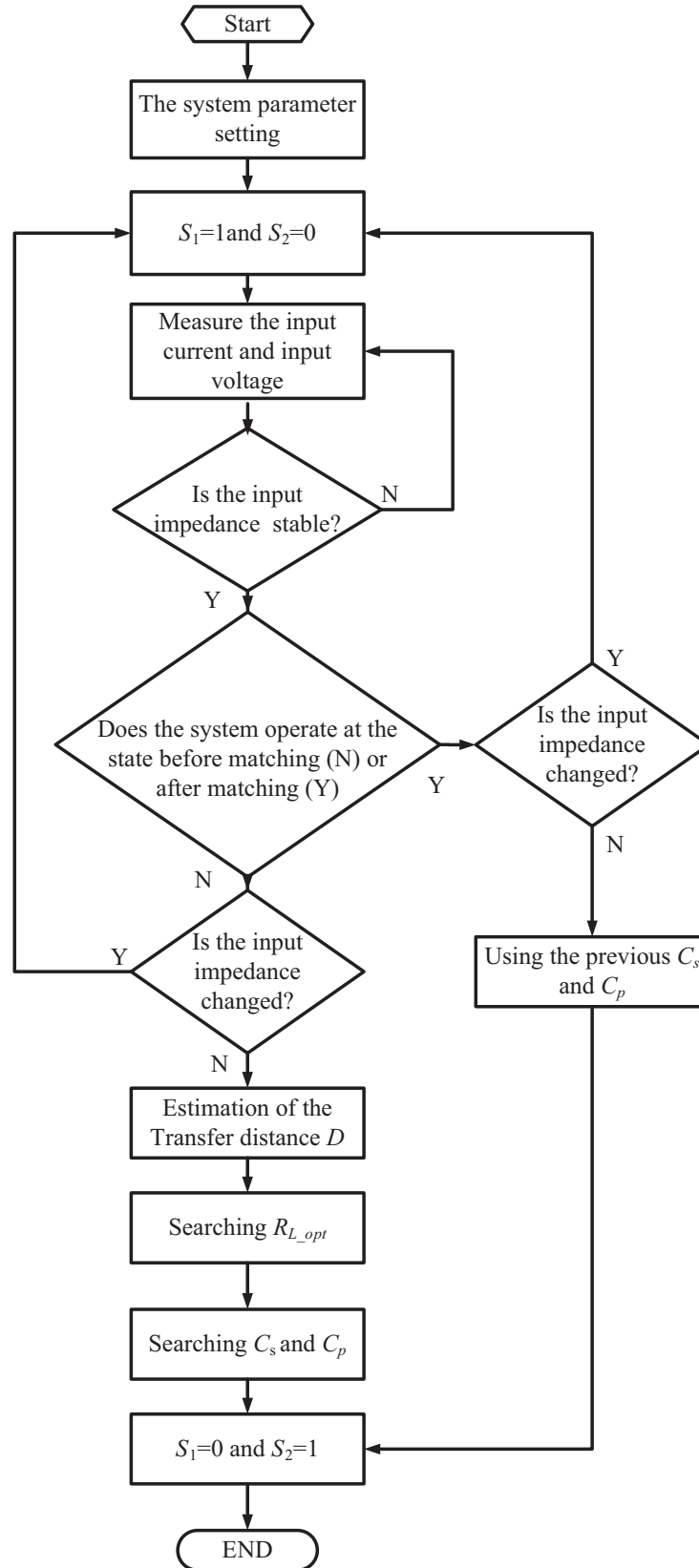
Figure 6. The flowchart of the FTOE method.
