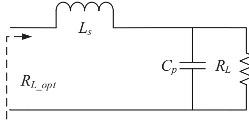
Figure 4. The circuits of the L-match network.
