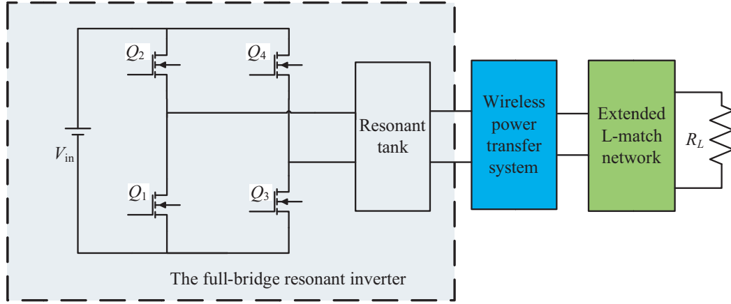
Figure 10. The schematic of the resonant inverter.
