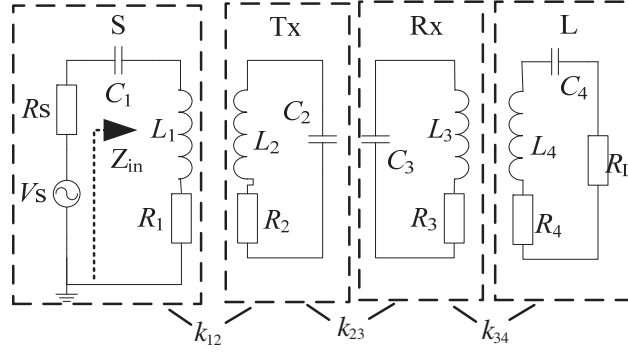
Figure 2. The equivalent circuit model for the WPT system. Each coil is modeled as series resonators.
