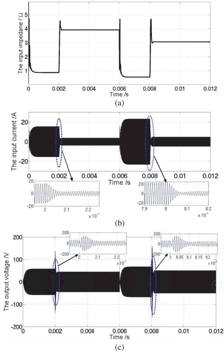
Figure 8. The simulation results with D changed from 30 cm to 25 cm. (a) The input impedance versus time. (b) The input current versus time. (c) The output versus time.
