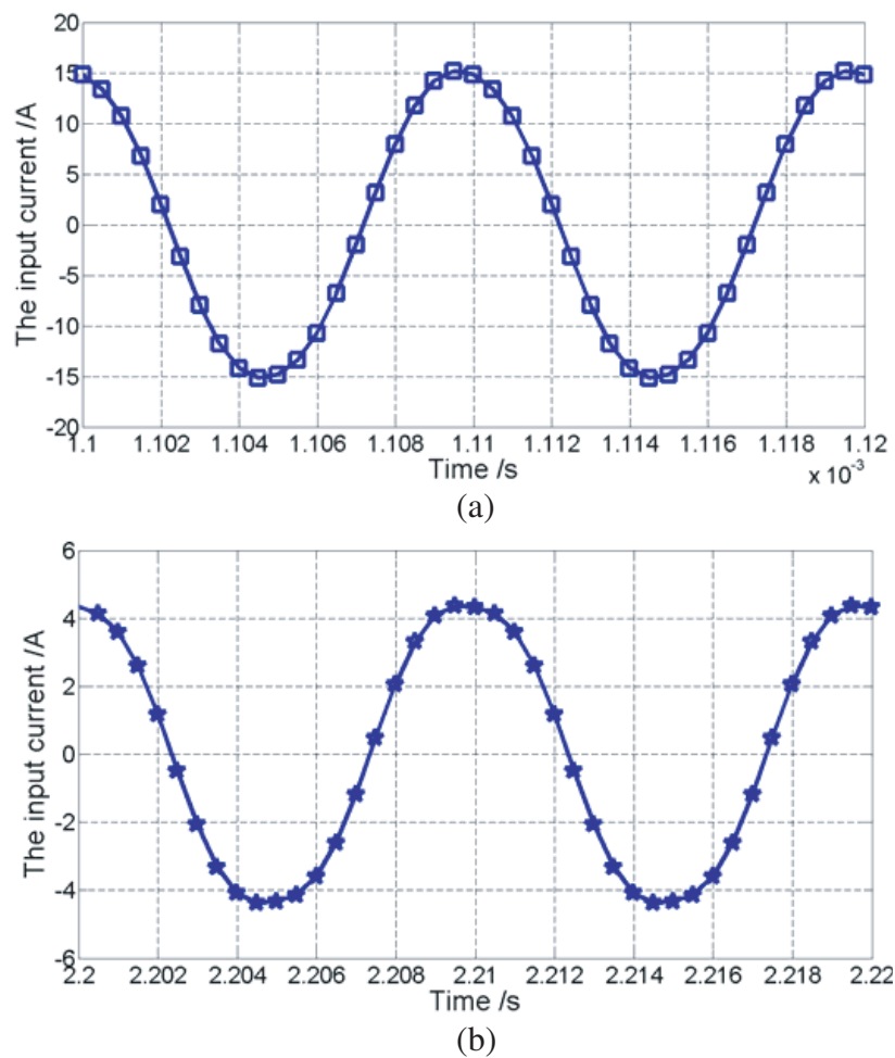
Figure 12. The input current versus time with D = 30 cm. (a) The input current before matching. (b) The input current after matching.
