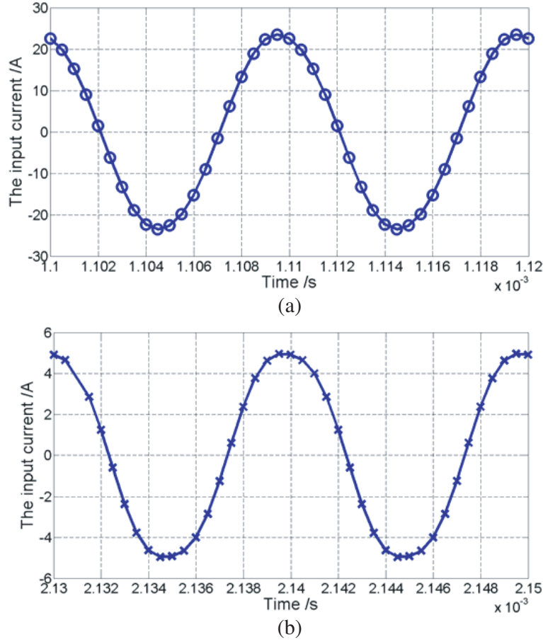
Figure 13. The input current versus time with D = 25 cm. (a) The input current before matching. (b) The input current after matching.
