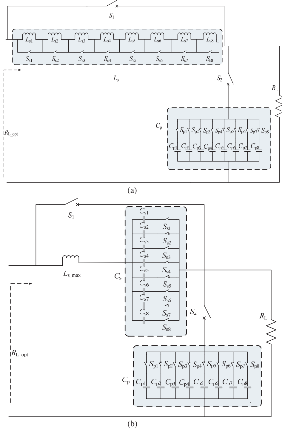
Figure 5. The extended L-match network. (a) The extended L-match network with using inductance matrix. (b) The extended L-match network with using capacitor matrix.
