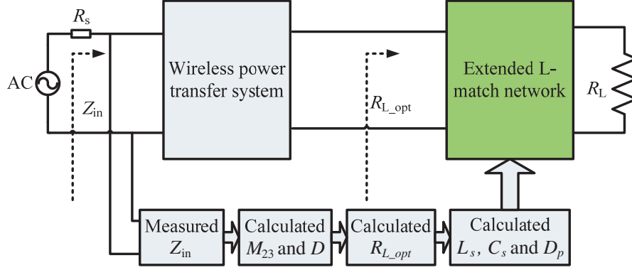
Figure 3. The circuit structure of the FTOE method.
