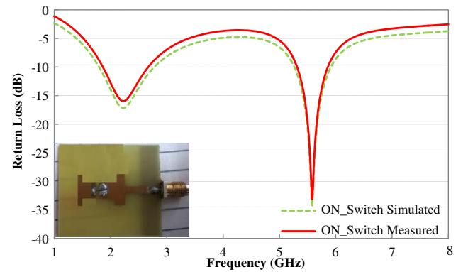
Figure 7. Simulated and measured results of antenna in ON switch.
