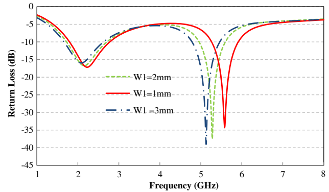
Figure 3. S_{11} against varied W1 .
