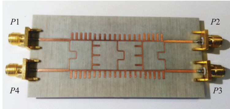
Figure 3. Resulting fabricated device.
