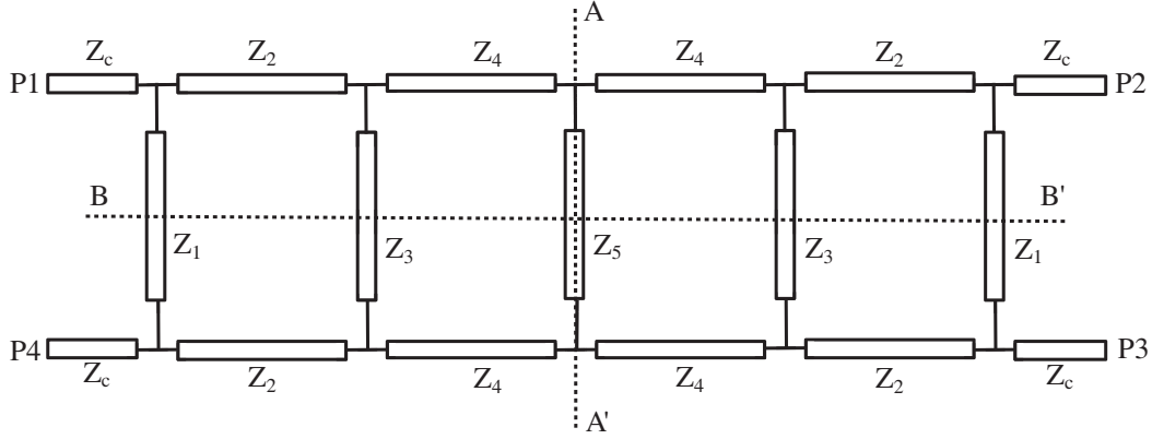
Figure 1. Crossover basic topology based on the cascade of 4-section branch line couplers.
