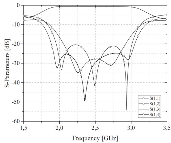
Figure 4. Measured S -parameters of the proposed device.
