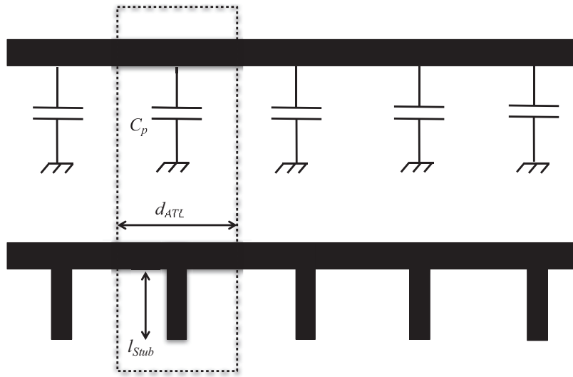
Figure 2. Stub-loaded Artificial Transmission Line (ATL).
