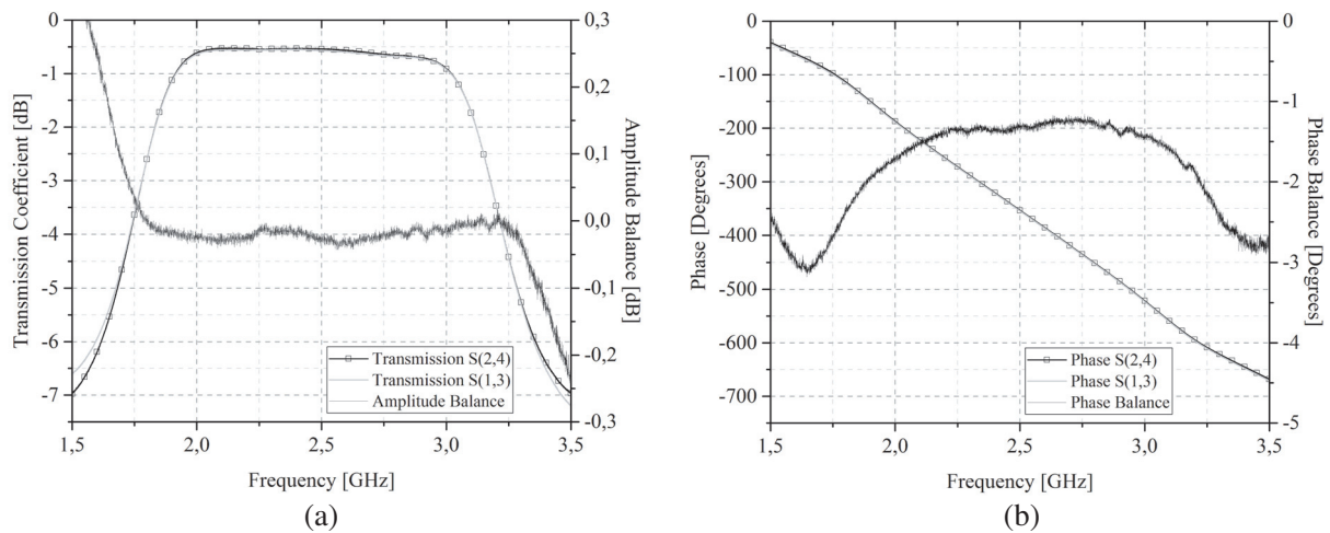
Figure 5. (a) Measured magnitude balance and (b) phase balance between RF ports 1-3 and 2-4.
