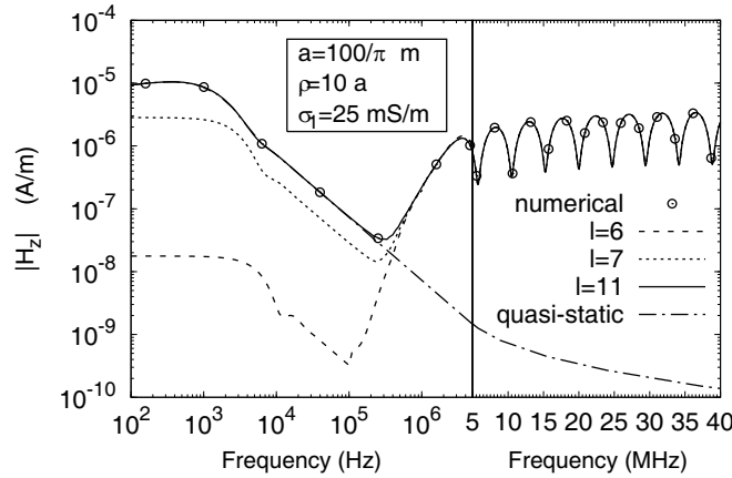
Figure 4: Amplitude-frequency spectrum of H_z , computed at distance \rho = 1000/\pi m from the loop axis.
