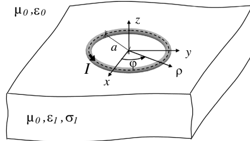
Figure 1: Thin-wire circular loop antenna on the surface of a single-layer conducting medium.
