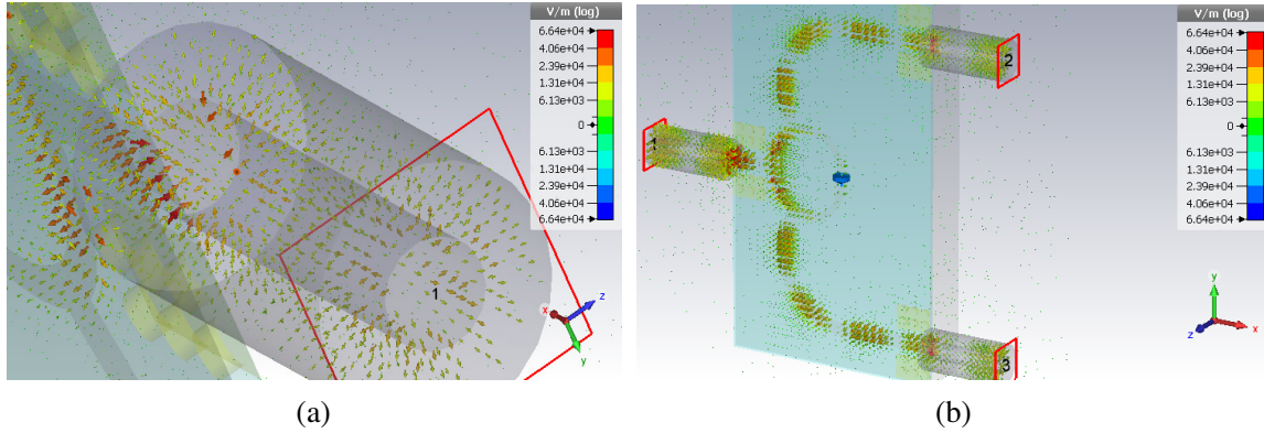
Figure 12. The electrical fields of the final proposed Wilkinson power divider with CB-CPW pre transition, Coaxial Off center from microstrip line and the edge cut of the center rod of the 2.4 mm connector. (a) The electrical field distribution in coaxial to microstrip line, and (b) electrical field distribution in the whole final Wilkinson power divider structure.
