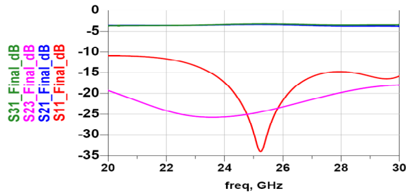
Figure 13. The final simulation results of magnitudes of S parameters of new Wilkinson power divider with transition.
