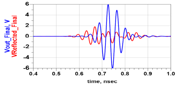
Figure 14. The time domain input reflection and output results of the final design (with CB-CPW pre transition, Coaxial Off center from Microstrip line and the edge cut of the center rod of the coaxial connector) Wilkinson power divider.
