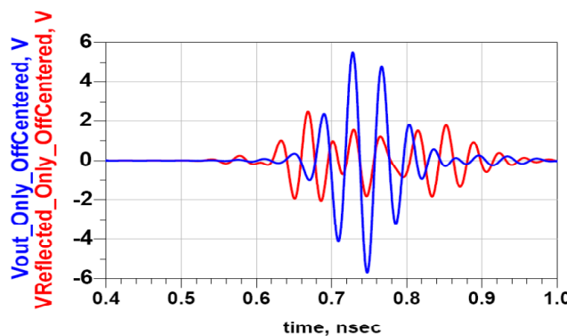
Figure 9. The time domain input reflection and output results of the second design (without pre-transition and only with off-centered coaxial connector) Wilkinson power divider.
