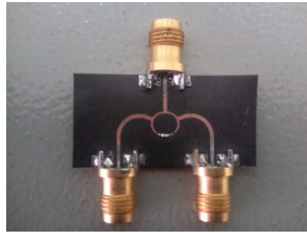
Figure 15. A photo of the final proposed modified Wilkinson power divider.
