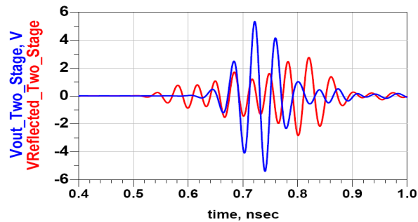
Figure 4. The time domain input reflection and output results of the first design (two stages) of Wilkinson power divider.
