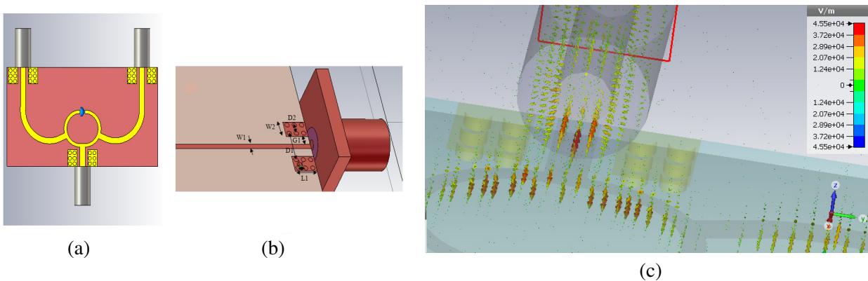
Figure 7. (a) The CST model of second proposed modified Wilkinson power divider, (b) the proposed transition dimensions, (c) the electrical fields of the second proposed Wilkinson power divider with CB-CPW pre transition section.
