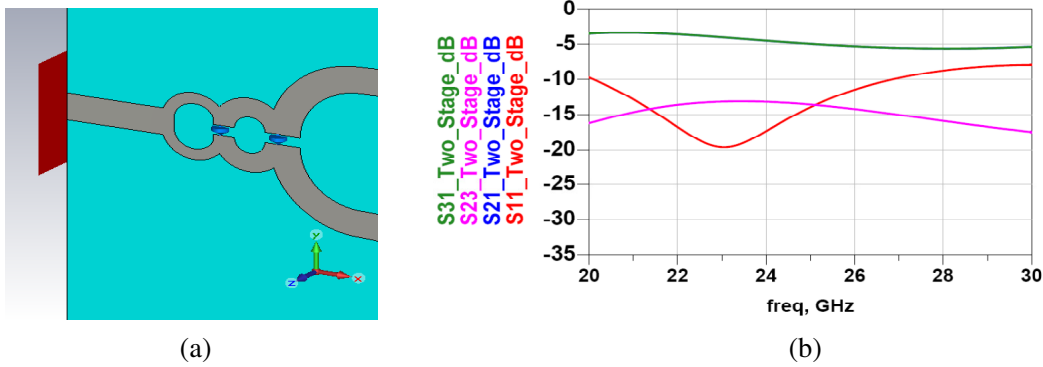
Figure 2. (a) The layout of the two sections Wilkinson power divider in CST, and (b) the simulation results of S -parameters of the two section power divider.
