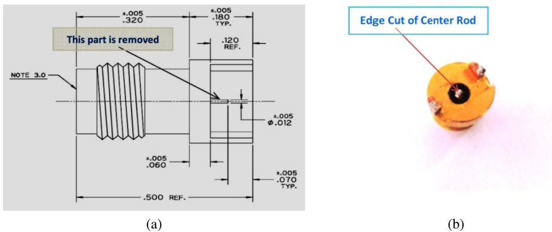
Figure 10. (a) Dimensions of the “Precision Connector, Inc.” 2.4 mm JACK PCB MOUNT, and (b) the photo of the connector with removing outer part of center rod and edge cut of remind center rod.
