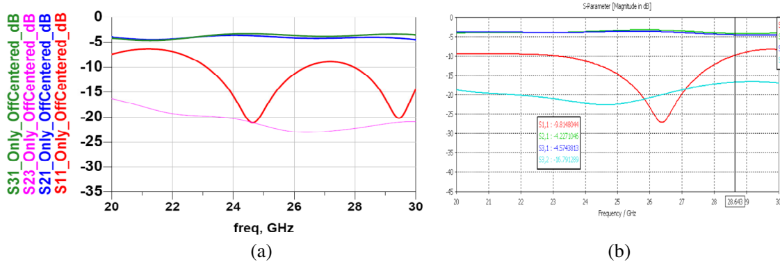
Figure 8. (a) The magnitudes of S -parameters of second Wilkinson power divider design without pre-transition and only with off-centred coaxial connectors and (b) the magnitude of S -parameters of the third design with Coaxial off-centred from microstrip line and CB-CPW pre transition.
