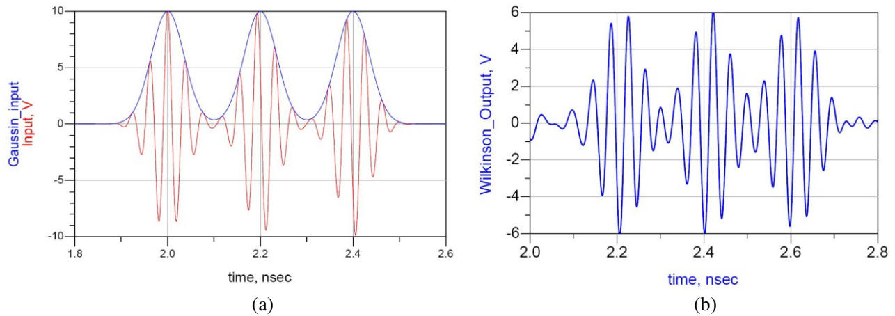
Figure 17. (a) 5 Gbps gaussian modulated input signal, and (b) 5 Gbps Gaussian modulated pulse output results of the measured final Wilkinson power divider.
