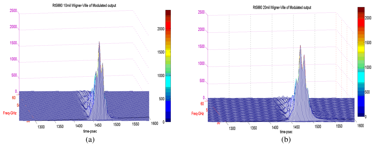
Figure 1. WVD of the propagated UWB modulated Gaussian pulses across the (a) 10 mil and (b) 20 mil laminates.
