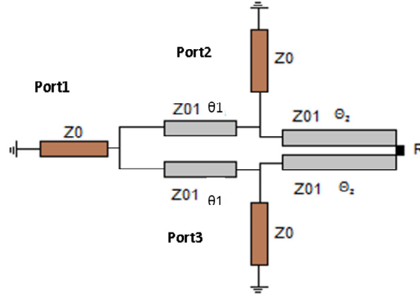
Figure 5. The schematic of the proposed modified Wilkinson power divider.
