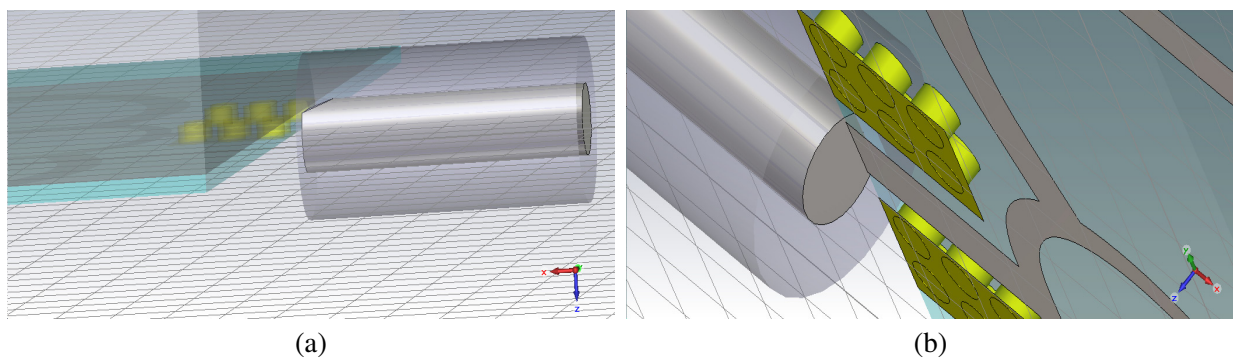
Figure 11. The structure view of the new proposed coaxial to microstrip transition. (a) The simulation graph of the edge cut of the center rod of the 2.4 mm connector in CST Software, (b) Coaxial Off center from microstrip line and CB-CPW to optimize the S -parameters results in CST software.
