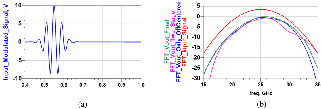
Figure 3. (a) The Gaussian modulated input signal, and (b) FFT of the input signal and output signals of different designed Wilkinson power dividers.
