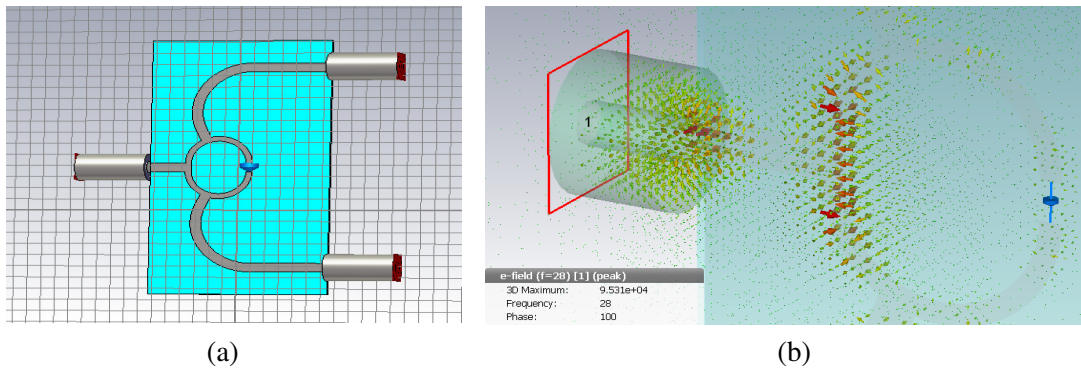
Figure 6. (a) The layout of the proposed Wilkinson power divider without CB-CPW pre transition section in CST, and (b) the electrical fields of the proposed Wilkinson divider without CB-CPW pre transition section.
