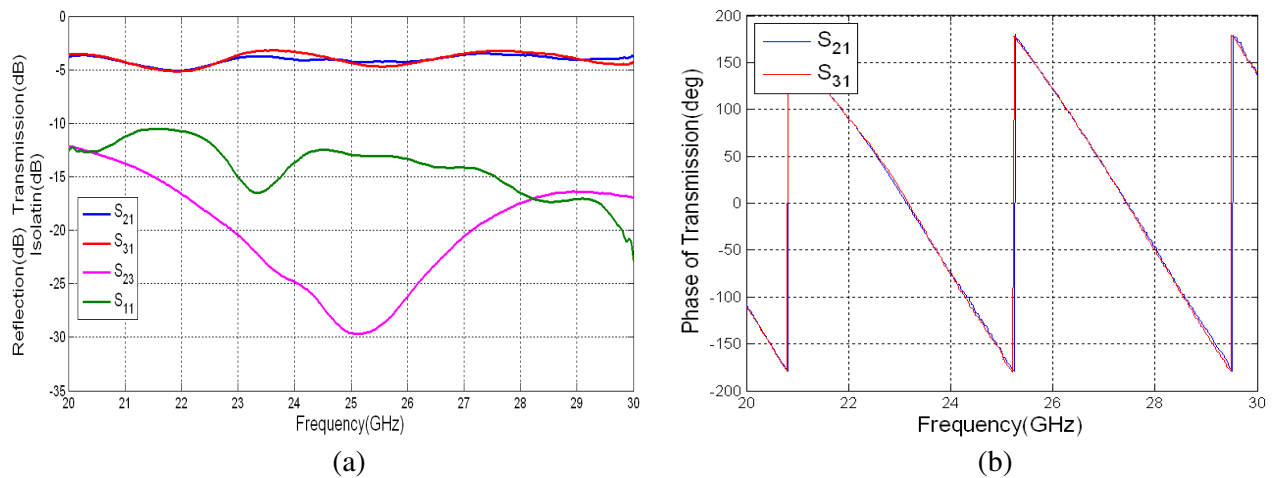
Figure 16. The measured S parameters results of the final proposed Wilkinson power divider; (a) Amplitude of the input reflection ( S_{11} ), transmissions ( S_{21} , S_{31} ), and isolation ( S_{23} ), and (b) phase of the transmission coefficients.
