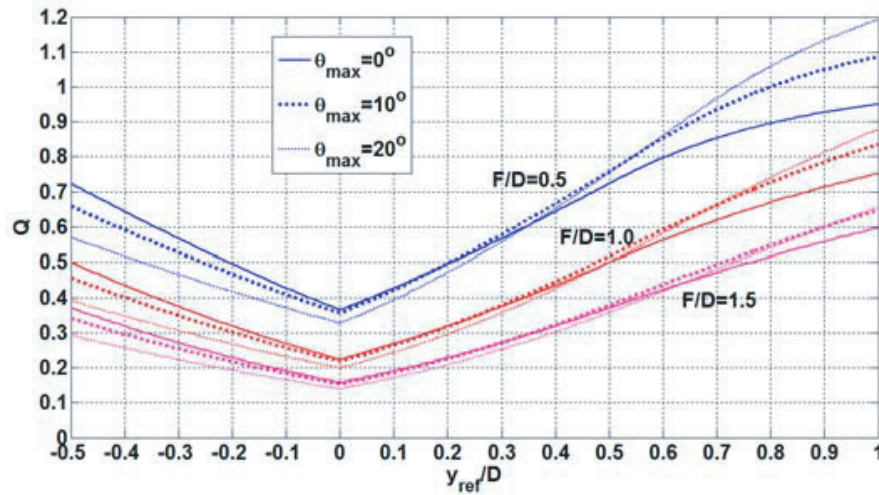
Figure 4. The function Q versus the normalized reference point y_{\text{ref}}/D .
