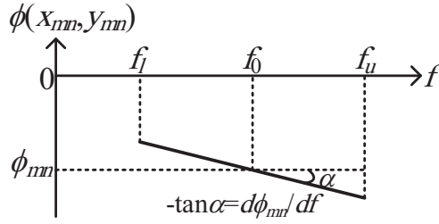
Figure 2. The phase-frequency response of cells of a wideband RAA.
