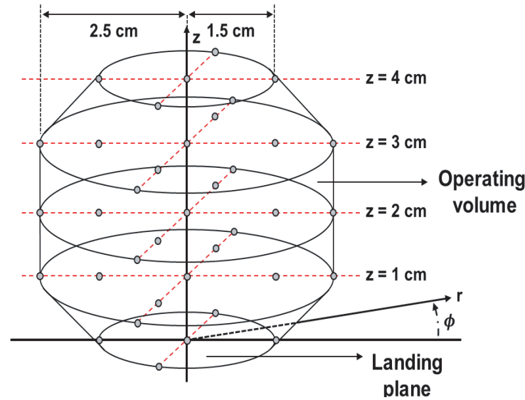
Figure 9. Operating volume for the EMV test.
