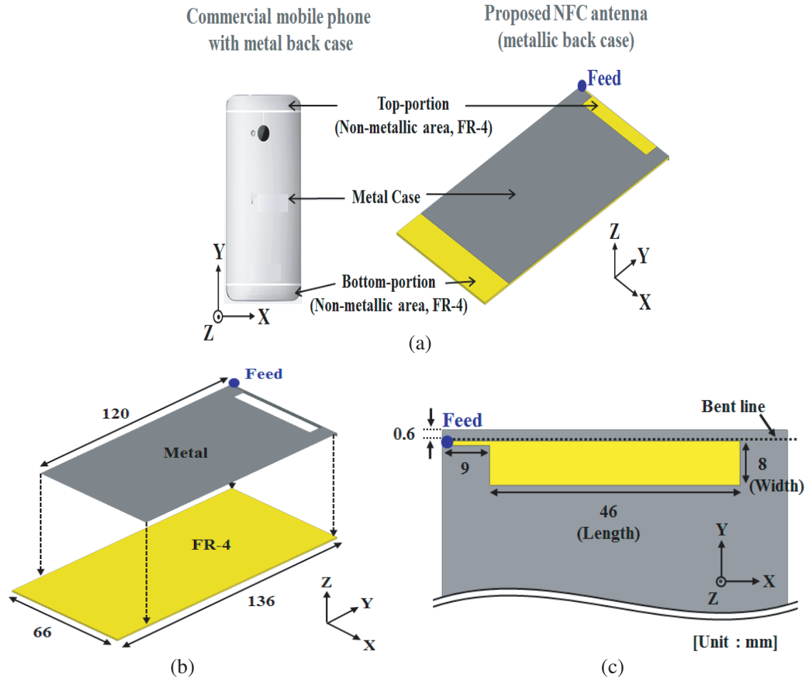
Figure 1. Geometry of the proposed NFC antenna: (a) Overall view, (b) dimension of the back case, and (c) dimension of the proposed single turn loop antenna on the top portion of the metal back case.
