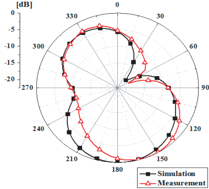
Figure 7. Normalized simulated and measured radiation patterns of the proposed secondary MIMO antenna at 880 MHz (XY-plane).
