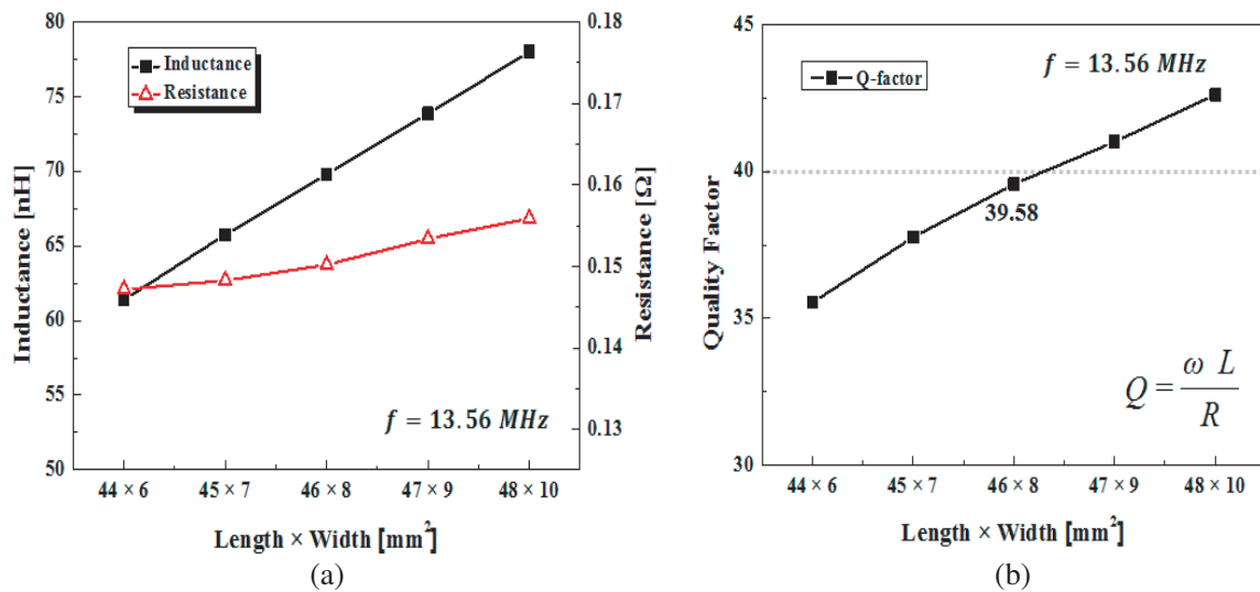
Figure 2. Simulated results of the proposed antenna with varying loop size at 13.56 MHz: (a) Inductance and resistance and (b) Q-factor.
