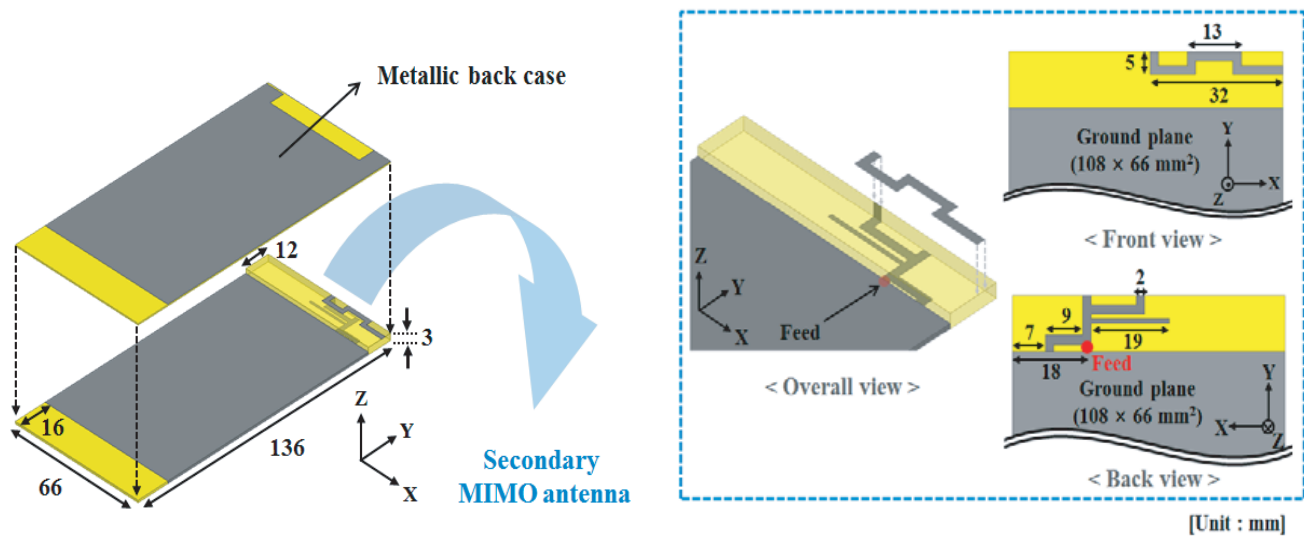
Figure 5. Geometry of the secondary MIMO antenna including the metal back case.
