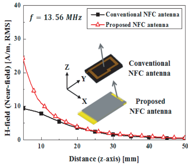
Figure 4. Simulated H -field (near-field) intensity with a normal direction ( z -axis) at the center of the proposed NFC antenna and the conventional 4-turn NFC loop antenna at 13.56 MHz.
