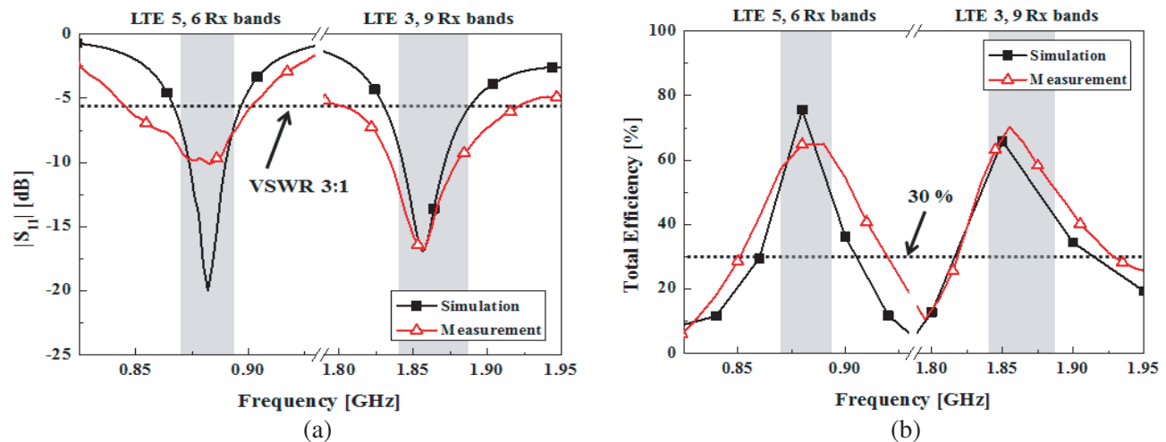
Figure 6. Simulated and measured results of the secondary MIMO antenna with the metal back case: (a) S_{11} and (b) total efficiency.
