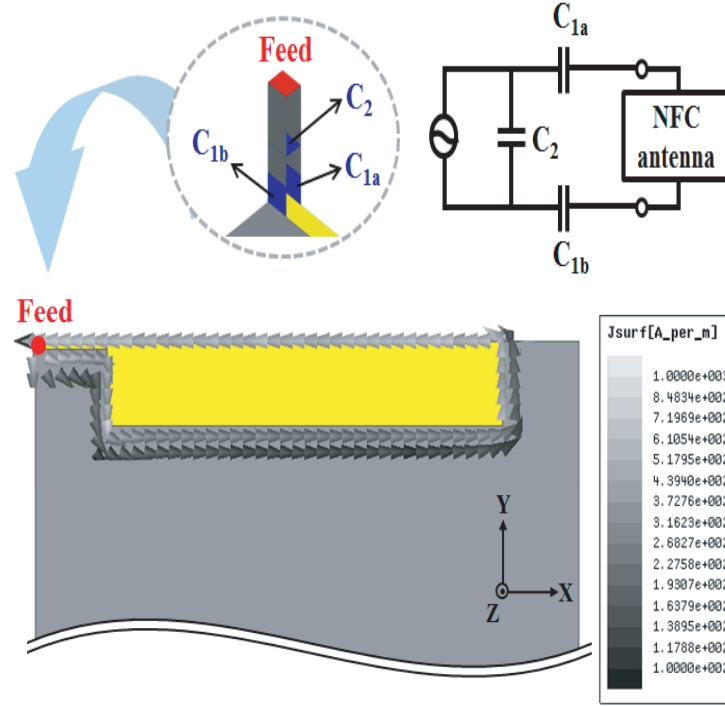
Figure 3. Matching circuit between the NFC chip and the NFC antenna, and current distribution of the proposed NFC antenna at 13.56 MHz.
