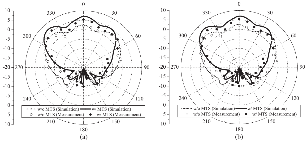
Figure 12. Simulated and measured far-field radiation patterns at high band. (a) E -plane. (b) H -plane.
