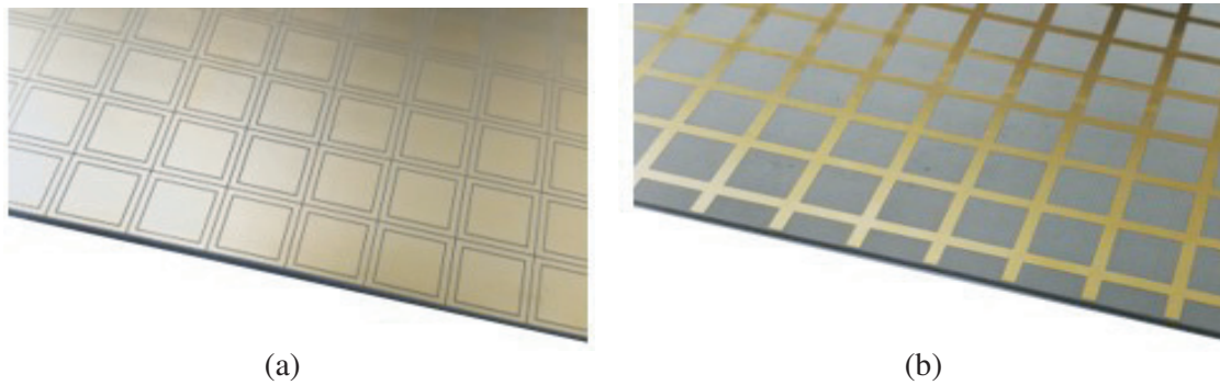
Figure 5. Photograph of the fabricated MTS (dimension = 144.5 mm \times 144.5 mm, number of unit cell = 17 \times 17). (a) One side. (b) The other side.
