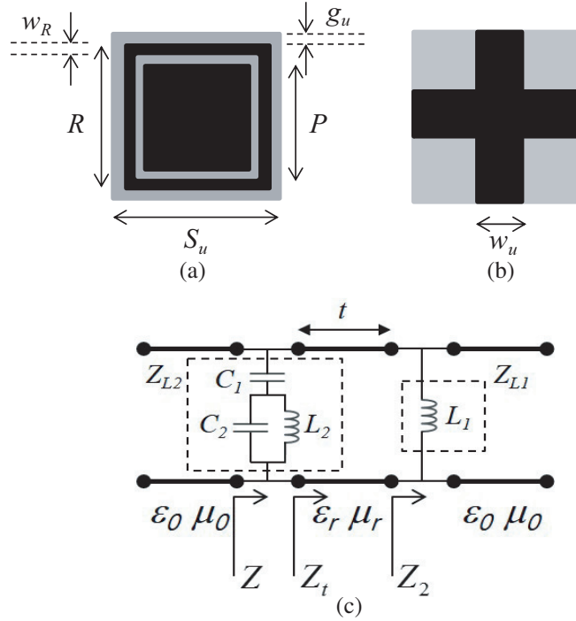
Figure 2. Unit cell of MTS. (a) One side. (b) The other side. (c) Its equivalent transmission line model.
