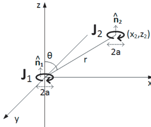
Figure 3. System comprising two identically sized and oriented magnetic dipoles.
