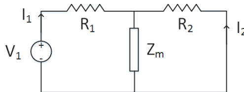
Figure 1. General two port network model describing the coupling between the dipoles.
