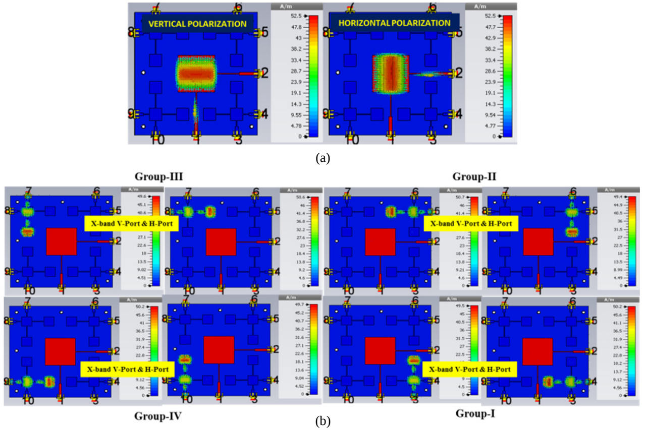
Figure 6. Surface current distribution of S/X-DBDP SAA for all ports. (a) S-band. (b) X-band.
