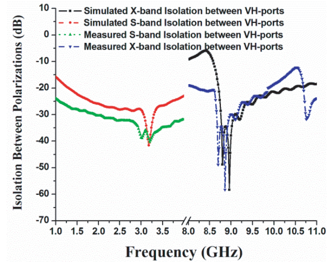
Figure 10. Simulated and measured isolation between bands of the S/X-DBDP SAA.
