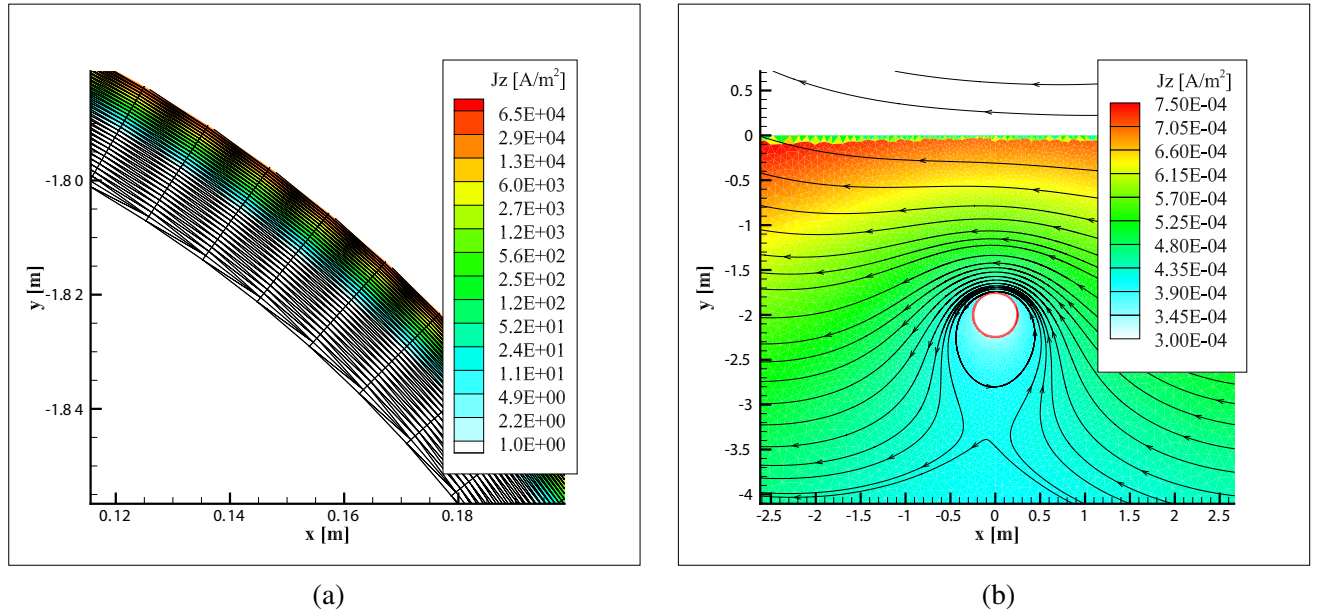
Figure 4. Distribution of |\mathbf{J}_z| through (a) the pipeline and (b) the the soil.
