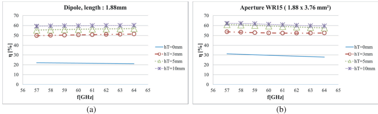
Figure 10. Radiation efficiency in [%] at different height above the body skin phantom: (a) dipole (length l = 1.88 mm); (b) aperture WR15: 1.88 \times 3.76 mm 2 .
