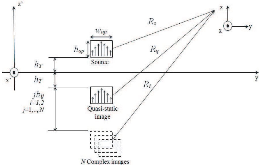
Figure 3. Complex image components for an aperture antenna.
