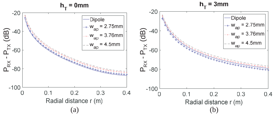
Figure 7. Path loss between antennas and observation point on body skin dielectric phantom ( h_R = 0 mm) for different transmitter height: (a) h_T = 0 mm, (b) h_T = 3 mm.
