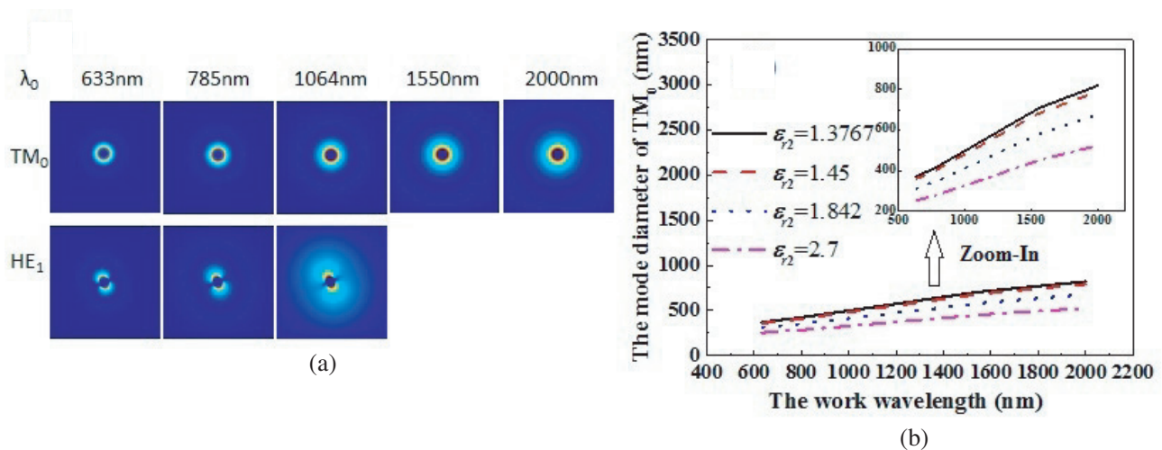
Figure 4. (a) |E| mode patterns for all supported modes by metal nanowires with a = 100 nm and \varepsilon_{r2} = 1.45^2 ; (b) Curves of mode field diameters with the work wavelengths and permittivity of cladding dielectric.
