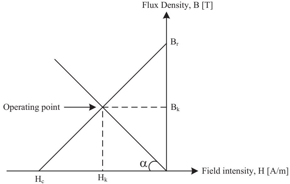
Figure 4. B-H curve and operating point of permanent magnet.
