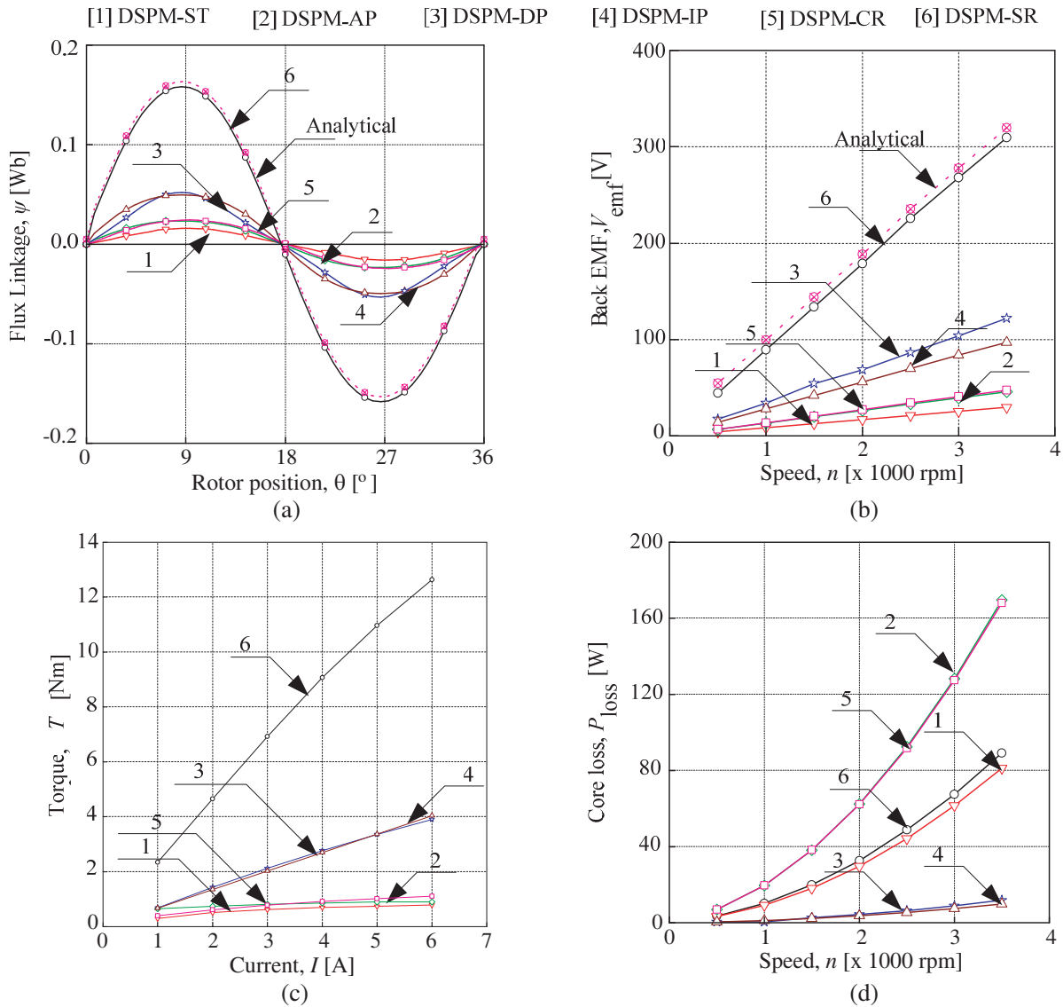
Figure 6. Comparison result for various model of DSPM motor. (a) Flux linkage. (b) Back emf. (c) Torque. (d) Core loss.
