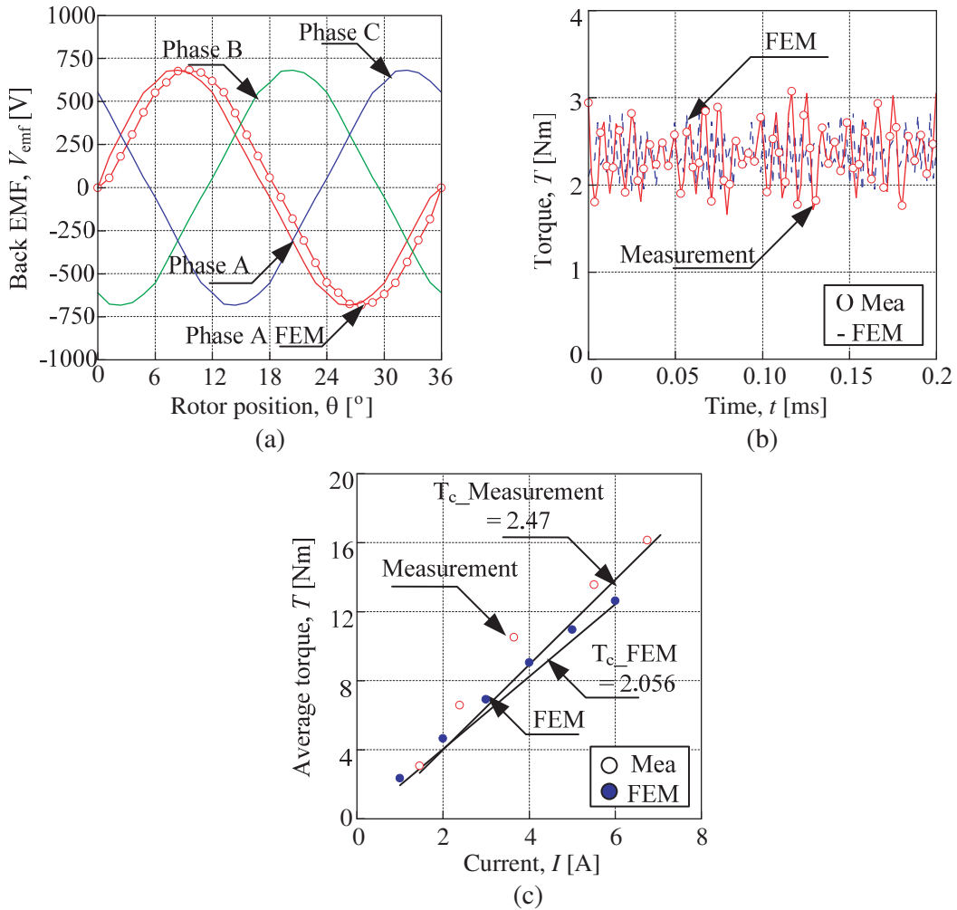
Figure 9. DSPM-SR verification result. (a) Back emf. (b) Torque. (c) Average torque.
