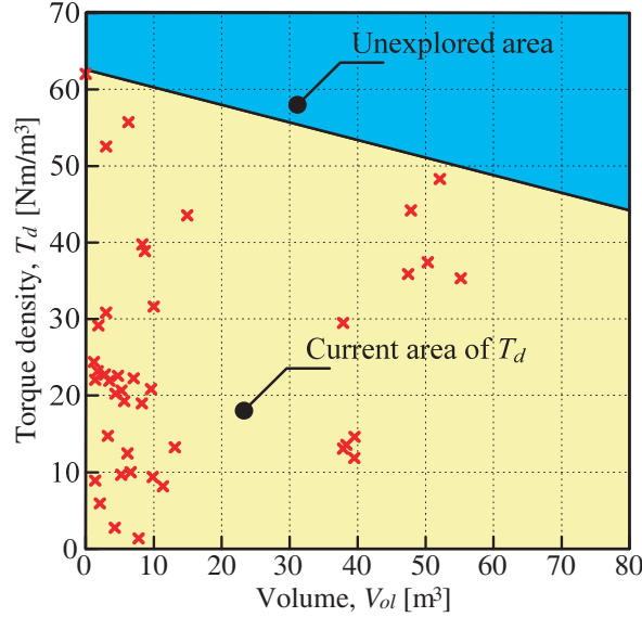
Figure 1. Current reported torque density.
