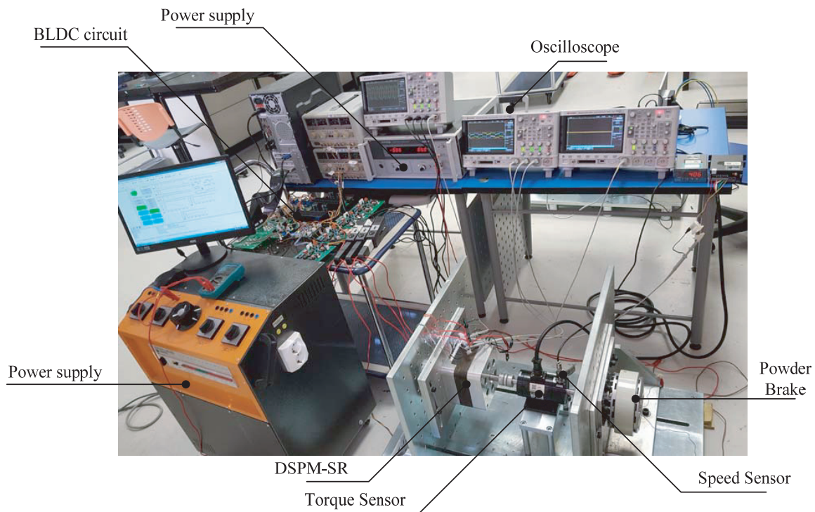
Figure 7. Fabricated DSPM-SR.
