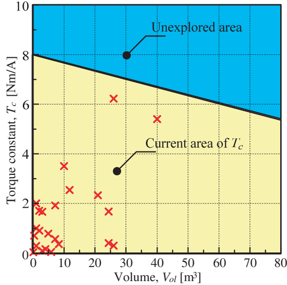
Figure 2. Current reported torque constant.
