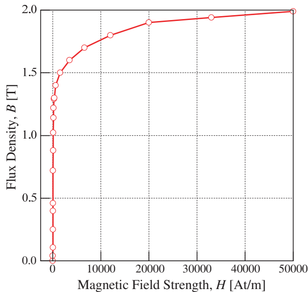
Figure 3. Non-oriented silicon steel M250-35A B-H curve.
