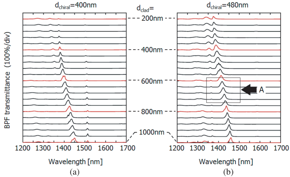
Figure 6. Calculated transmission spectra of BPFs using Si/Al 2 O 3 PCM. (a) Thin Si chiral layer ( d_{\text{chiral}} = 400 nm) case. Each plot correspond to different underclad thickness. (b) Thick ( d_{\text{chiral}} = 480 nm) Si chiral layers. Region A indicates the unimodal construction. Grating period was fixed as \Lambda = 960 nm.
