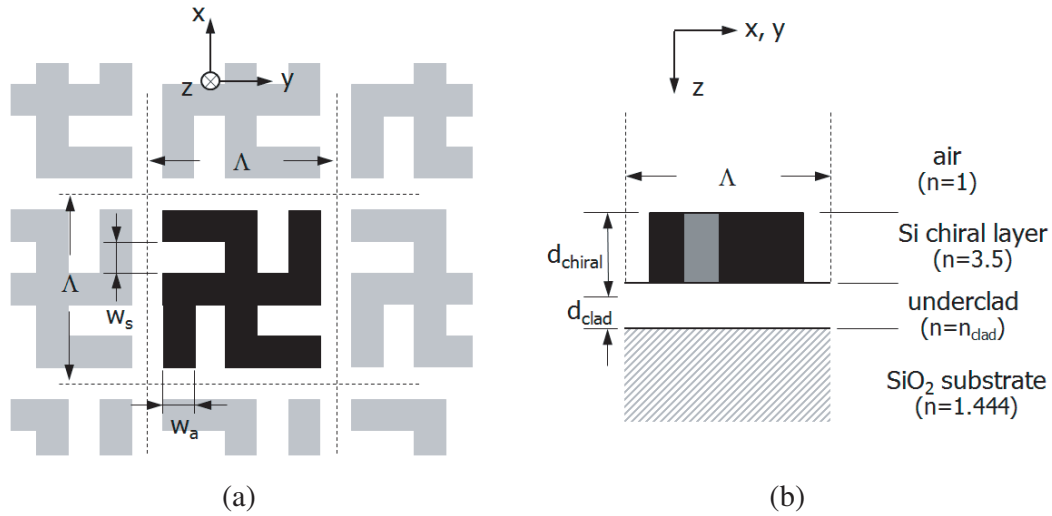
Figure 2. Schematic view of the PCM. (a) Top view, (b) cross sectional layer profile.
