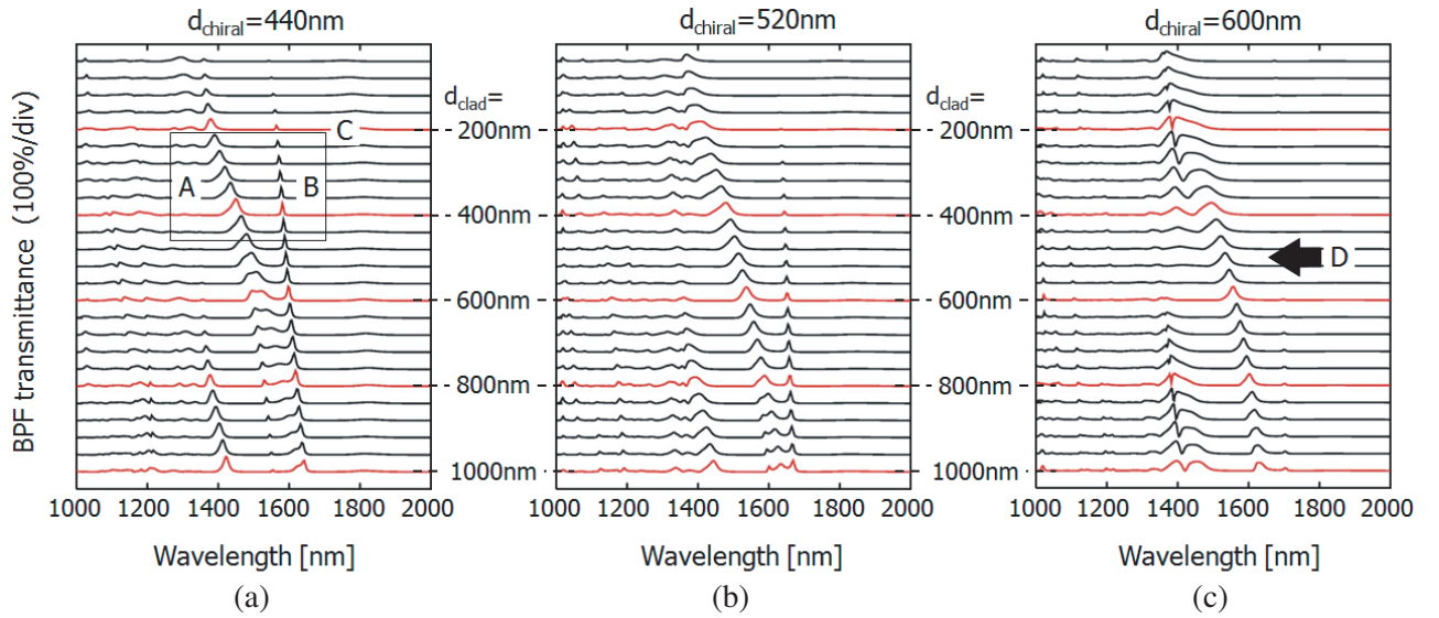
Figure 3. Calculated transmission spectra of the BPF using Si/Si 3 N 4 PCM. (a) Thin Si chiral layer ( d_{\text{chiral}} = 440 \text{ nm} ) case. Each plot correspond to different underclad thickness. Series A and B denote Fabry-Perot (FP) and guided-mode resonance (GMR) peaks, respectively. High transmittance peaks were obtained around the region C. (b) Intermediate ( d_{\text{chiral}} = 520 \text{ nm} ), and (c) thick ( d_{\text{chiral}} = 600 \text{ nm} ) Si chiral layers. Series D is the FP peak. Grating period was fixed as \Lambda = 960 \text{ nm} .
