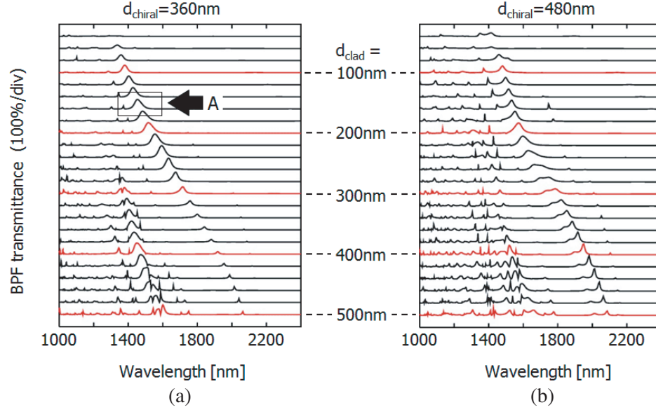
Figure 8. Calculated transmission spectra of BPFs using partial-etched type Si PCM. (a) Thin Si chiral layer ( d_{\text{chiral}} = 360 \text{ nm} ) case. Each plot correspond to different “unetched” Si thickness. Region A indicates high transmittance and almost unimodal construction. (b) Thick ( d_{\text{chiral}} = 480 \text{ nm} ) chiral layer. Grating period was fixed as \Lambda = 960 \text{ nm} .
