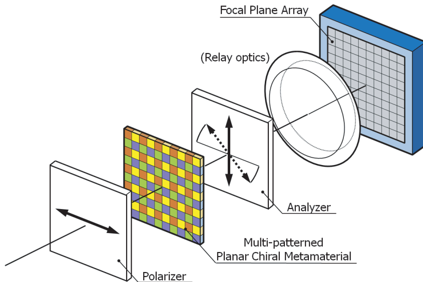
Figure 1. Schematic construction of a multispectral imaging system utilizing the polarization interference type band-pass filter array.
