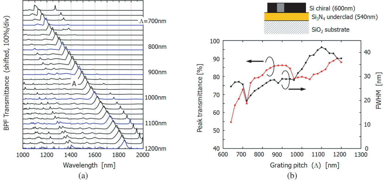
Figure 5. Designed single-peak filtering characteristics of Si/Si 3 N 4 PCM. (a) Spectra for various grating period ( \Lambda ). Thickness of Si chiral and Si 3 N 4 underclad layers were 600 nm and 540 nm, respectively. (b) Maximum transmittance and bandwidth of the main peak (indicated as ‘A’ in the left figure).
