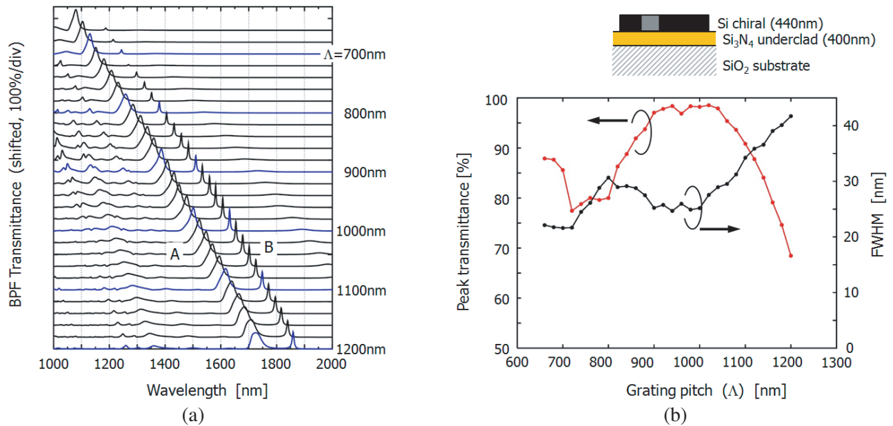
Figure 4. Designed double-peak filtering characteristics of Si/ \text{Si}_3\text{N}_4 PCM. (a) Spectra for various grating period ( \Lambda ). Thickness of Si chiral and \text{Si}_3\text{N}_4 underclad layers were 440 nm and 400 nm, respectively. (b) Transmittance and bandwidth of the main peak (indicated as 'A' in the left figure).
