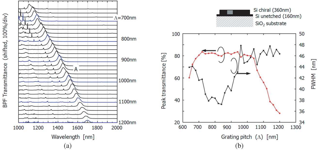
Figure 9. Designed filtering characteristics of the Si PCM. (a) Spectra for various grating period ( \Lambda ). Thickness of the etched and unetched parts of the Si layer were 360 nm and 160 nm, respectively. (b) Transmittance and bandwidth of the peak series A in the left figure.
